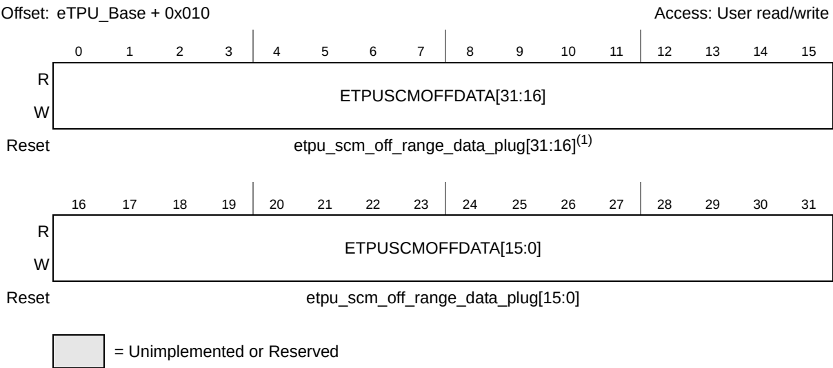
Figure 492. ETPU_SCMOFFDATAR Register
