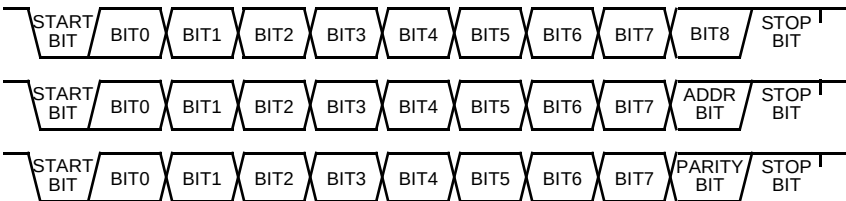
Figure 781. SCI Frame Formats (9 payload bits)
