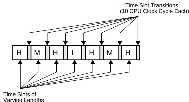
Figure 557. Time-slot sequence
