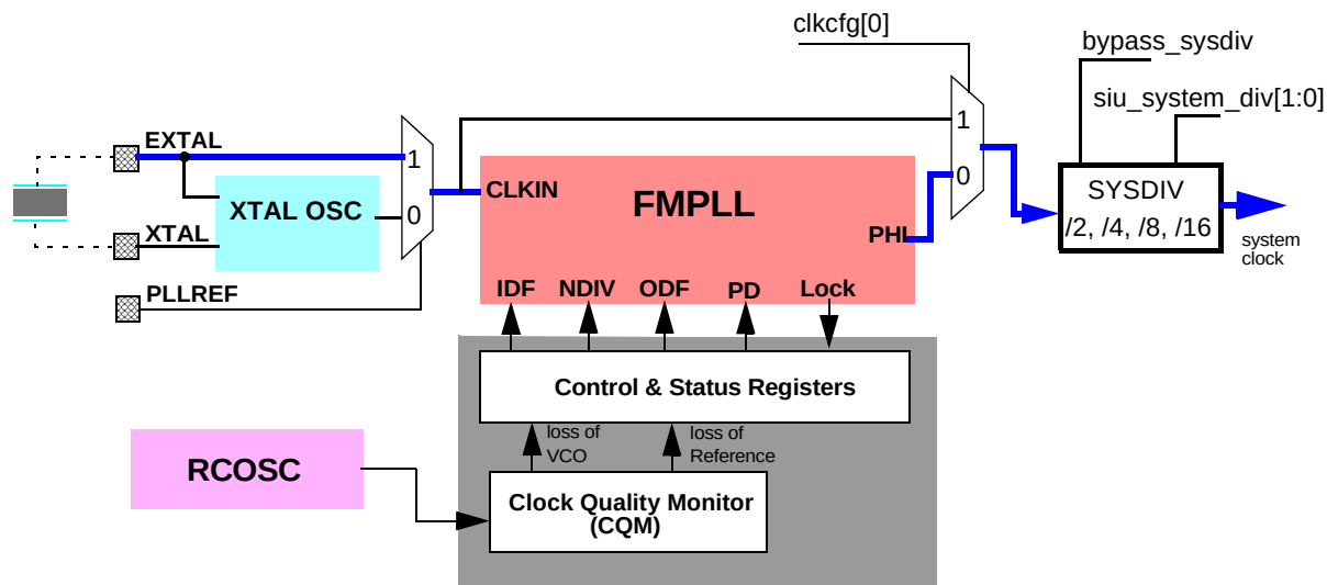
Figure 11. Normal Mode with External Reference
