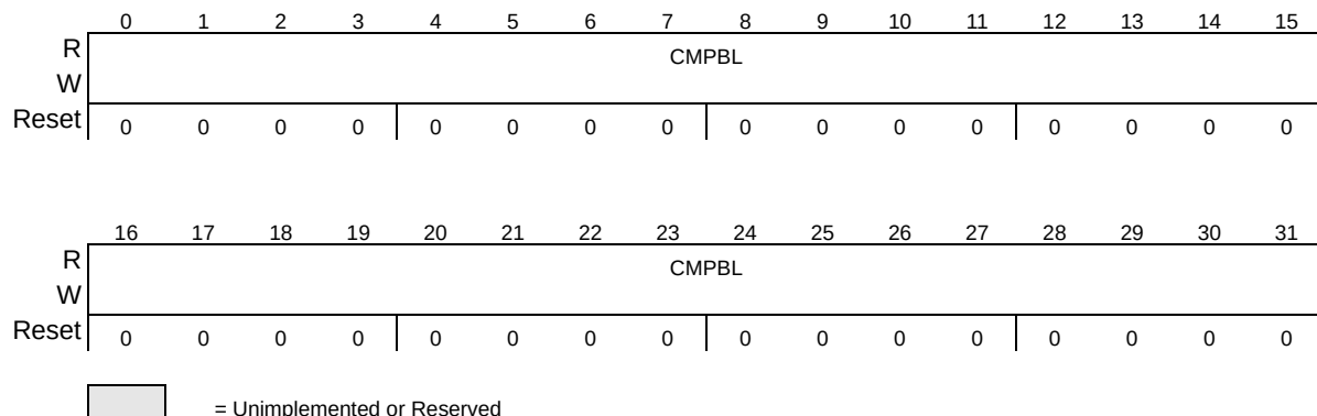
Figure 357. Compare B Low Register (SIU_CBRL)
