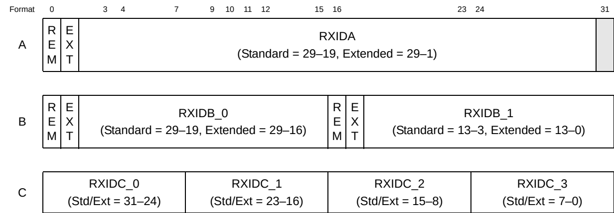
Figure 812. ID Table 0 – 7
