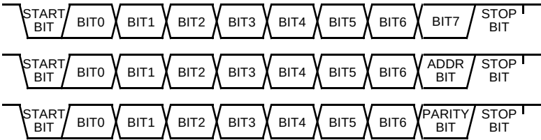
Figure 780. SCI Frame Formats (8 payload bits)
