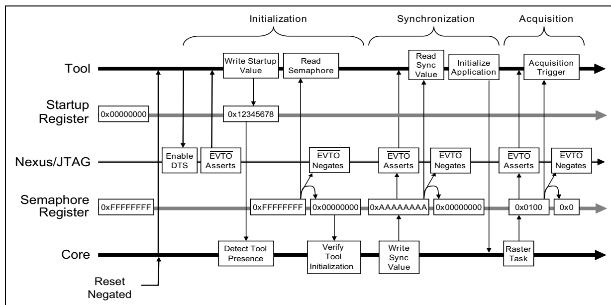
Figure 1032.DTS startup sequence example
