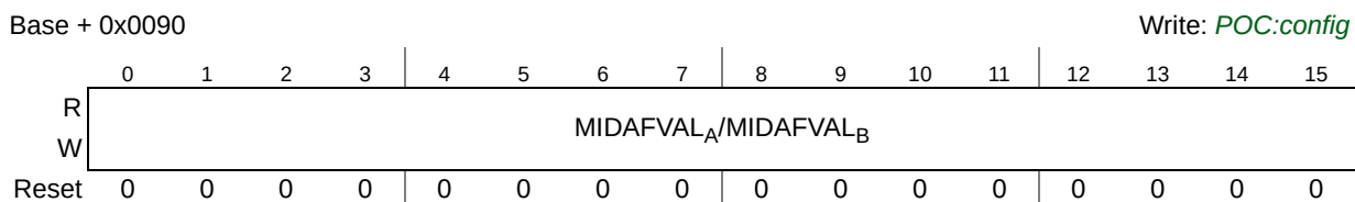
Figure 888. Receive FIFO Message ID Acceptance Filter Value Register (FR_RFMIDAFVR)
