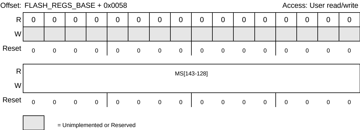
Figure 74. User Multiple Input Signature Register 4 (UMISR4)
