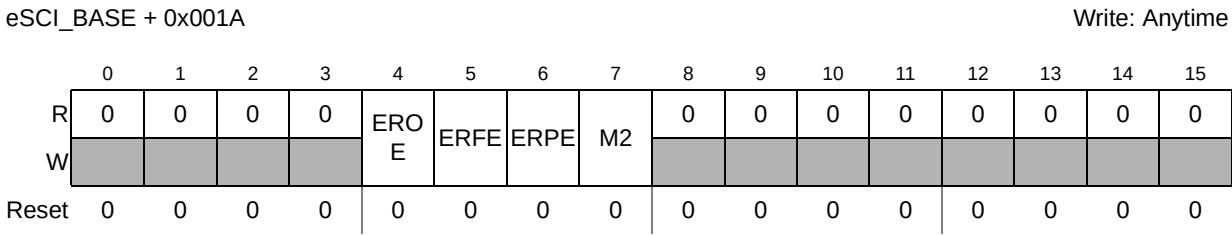
Figure 778. Control register 3 (eSCI_CR3)
