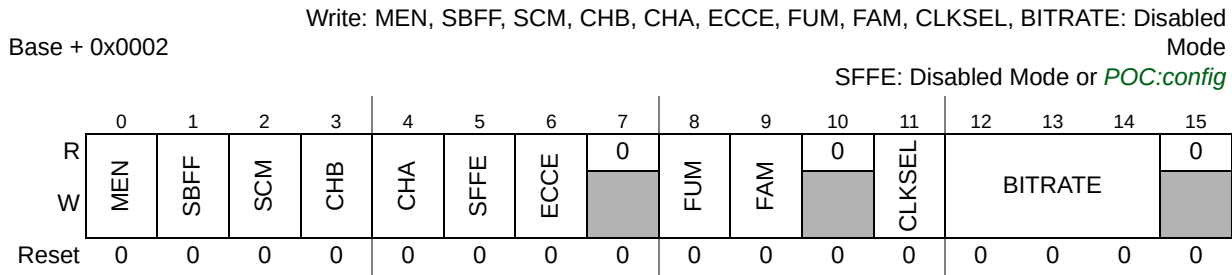
Figure 829. Module Configuration Register (FR_MCR)
