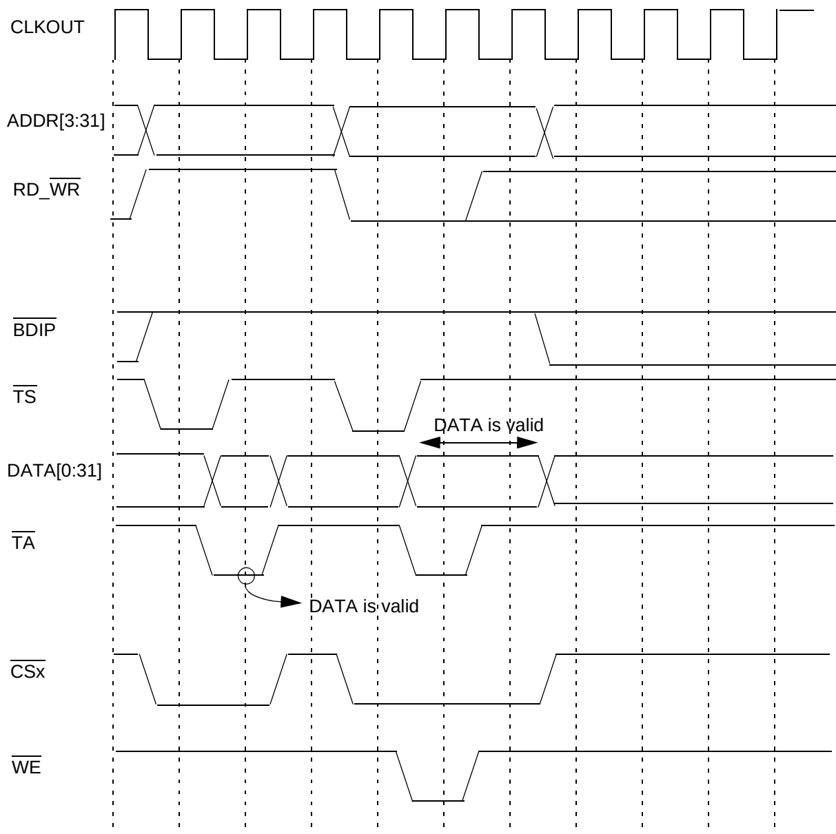
Figure 103. Write After Read to the Same \overline{\text{CS}} Bank
