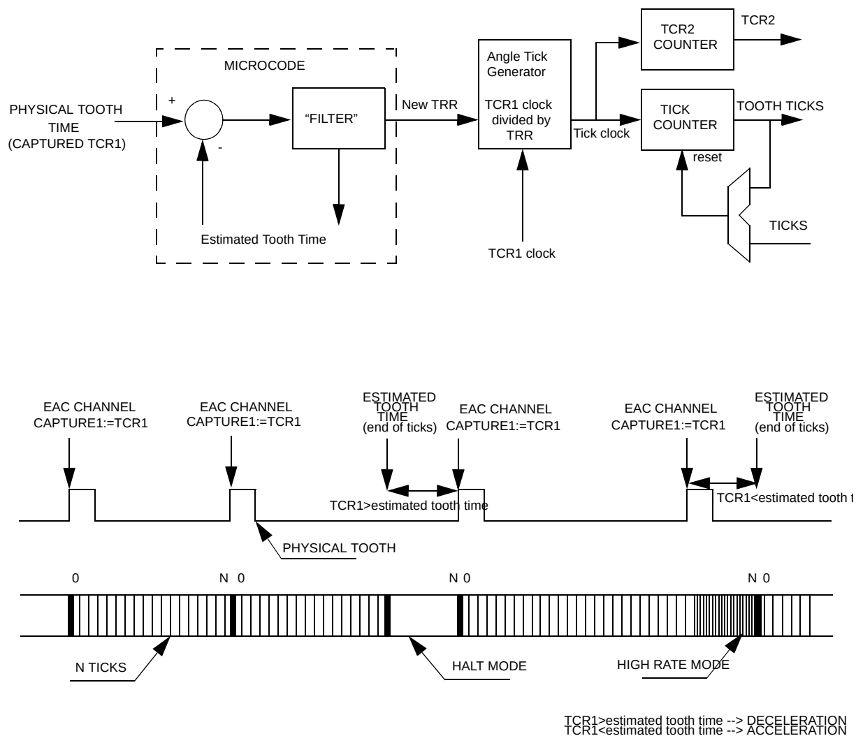
Figure 546. EAC “PLL”
