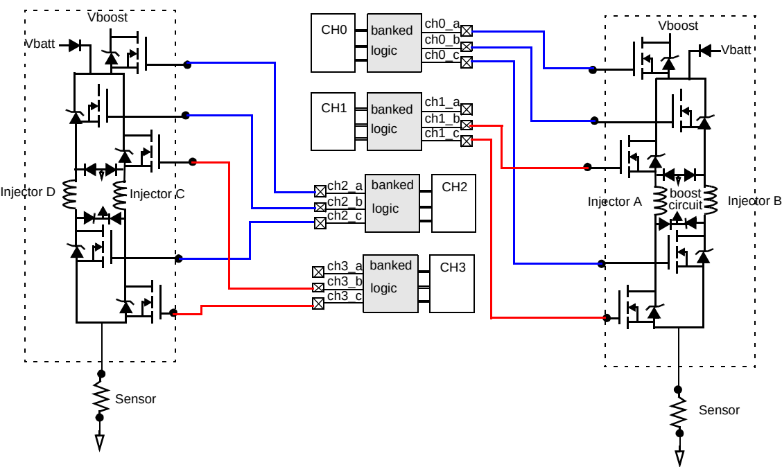
Figure 491. Four channels controlling two injector banks in banked mode
