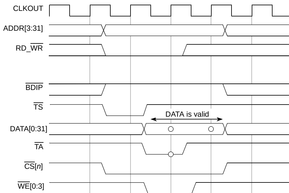
Figure 98. Single Beat 32-bit Write Cycle, \overline{\text{CS}} Access, Zero Wait States
