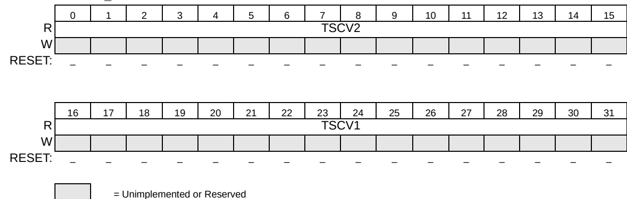
Figure 697. Temperature Calculation Constants Register 0 (TSENS_TCCR0)
