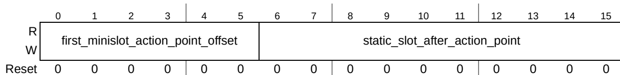
Figure 909. Protocol Configuration Register 13 (FR_PCR13)
