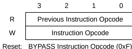
Figure 1016.4-bit Instruction Register
