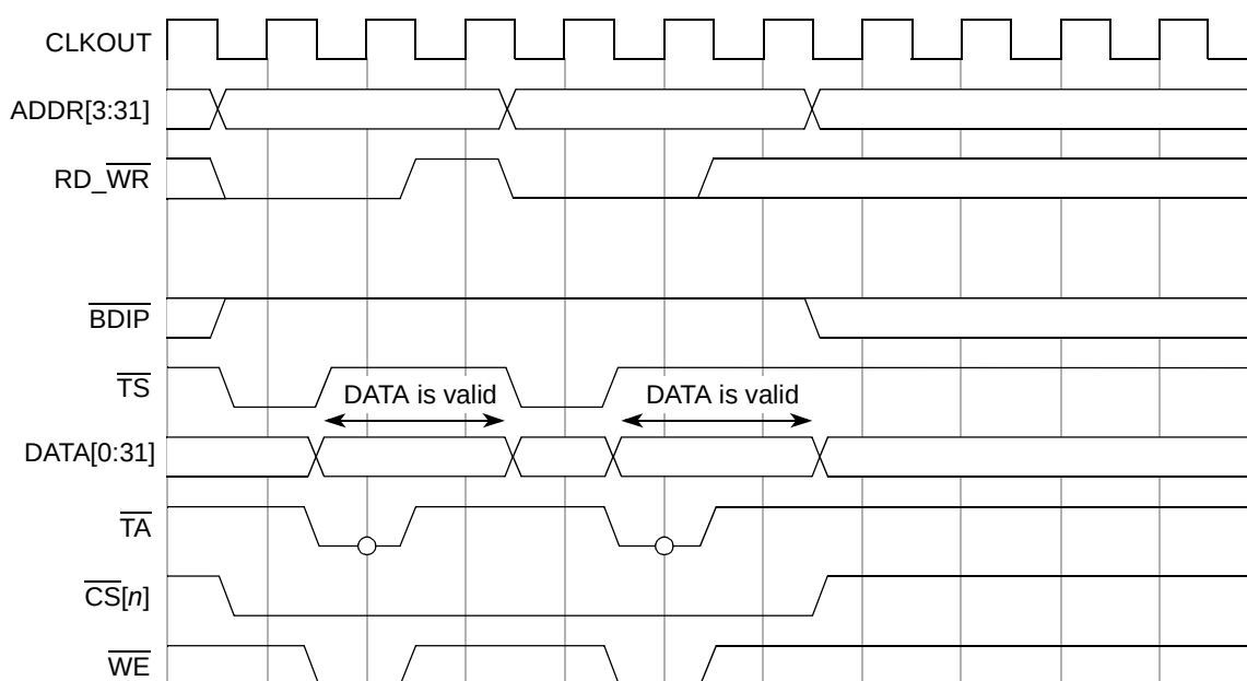
Figure 104. Back-to-Back 32-bit Writes to the Same \overline{\text{CS}} Bank
