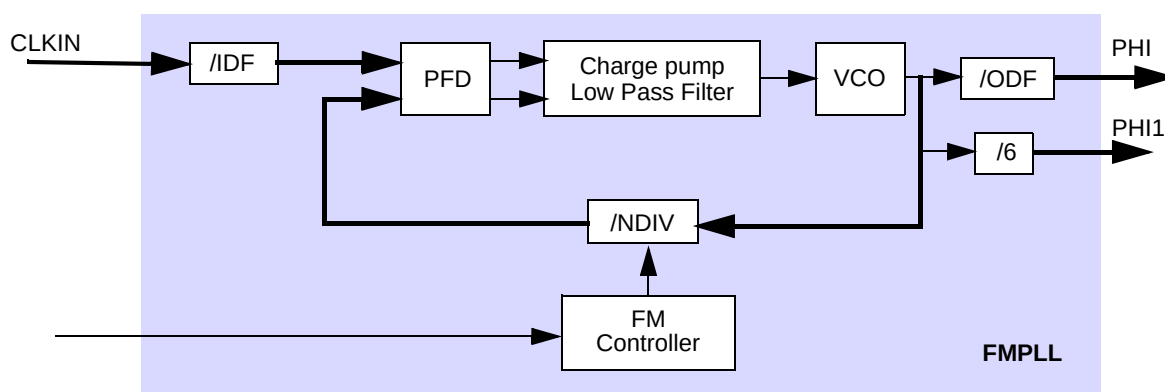
Figure 7. FMPLL
