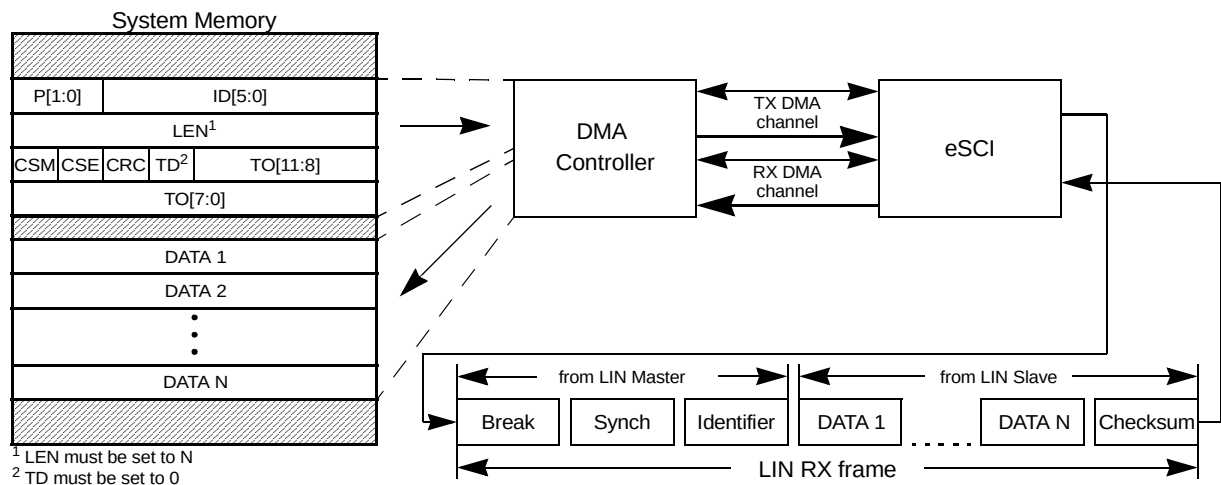
Figure 803. DMA Controlled LIN RX Frame generation and reception
