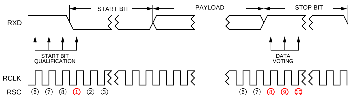
Figure 787. Faster Receiver
