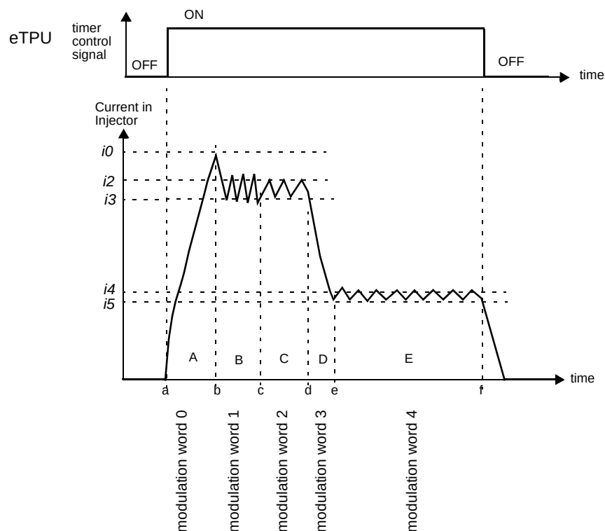
Figure 489. Advancing modulation phase on a threshold level
