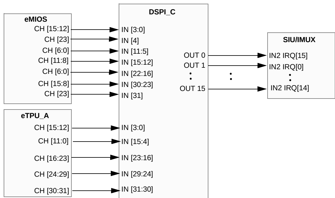
Figure 762. DSPI_C connectivity
