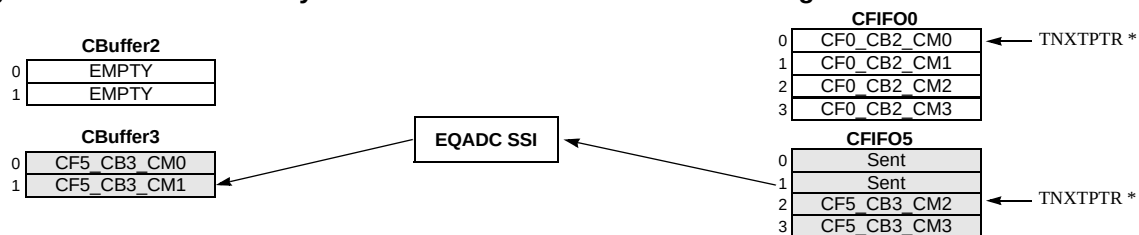
Figure 641. Non-Coherency Event when Different CFIFOs are using Different CBuffers
