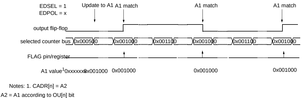
Figure 424. SAOC example toggling the output flip-flop
