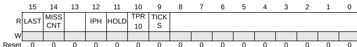
Figure 543. TPR Register
