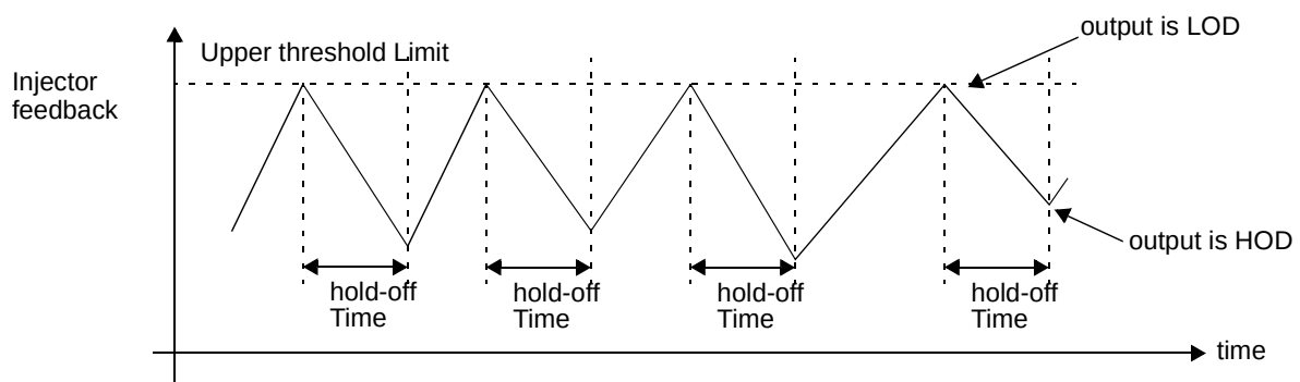
Figure 477. Threshold/hold-off modulation mode
