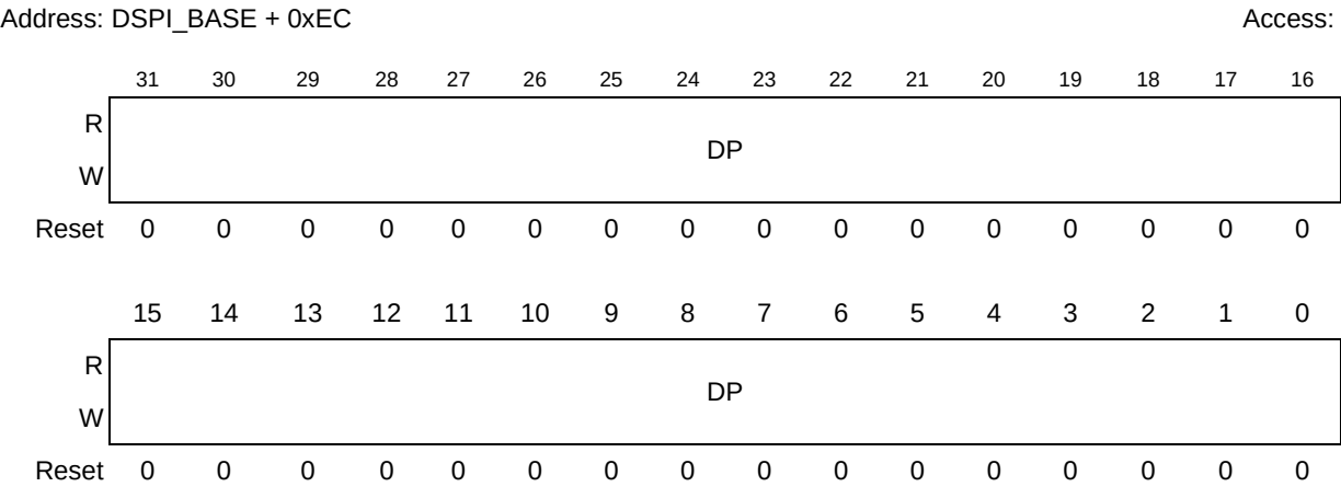
Figure 734. DSPI DSI Deserialized Data Polarity Interrupt Register (DSPI_DIPR)
