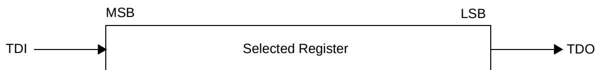
Figure 1013. Shifting data through a register
