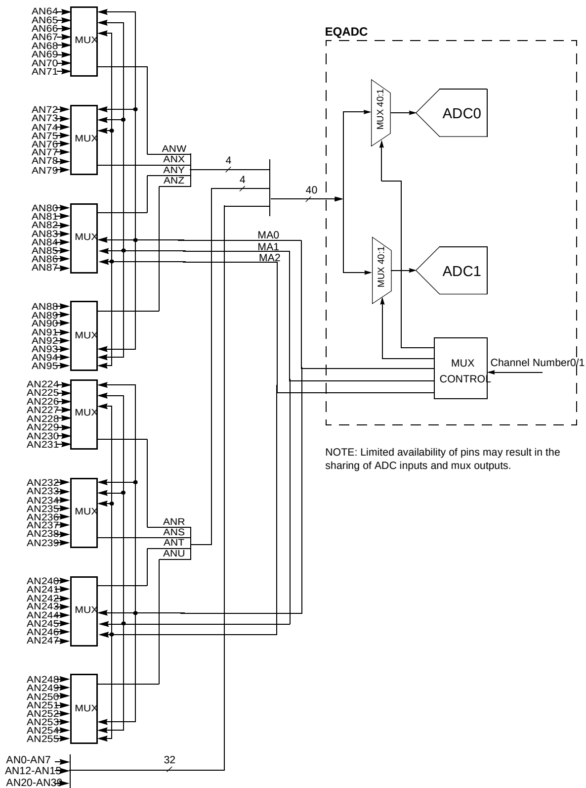
Figure 652. Example of External Multiplexing
