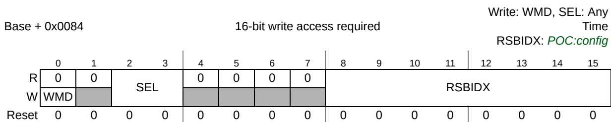
Figure 878. Receive Shadow Buffer Index Register (FR_RSBIR)
