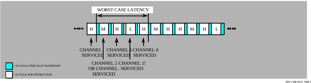
Figure 564. Worst-case latency for channel 0 (second try)
