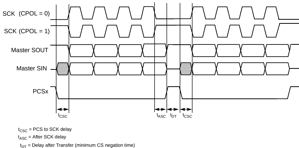
Figure 751. Example of non-continuous format (CPHA = 1, CONT = 0)
