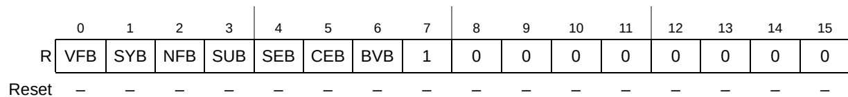
Figure 950. Receive message buffer slot status structure (ChB)
