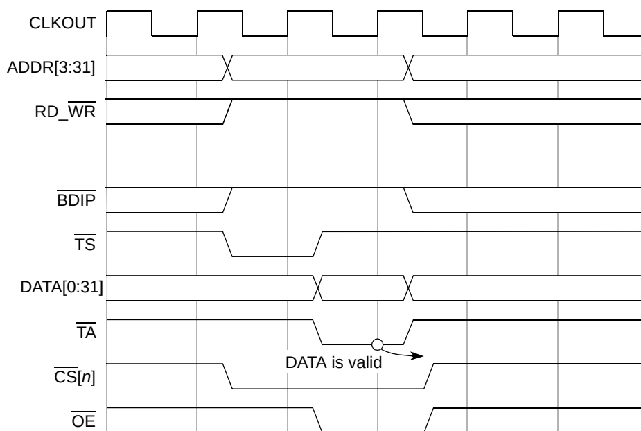
Figure 94. Single Beat 32-bit Read Cycle, \overline{\text{CS}} Access, Zero Wait States
