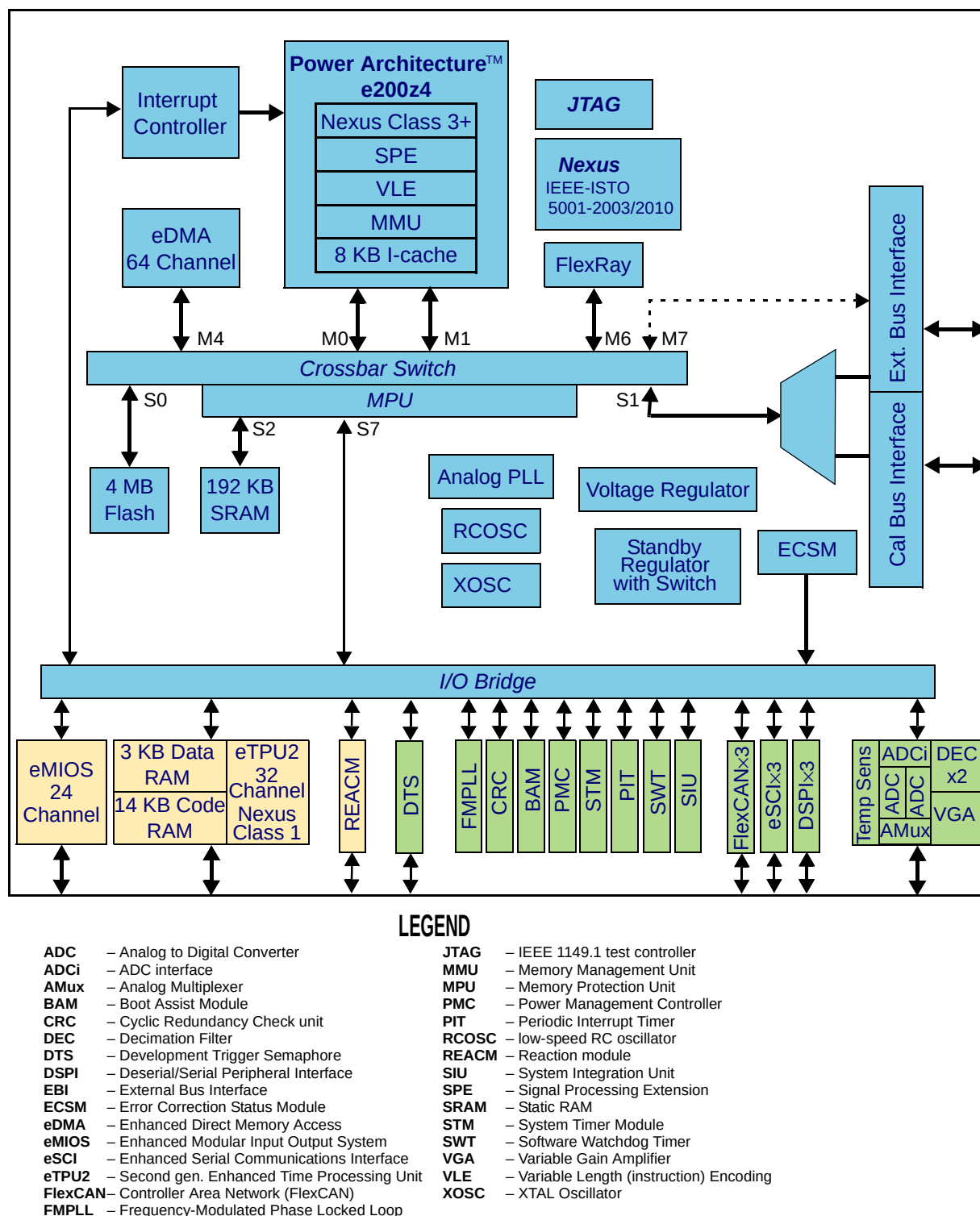
Figure 1. SPC564A74xx, SPC564A80xx Block Diagram
