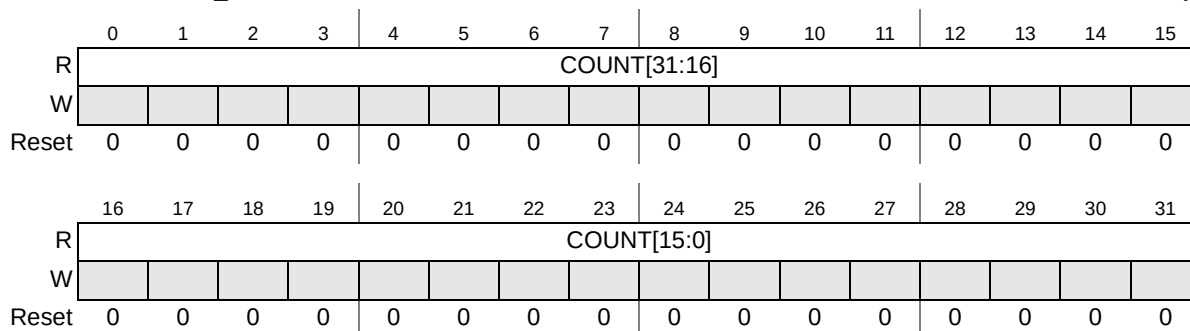
Figure 684. Decimation Filter Current Integration Count Value Register (DECFILTER_CINTCNT)
