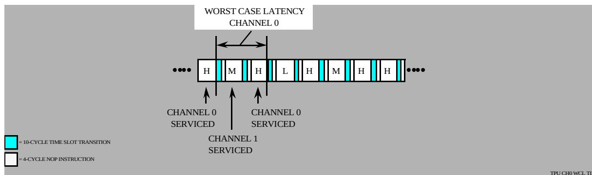
Figure 560. Next Servicing for Channel 0
