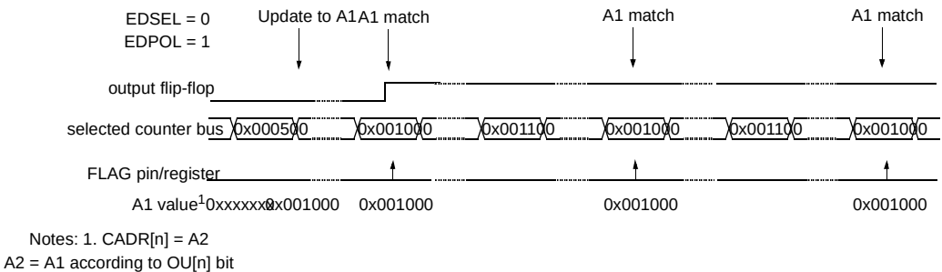
Figure 423. SAOC example with EDPOL value being transferred to the output flip-flop
