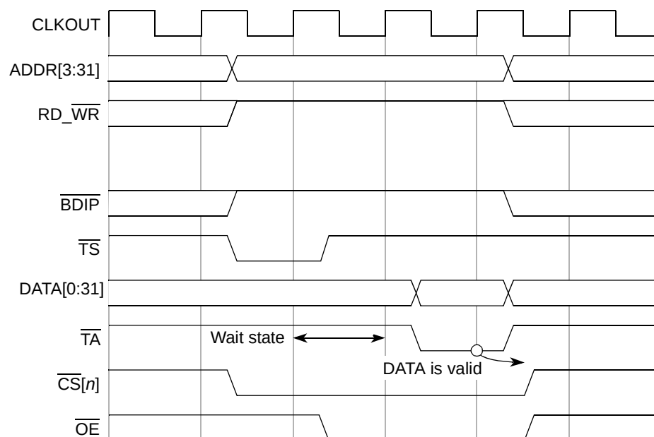
Figure 95. Single Beat 32-bit Read Cycle, \overline{\text{CS}} Access, One Wait State
