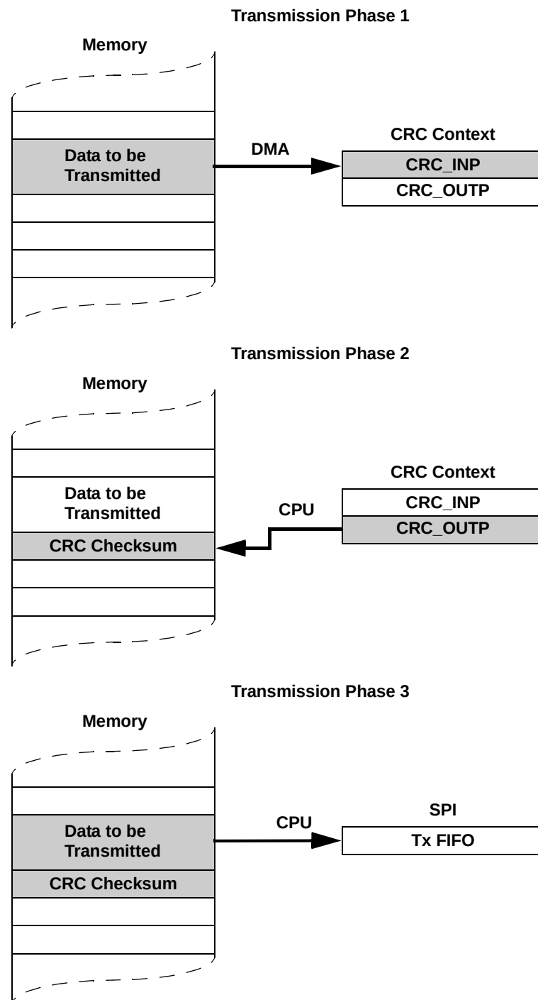
Figure 704. Transmission sequence
