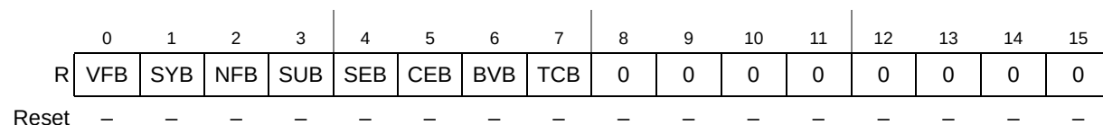
Figure 953. Transmit message buffer slot status structure (ChB)
