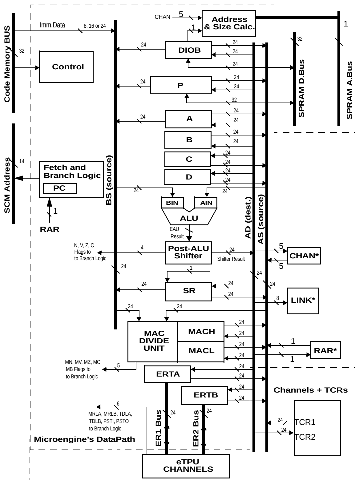
Figure 553. Microengine Block Diagram
