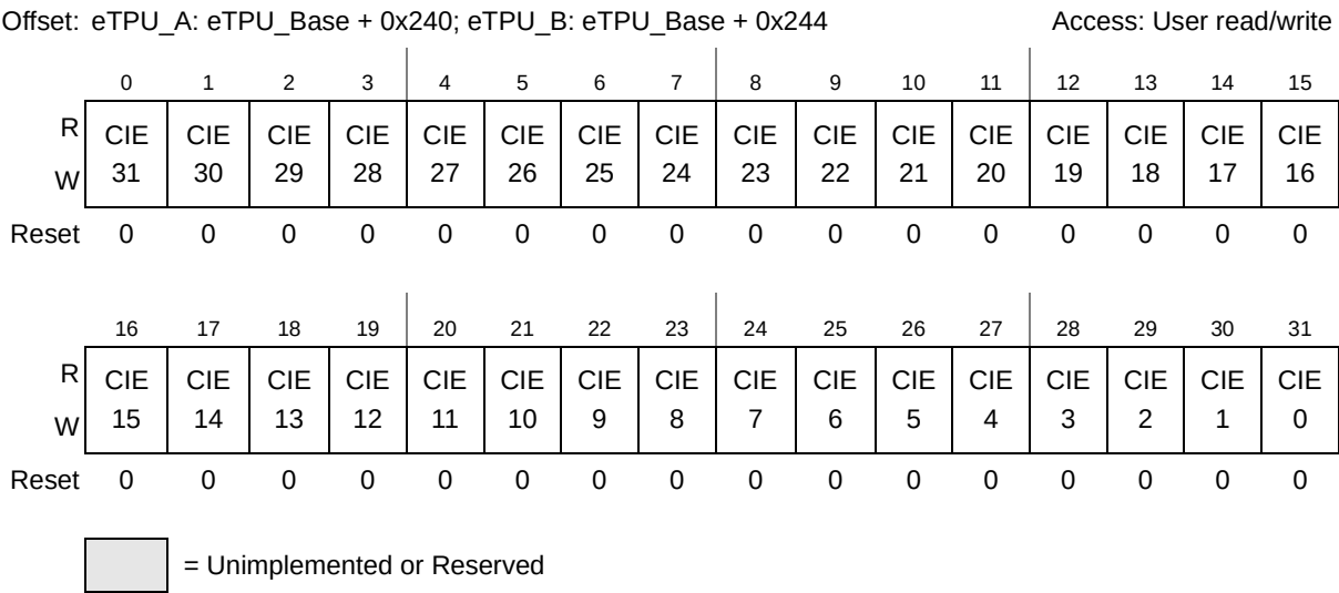
Figure 508. ETPU_CIER Register
