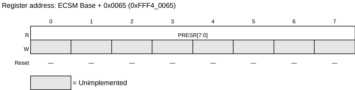
Figure 384. RAM ECC Syndrome Register (ECSM_PRESR)
