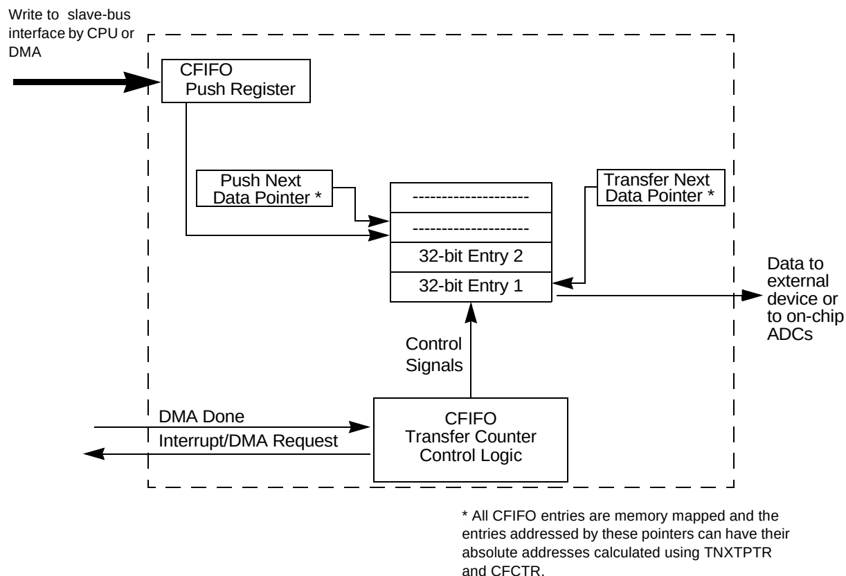
Figure 629. CFIFO Diagram
