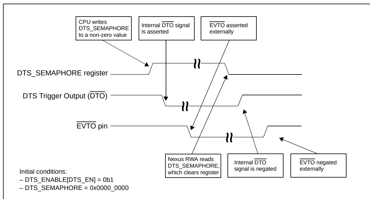
Figure 1027.DTSO event sequence
