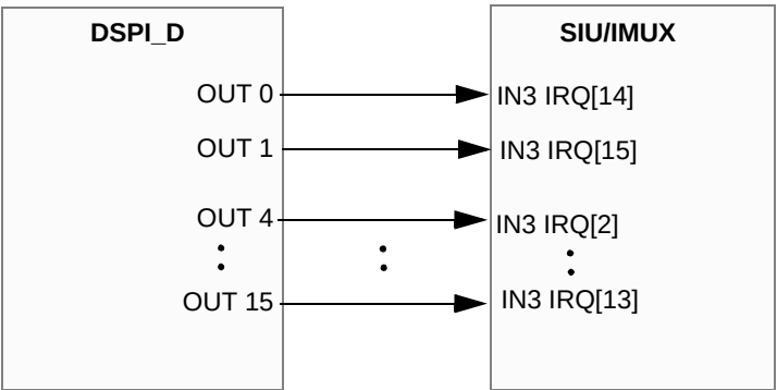
Figure 763. DSPI_D connectivity
