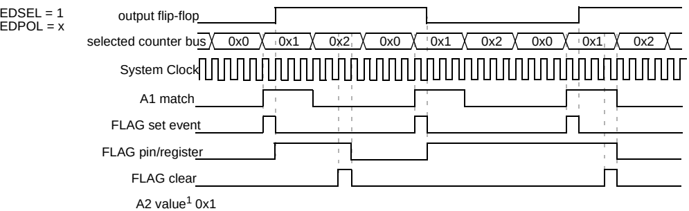
Figure 424. SAOC example toggling the output flip-flop
