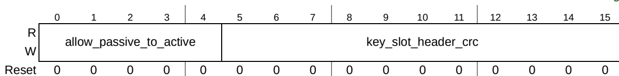
Figure 908. Protocol Configuration Register 12 (FR_PCR12)
