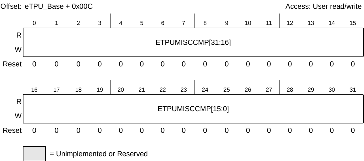
Figure 496. ETPU_MISCCMPR Register
