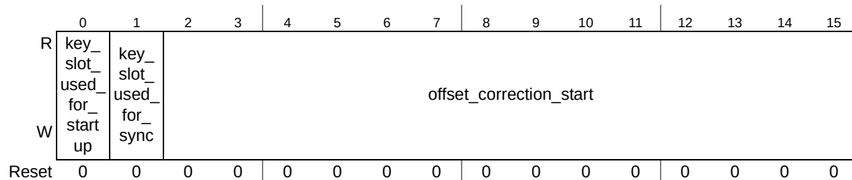
Figure 907. Protocol Configuration Register 11 (FR_PCR11)
