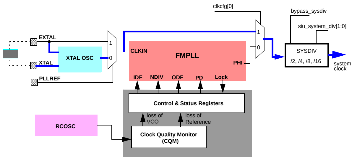
Figure 8. Bypass mode with crystal reference
