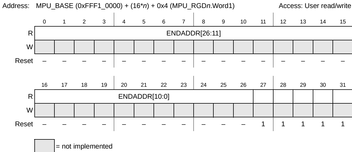
Figure 81. MPU Region Descriptor n , Word 1 Register (MPU_RGD n .Word1)
