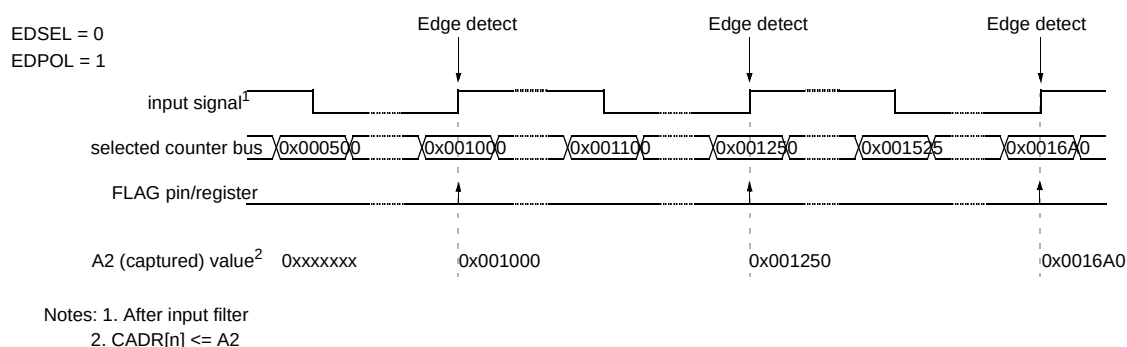
Figure 421. Single Action Input Capture with rising edge triggering example
