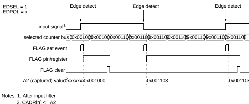
Figure 422. Single Action Input Capture with both edges triggering example
