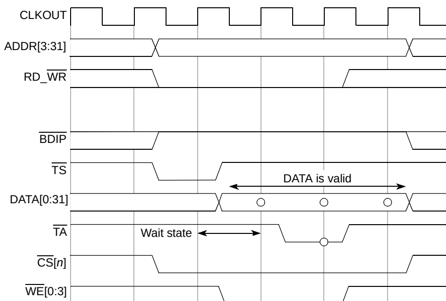
Figure 99. Single Beat 32-bit Write Cycle, \overline{\text{CS}} Access, One Wait State
