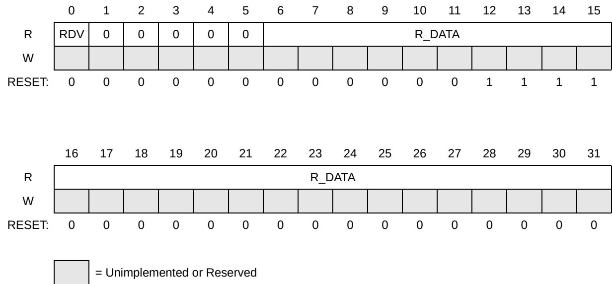
Figure 592. EQADC SSI Receive Data Register (EQADC_SSIRDR)
