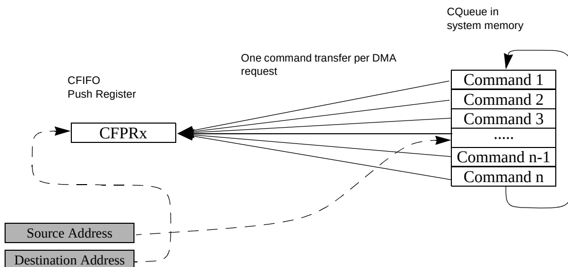
Figure 665. CQueue/CFIFO Interface
