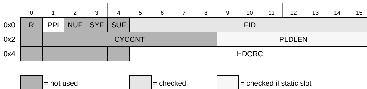
Figure 946. Frame header structure (transmit message buffer)
