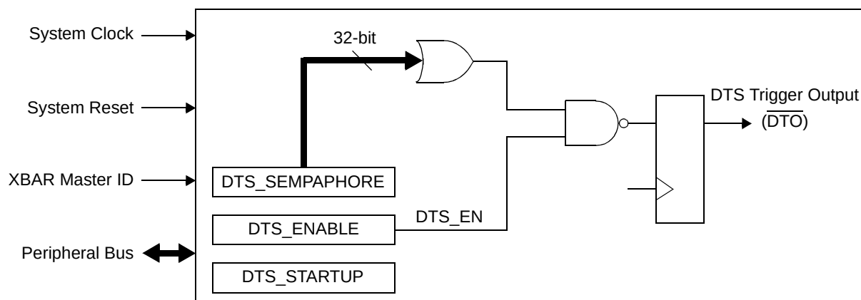
Figure 1026.DTS block diagram
