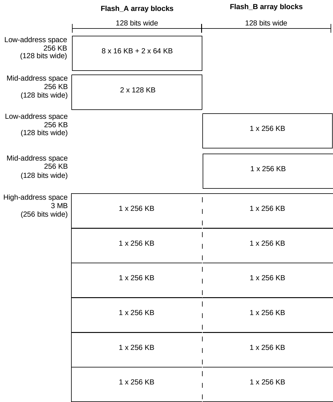
Figure 55. Flash segmentation
