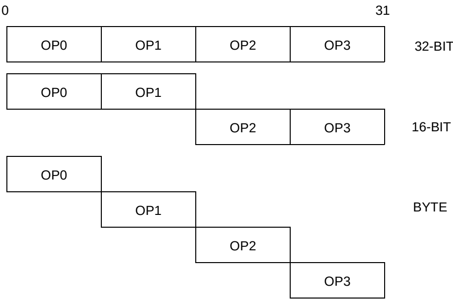
Figure 115. Internal Operand Representation
