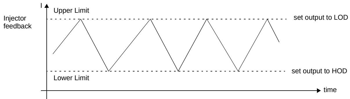
Figure 476. Threshold/threshold modulation mode
