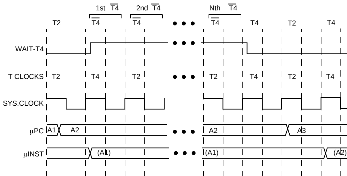
Figure 569. \overline{T4} timing
