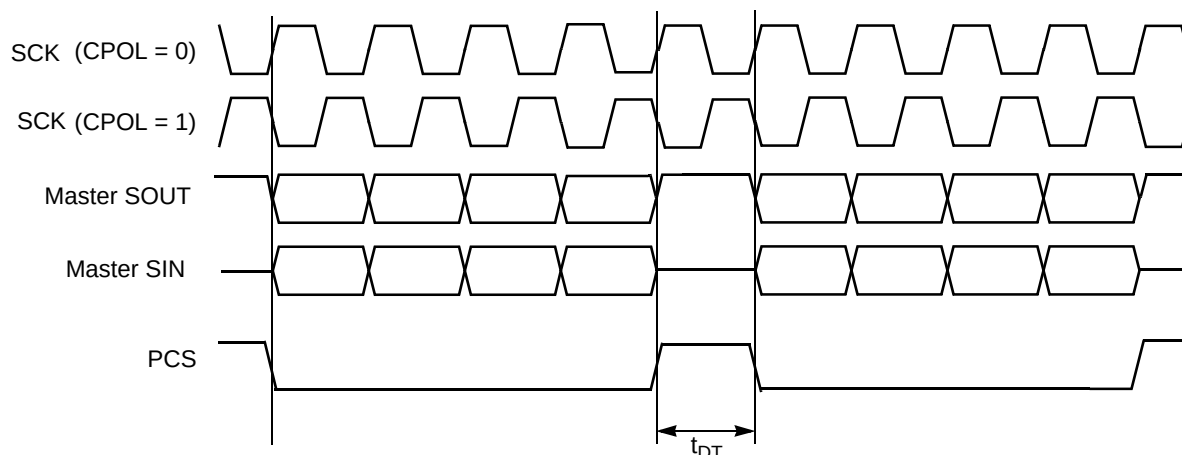
Figure 753. Continuous SCK timing diagram (CONT = 0)
