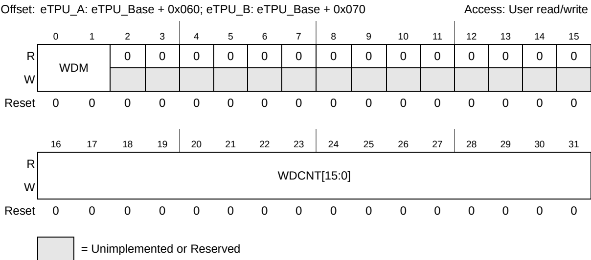
Figure 501. ETPU_WDTR Register
