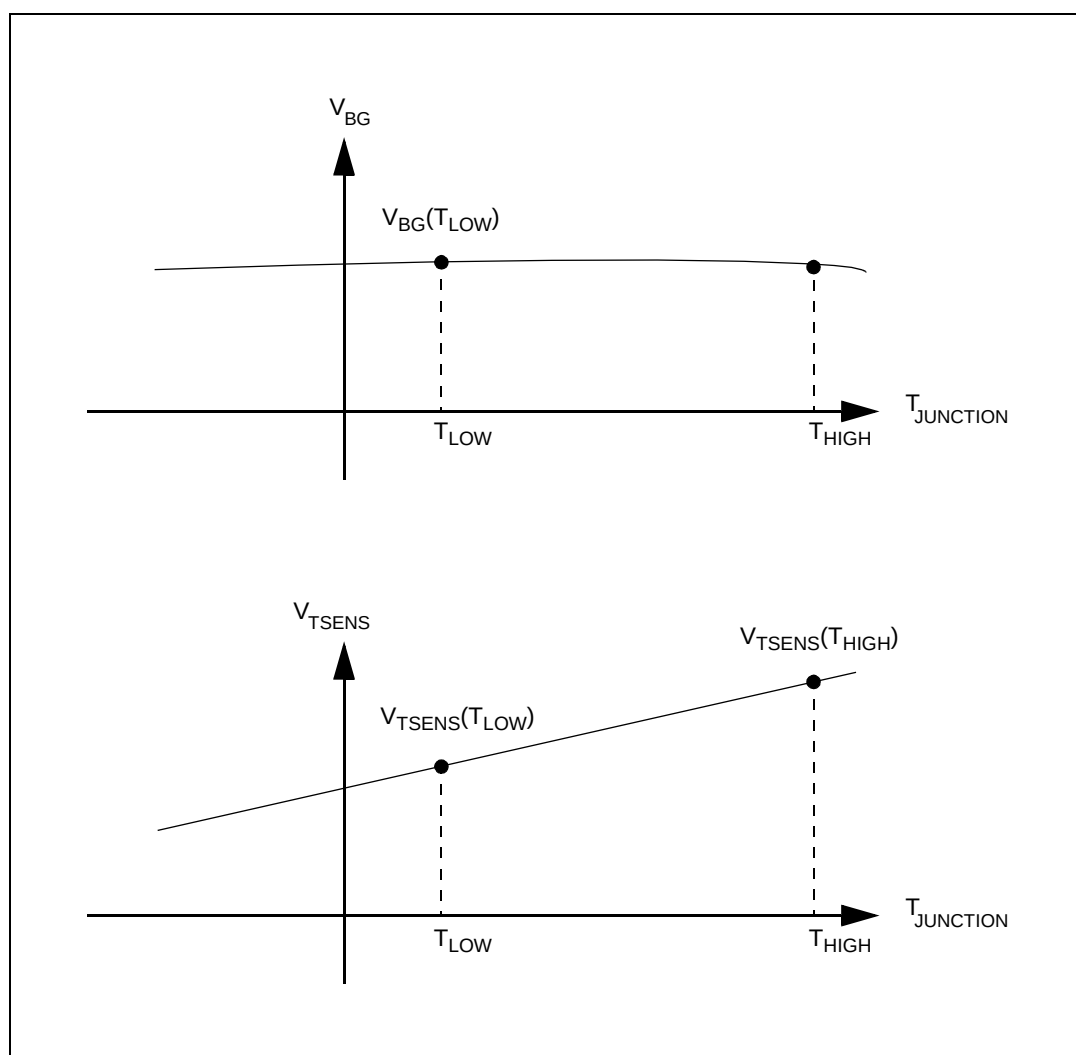
Figure 695. Calibration points
