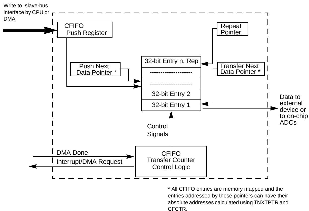
Figure 631. CFIFO0 in Streaming Mode Diagram
