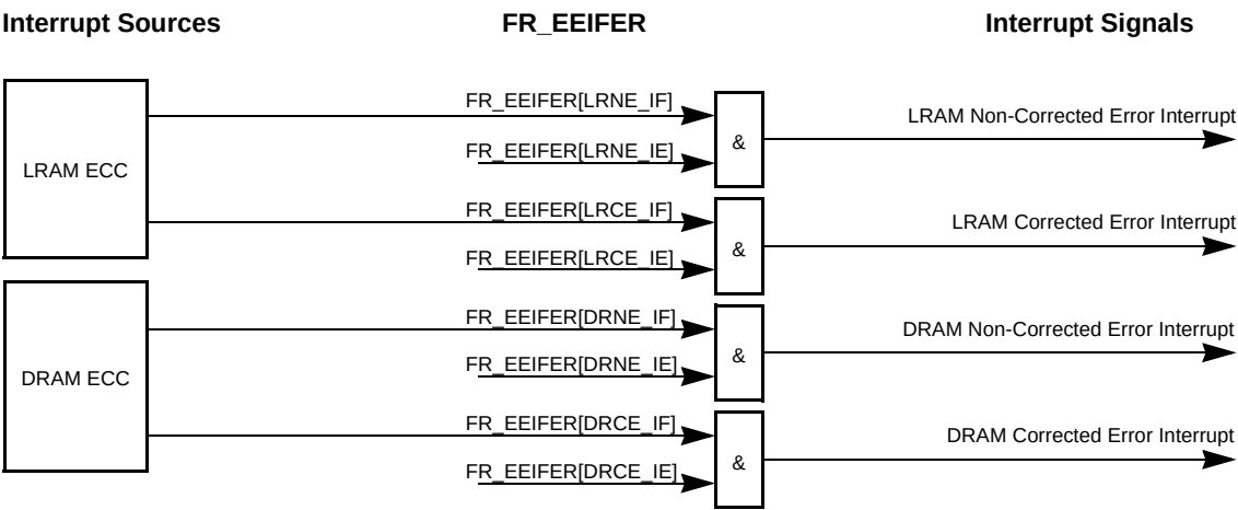
Figure 987. Scheme of FR_EEIFER interrupt signal generation
