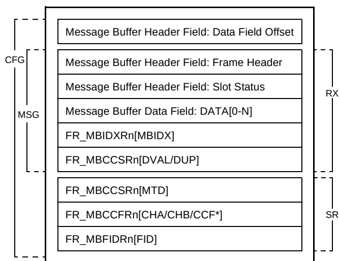
Figure 963. Receive message buffer access regions
