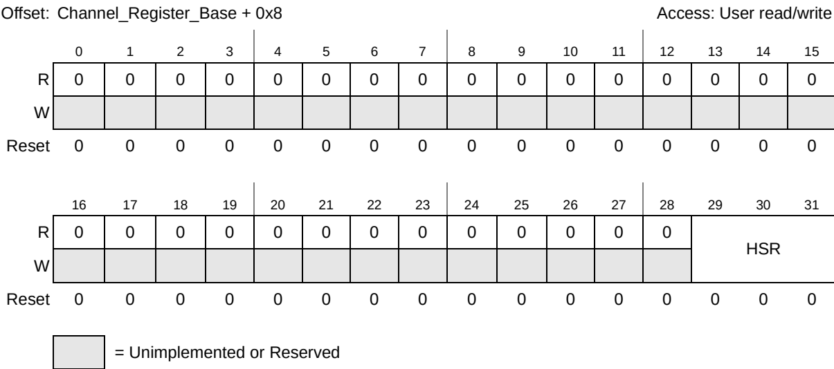
Figure 514. ETPU_CxHSRR Register
