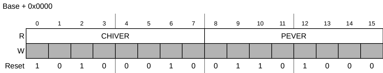
Figure 828. Module Version Register (FR_MVR)
