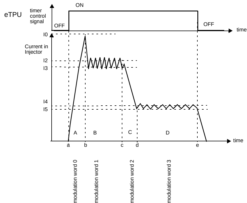
Figure 487. Modulation phases
