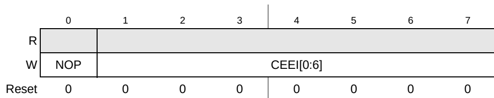
Figure 29. eDMA Clear Enable Error Interrupt Register (EDMA_CEEIR)
