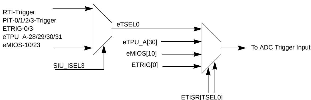
Figure 363. eQADC trigger input multiplexing example
