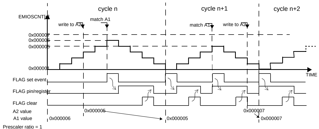
Figure 434. Modulus Counter Buffered (MCB) Up/Down Mode
