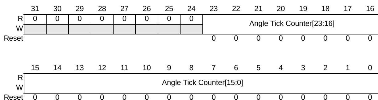
Figure 544. TCR2 in Angle Mode
