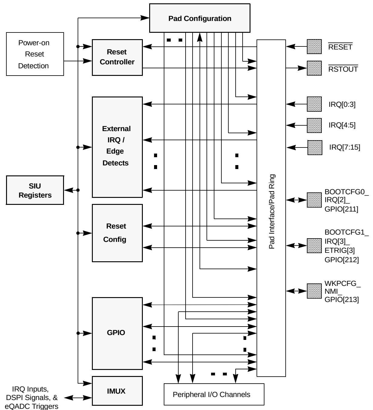
Figure 143. SIU block diagram
