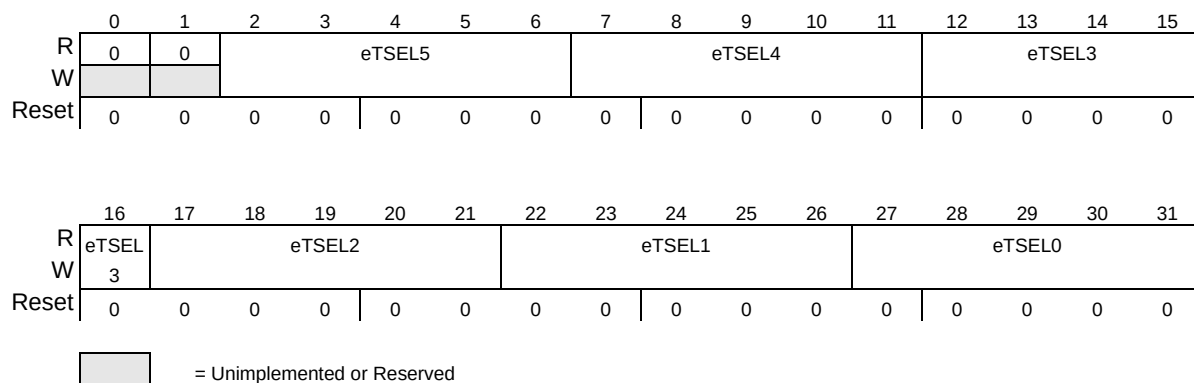
Figure 348. IMUX Select Register 3 (SIU_ISEL3)
