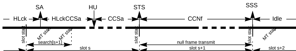
Figure 961. Null frame transmission from HLck state with unlock
