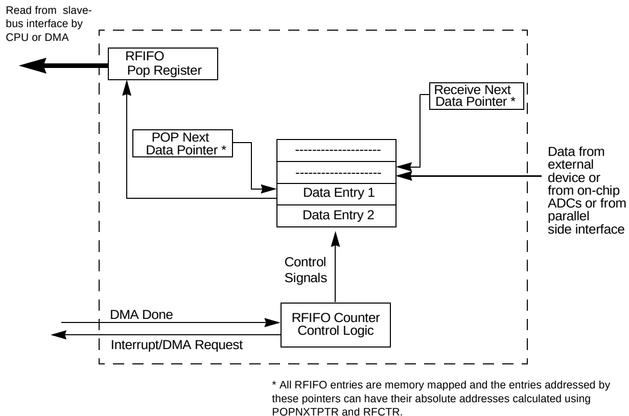
Figure 643. RFIFO Diagram
