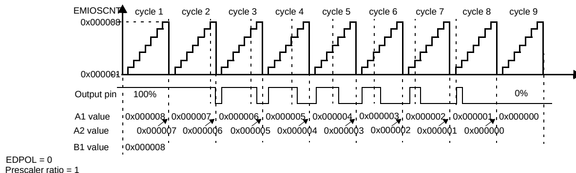
Figure 441. OPWFMB mode from 100% to 0% duty cycle
