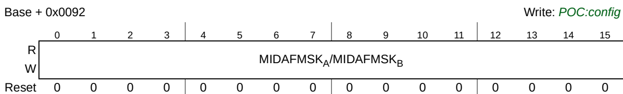
Figure 889. Receive FIFO Message ID Acceptance Filter Mask Register (FR_RFMIDAFMR)
