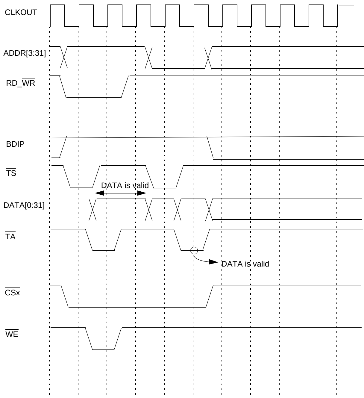
Figure 105. Read After Write to the Same \overline{CS} Bank
