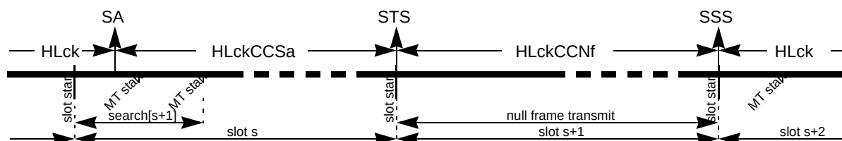
Figure 960. Null frame transmission from HLck state
