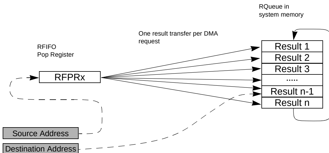
Figure 666. RQueue/RFIFO Interface
