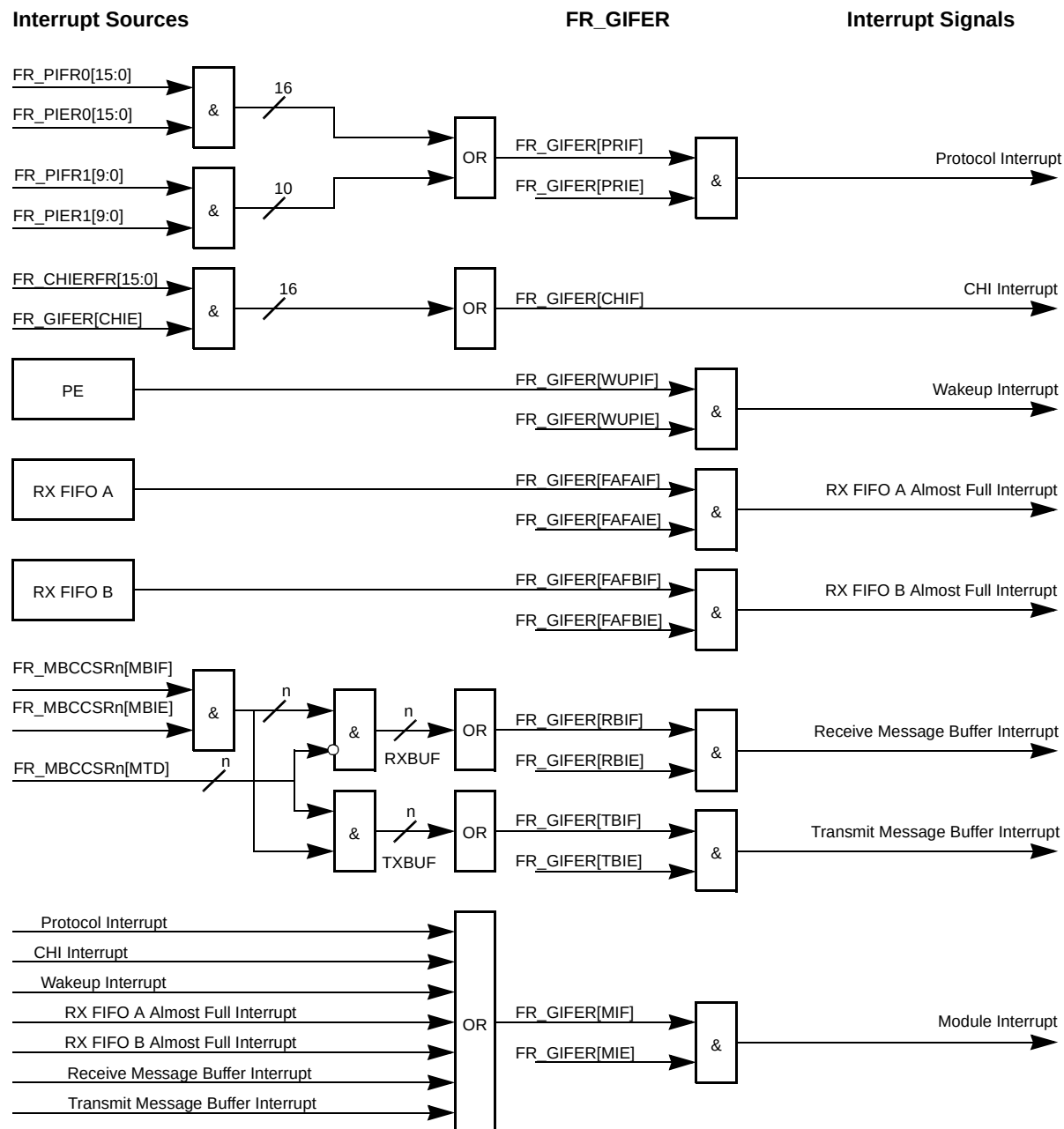
Figure 986. Scheme of FR_GIFER interrupt signal generation
