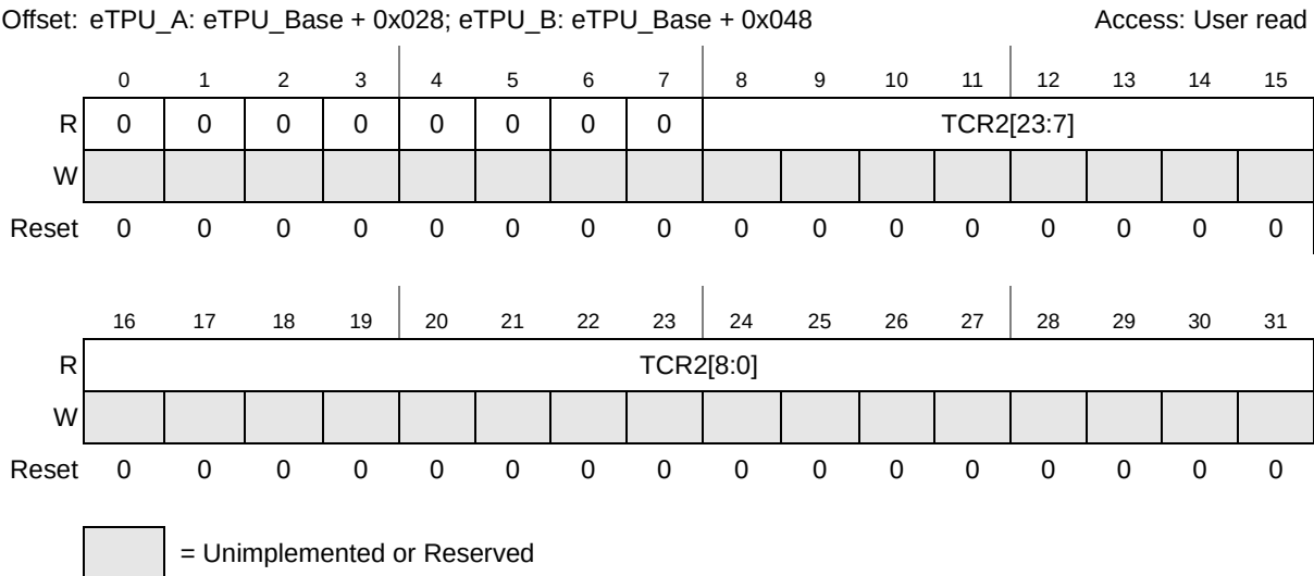
Figure 499. ETPU_TB2R Register
