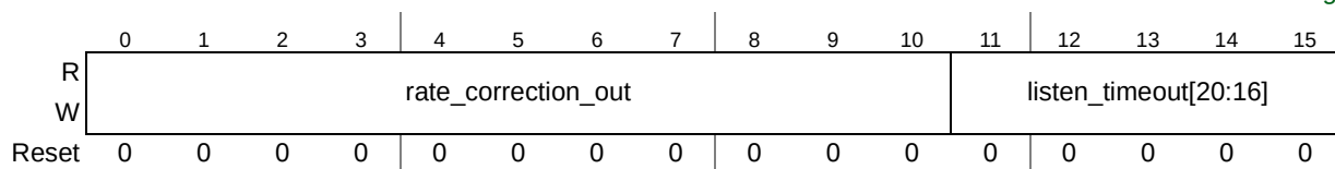
Figure 910. Protocol Configuration Register 14 (FR_PCR14)
