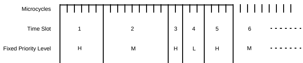
Figure 525. Time-slot variation
