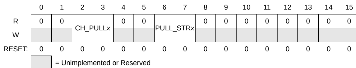
Figure 616. ADC Pull Up/Down Control Register x (ADC_PUDCRx, x=0-7)
