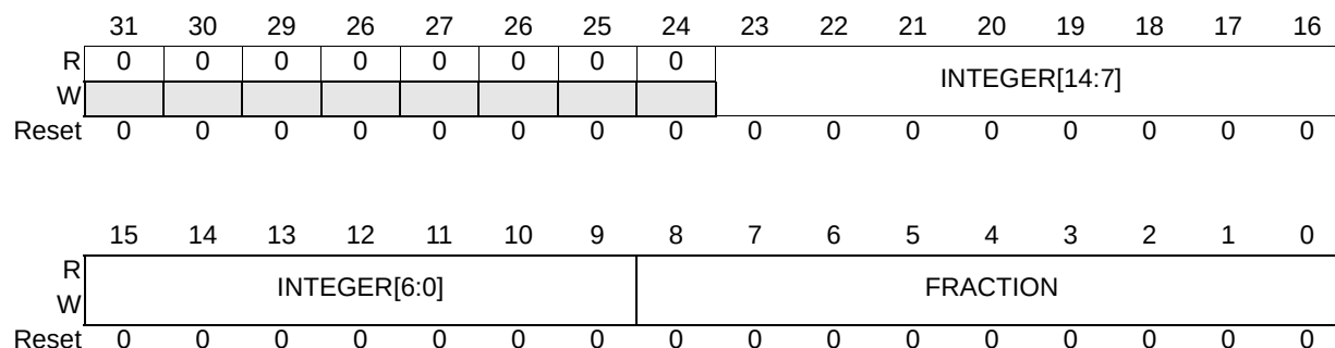
Figure 545. TRR Register
