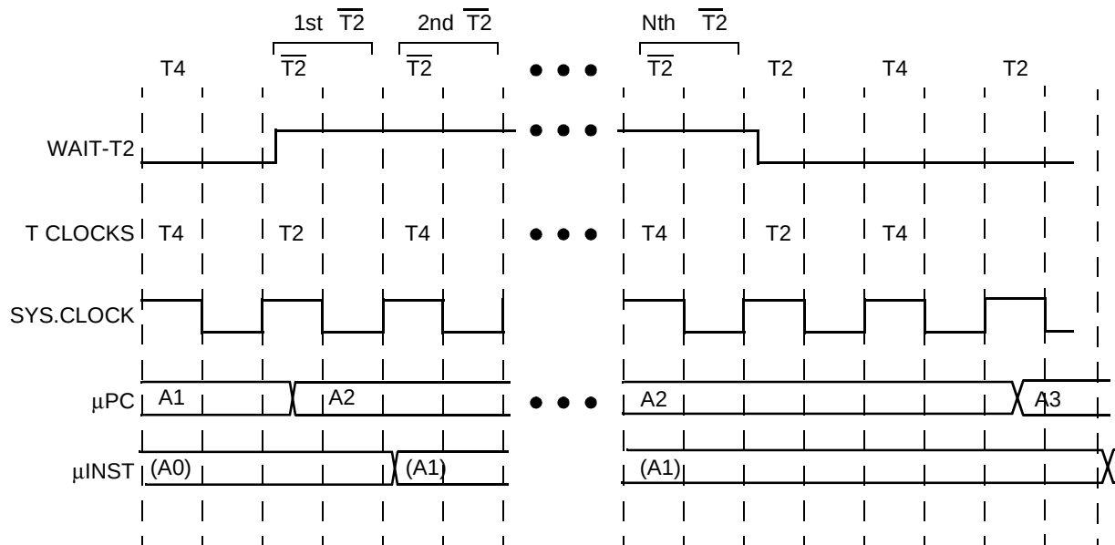
Figure 568. \overline{T2} timing
