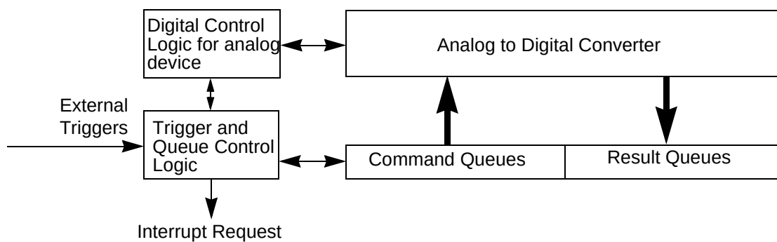
Figure 669. QADC Overview
