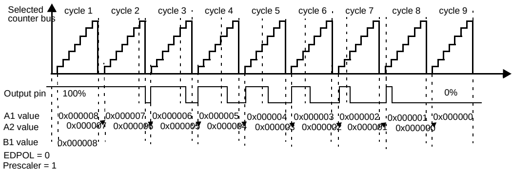
Figure 445. OPWMB mode from 100% to 0% duty cycle
