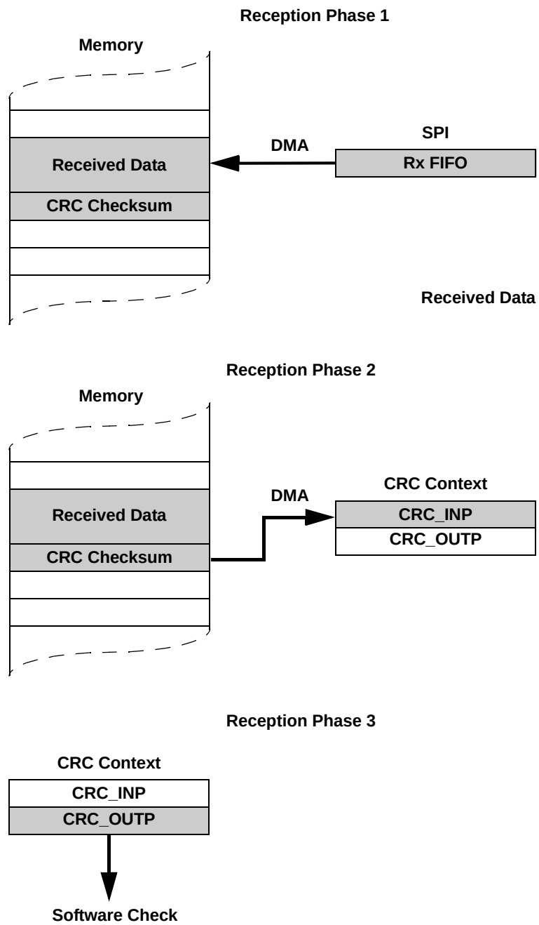
Figure 705. Reception sequence
