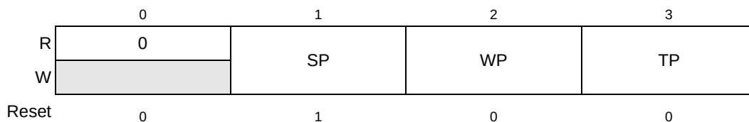
Figure 53. PACR n field structure
