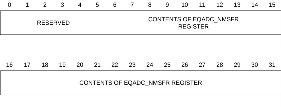
Figure 628. Null Message Receive Format for External Device Operation
