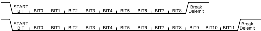
Figure 784. LIN Break Symbol Format
