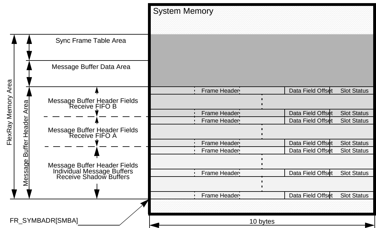
Figure 943. Example of FlexRay memory area layout (FR_MCR[FAM] = 0)
