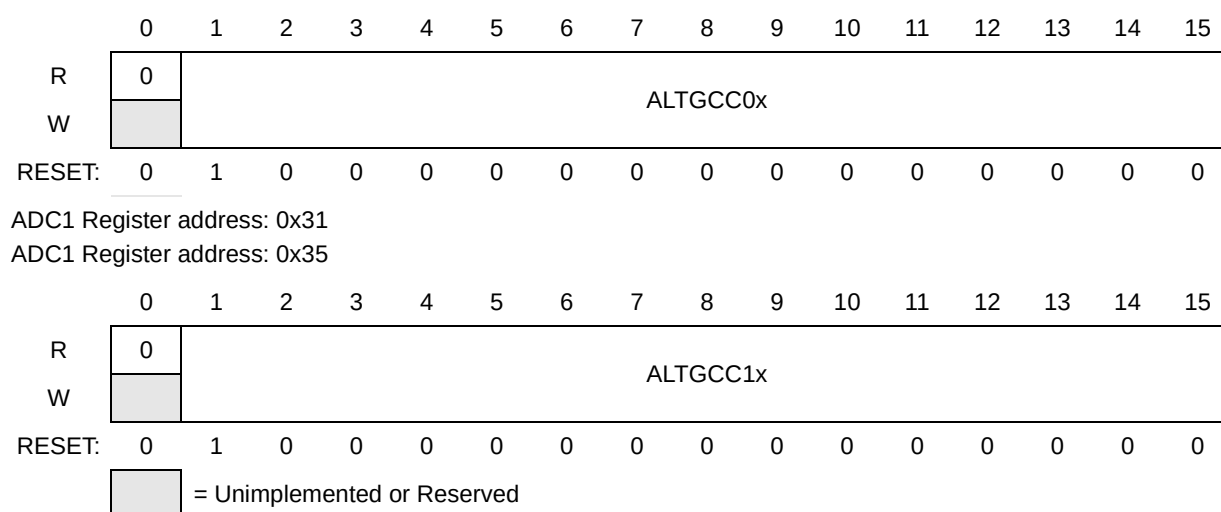
Figure 614. ADC0/1 Alternate x Gain Register (ADC0/1_AGRx, x=1-2) field description
