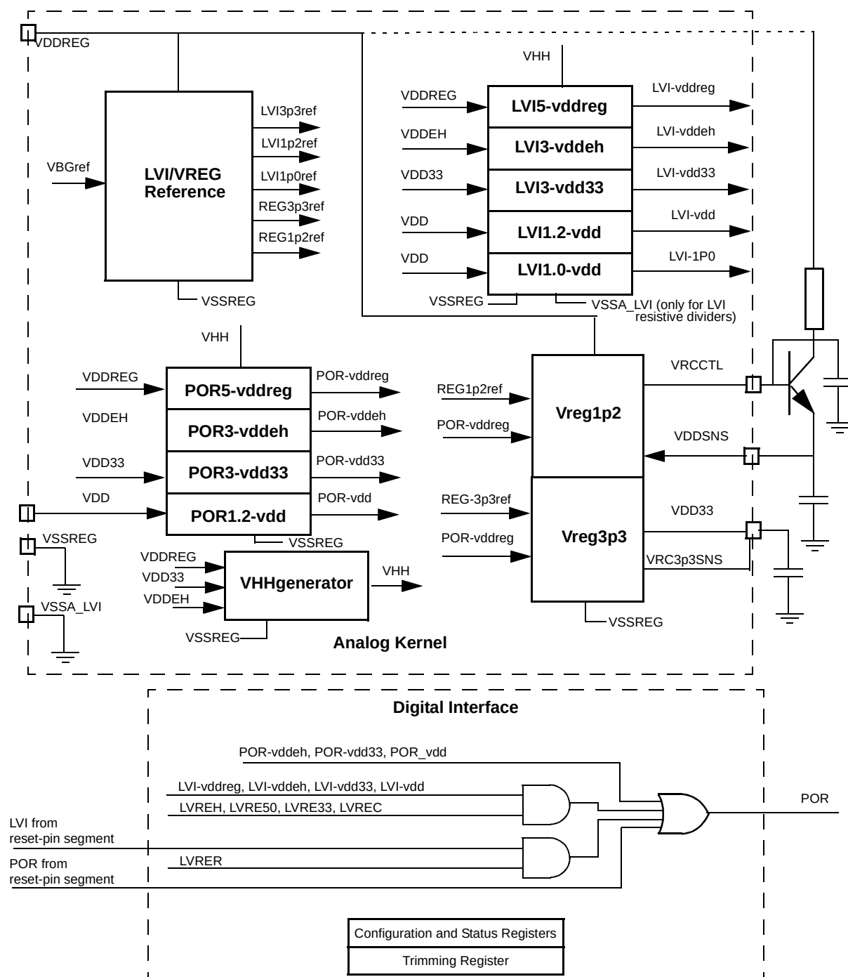
Figure 1000. Power management controller diagram
