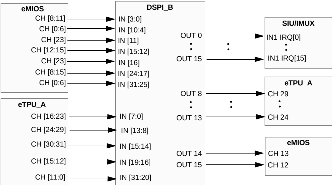
Figure 761. DSPI_B connectivity
