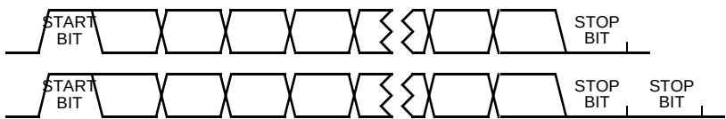
Figure 783. Inverted SCI Frame Formats
