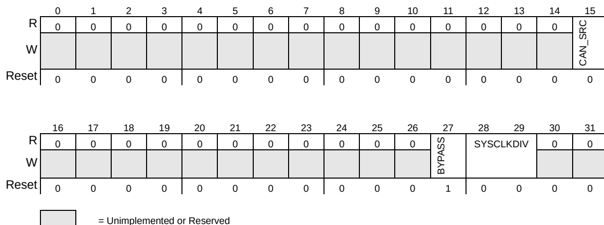
Figure 358. System Clock Register (SIU_SYSDIV)
