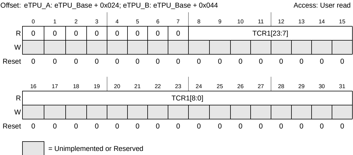
Figure 498. ETPU_TB1R Register
