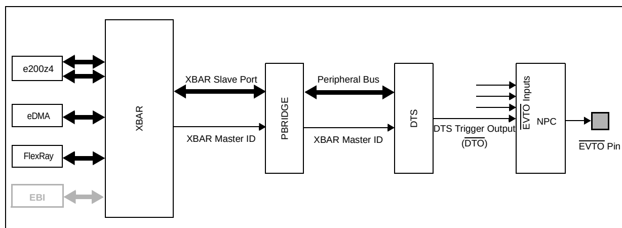
Figure 1028.DTS device connections
