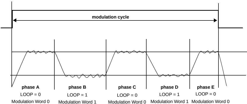
Figure 490. LOOP function used within a modulation cycle
