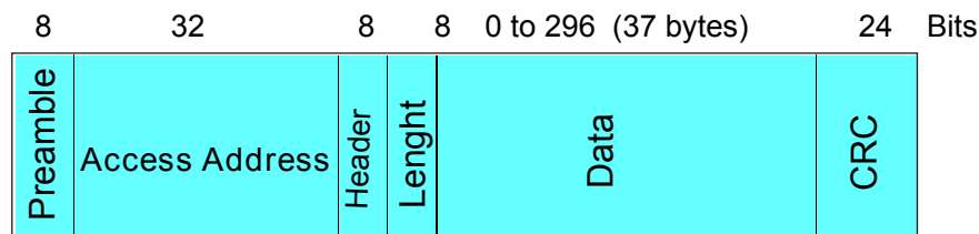
Figure 4. Packet structure
