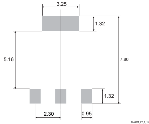
Figure 14. SOT-223 footprint (dimensions in mm)
