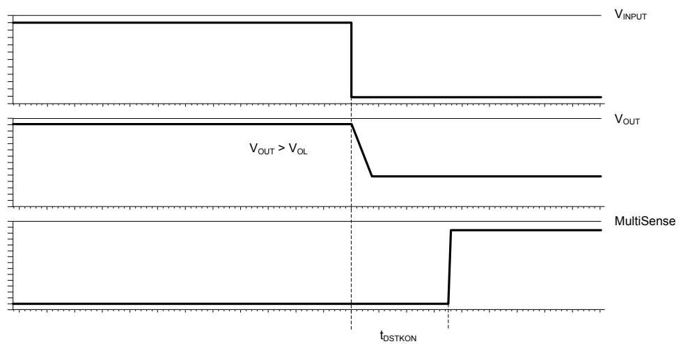
Figure 6. T_{\text{DSTKON}}
