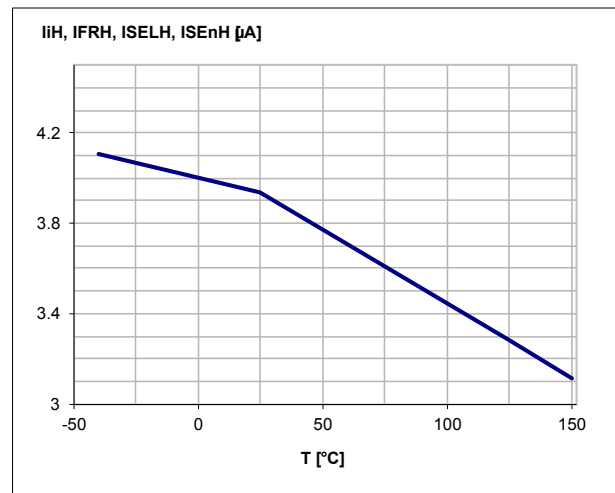
Figure 12. High level logic input current
