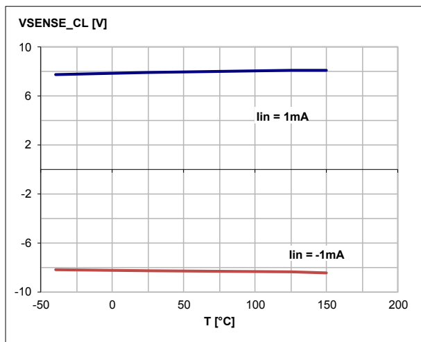
Figure 25. V_{\text{Sense clamp}} vs T_C
