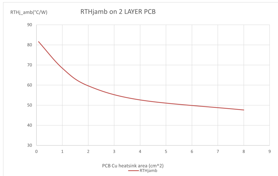
Figure 43. Thermal_curves
