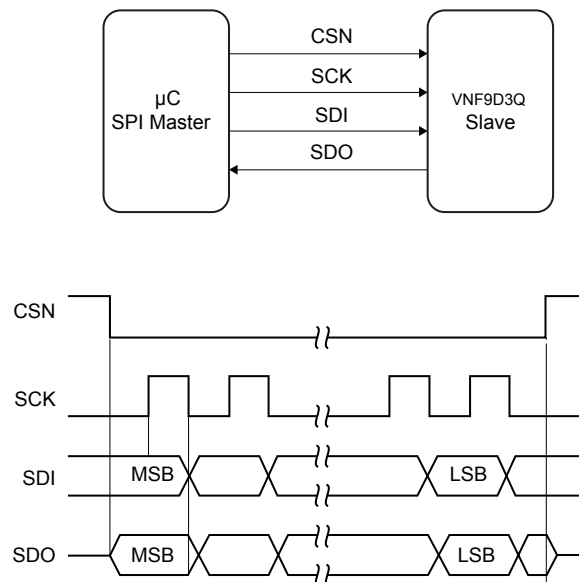
Figure 9. Supported SPI mode
