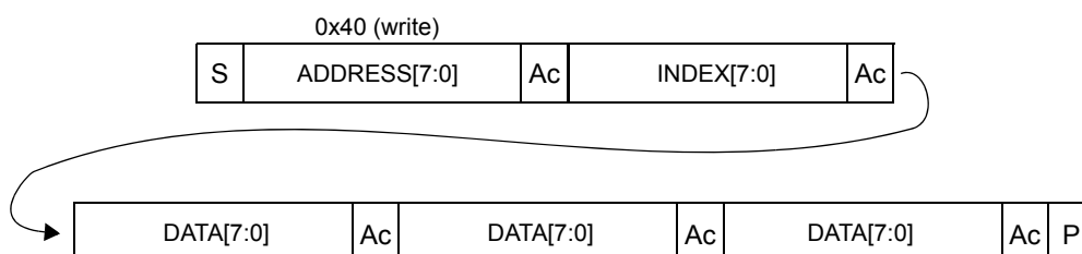
Figure 12. Data format (sequential write)
