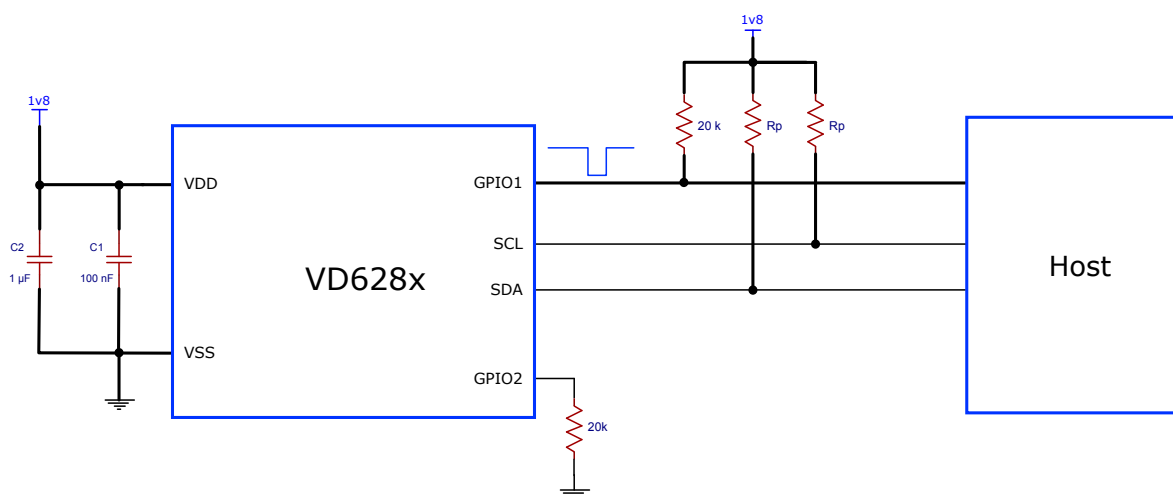
Figure 4. Application schematic, ALS, and flicker in digital PDM format (mode 1)
