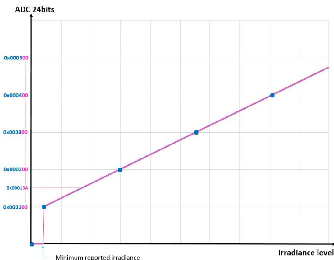
Figure 7. 24-bit ADC readout vs. light level
