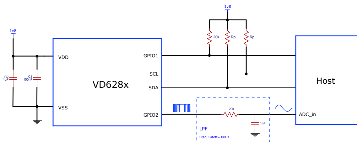
Figure 5. Application schematic, ALS, and flicker in analog format (mode 2)
