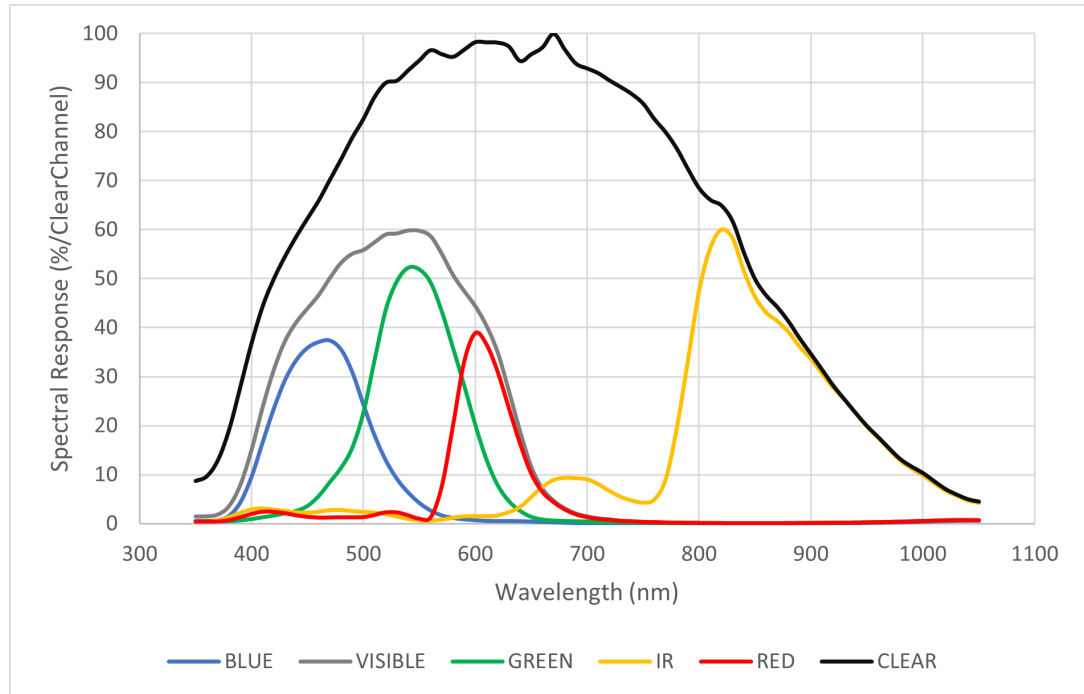
Figure 18. VD6283TX45/1 spectral response (full color set RGBIRClear)
