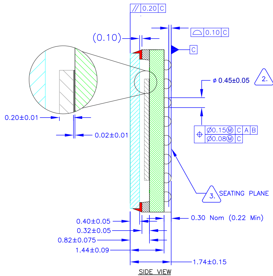
Figure 12. Side view
