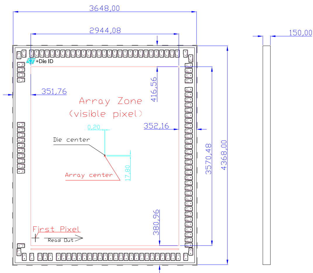
Figure 10. Die mechanical dimensions (μm)
