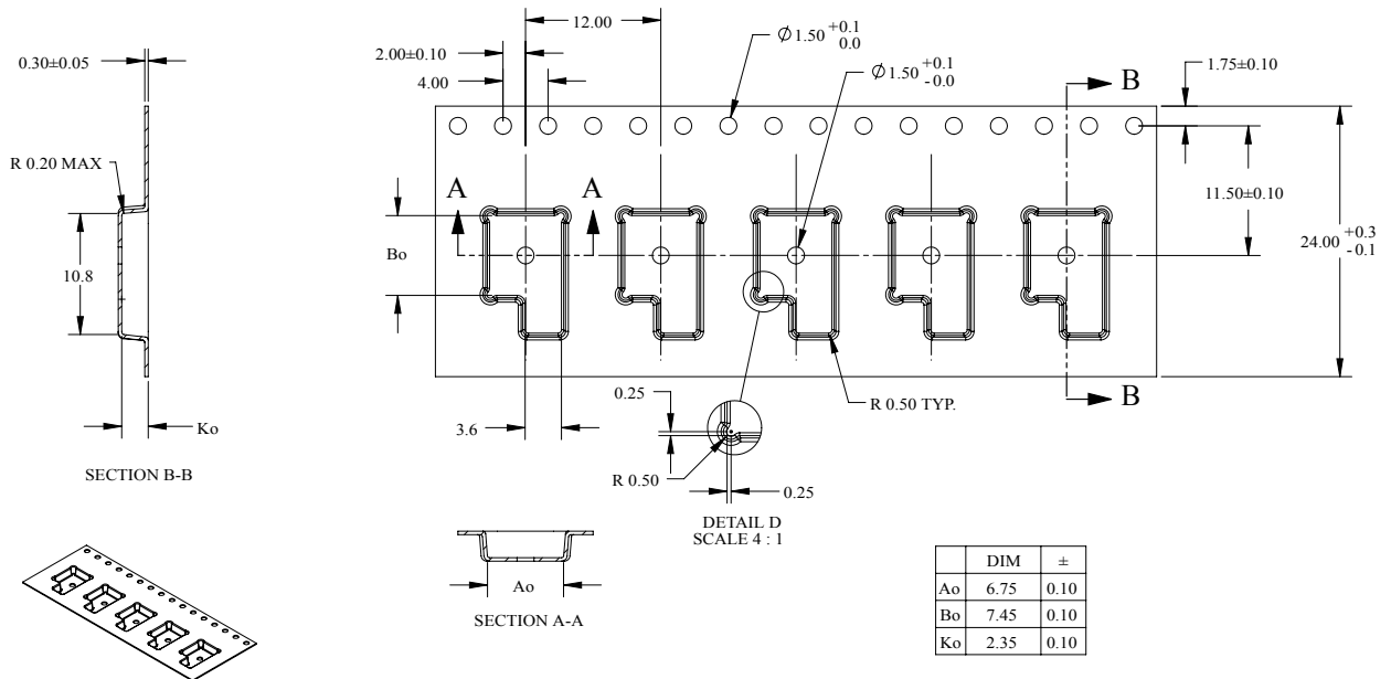
Figure 29. Reel description
