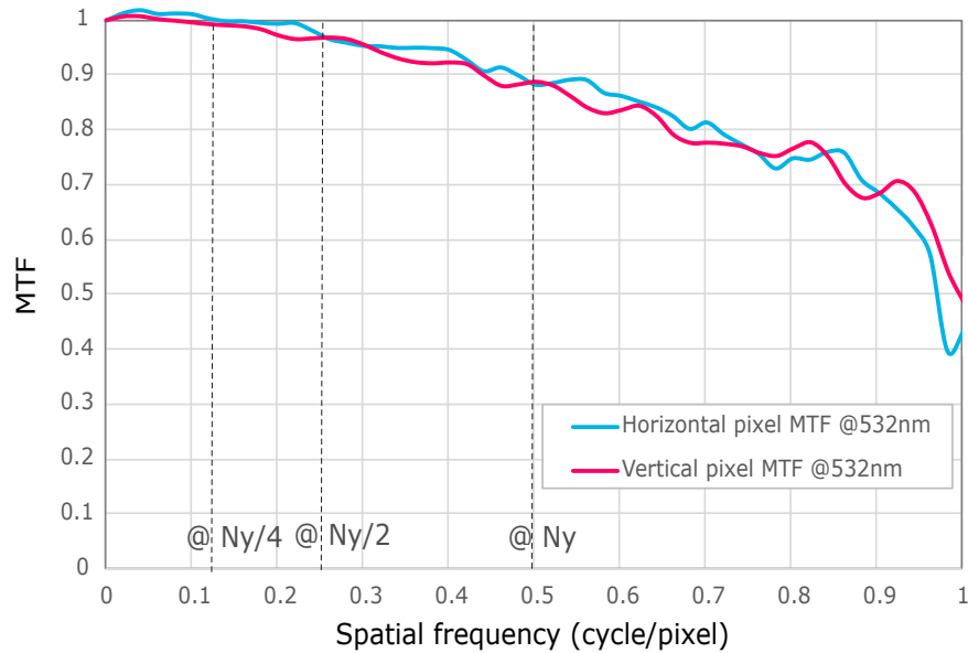
Figure 20. On-axis vertical and horizontal pixel MTF @ 532 nm
