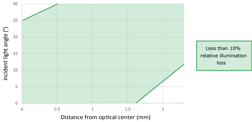
Figure 24. Co-centric pixel microlens CRA shift
