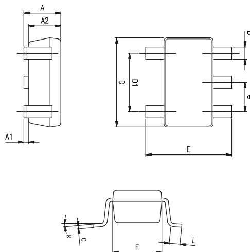
Figure 5. SOT23-5 package outline
