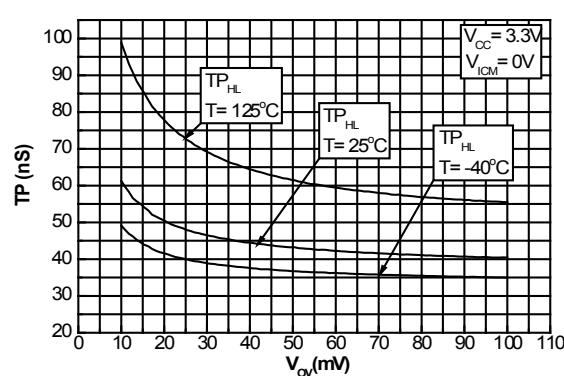
Figure 19. Propagation delay (HL) vs. overdrive at V_{cc} = 3.3V , V_{cm} = 0V
