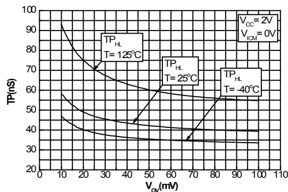
Figure 15. Propagation delay (HL) vs. overdrive at V_{cc} = 2V , V_{cm} = 0V
