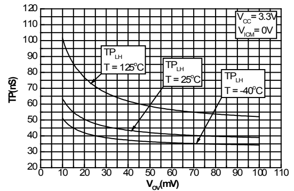
Figure 21. Propagation delay (LH) vs. overdrive at V_{CC} = 3.3\text{ V} , V_{ICM} = 0\text{ V}
