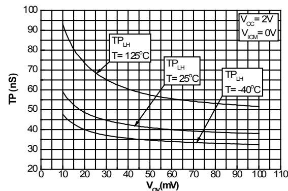
Figure 17. Propagation delay (LH) vs. overdrive at V_{cc} = 2V , V_{cm} = 0V
