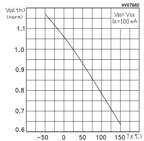
Figure 10. Normalized gate threshold vs temperature
