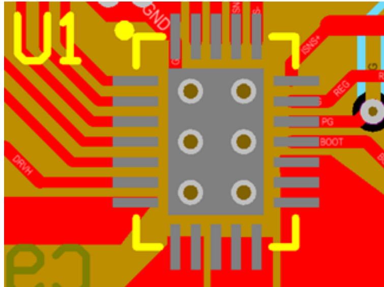
Figure 44. Thermal aspects
