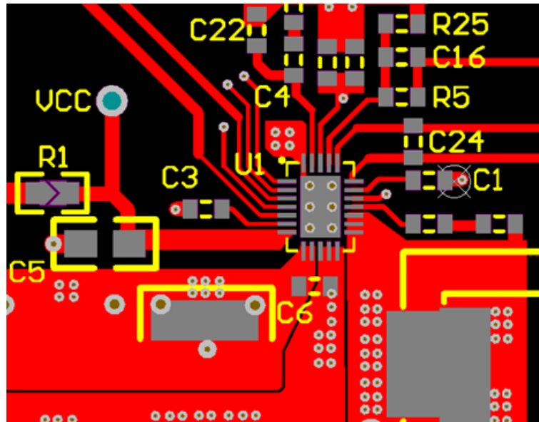
Figure 41. Capacitor placing
