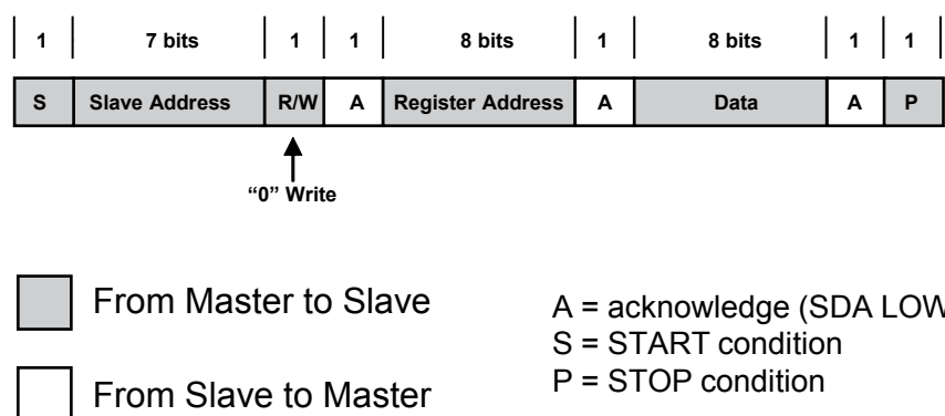
Figure 39. Write command
