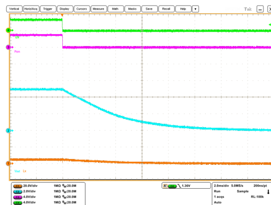
Figure 29. Enable shutdown ( V_{in} = V_{CC} = 24\text{ V} , V_{out} = 0\text{x64} (5 V), no load)
