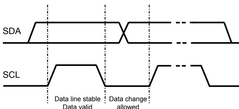
Figure 37. Data transfer validity
