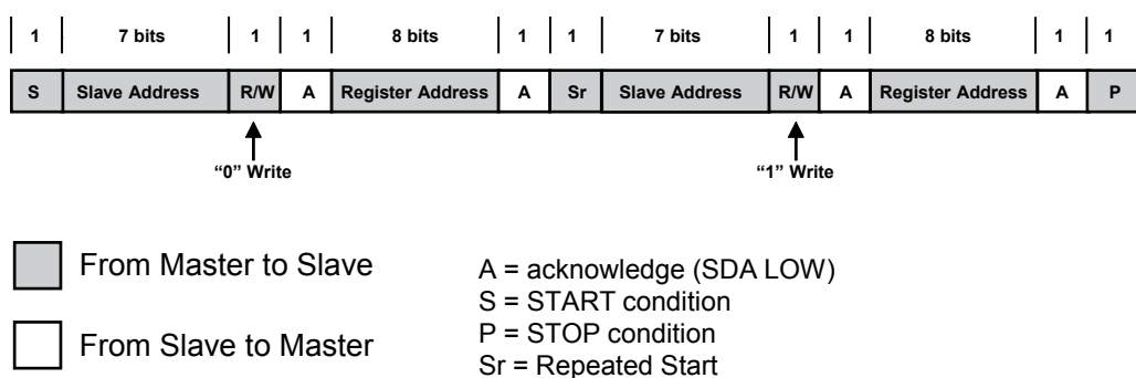
Figure 40. Read command
