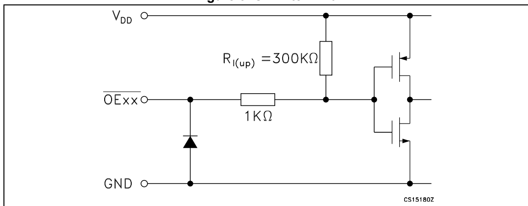
Figure 4. LE\DM terminal
