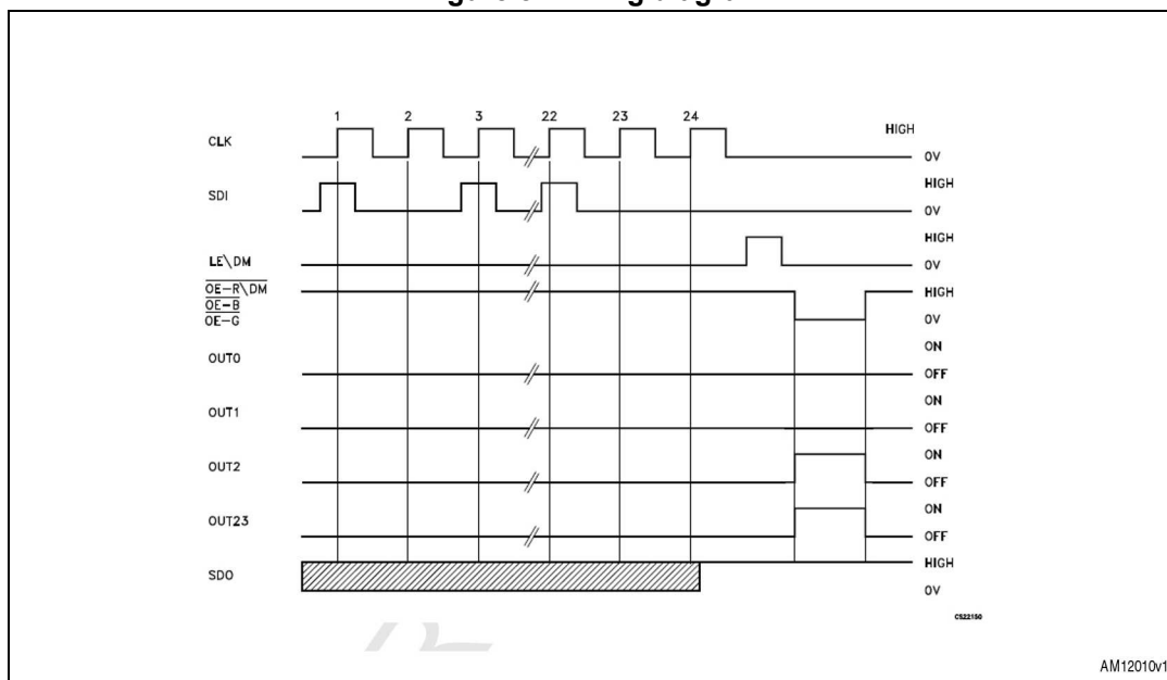
Figure 8. Timing diagram
