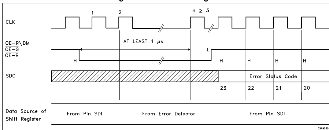
Figure 15. Detection diagram
