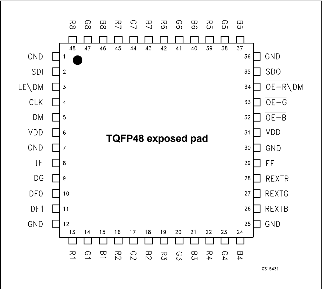
Figure 1. Pin connection
