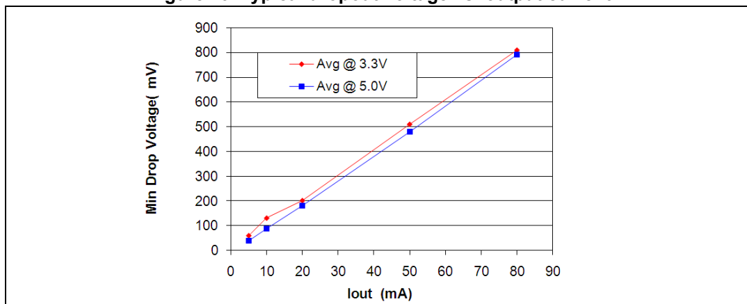
Figure 19. Typical dropout voltage vs. output current
