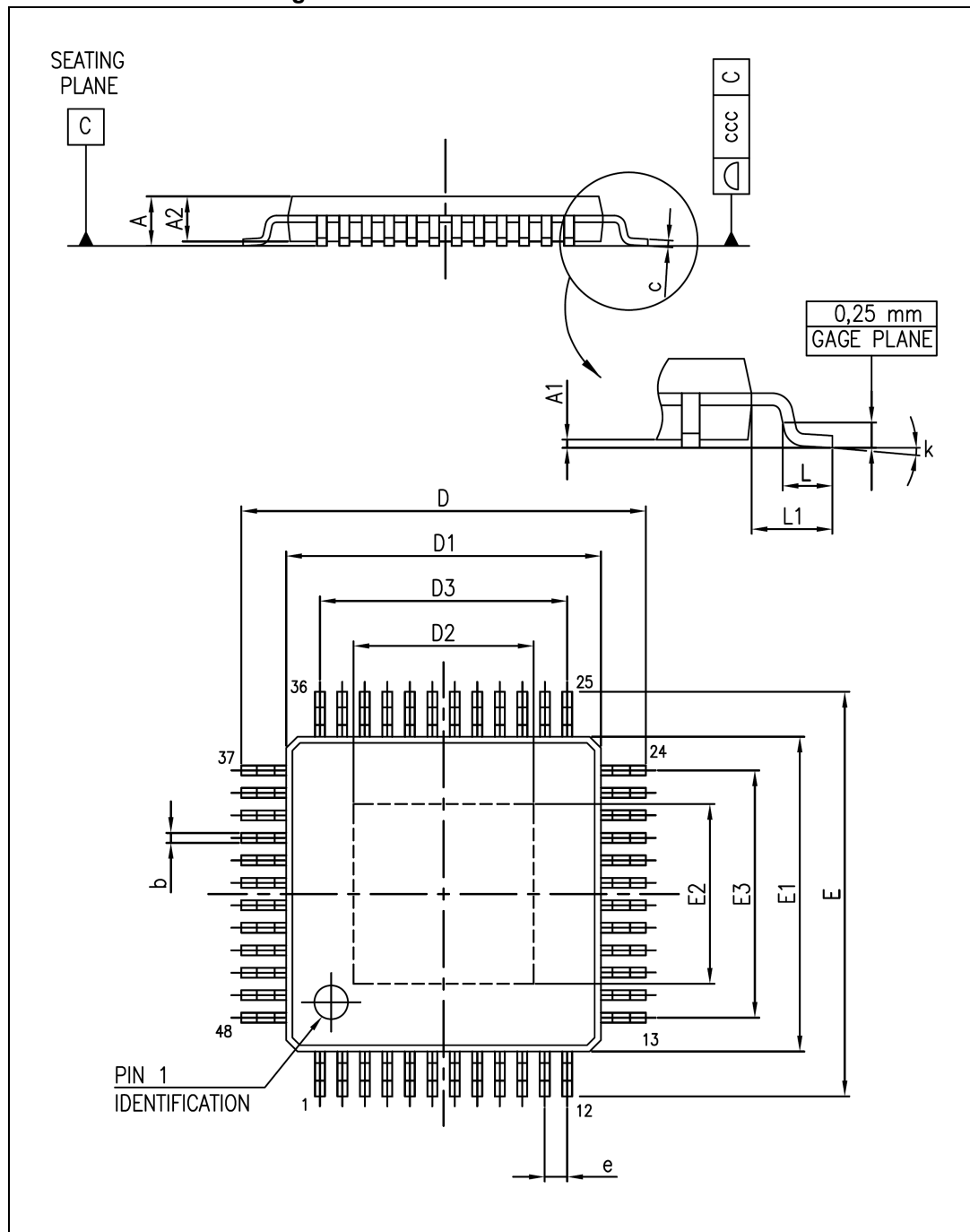
Figure 20. TQFP48-EP mechanical data
