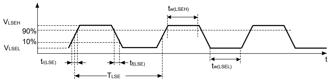
Figure 14. Low-speed external clocksource AC timing diagram
