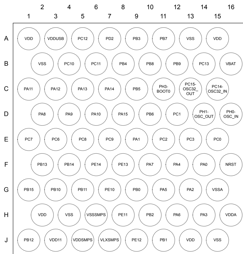
Figure 12. WLCSP72_SMPS ballout
