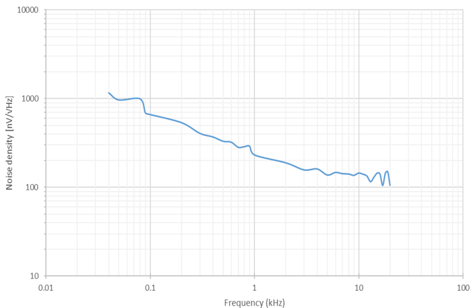
Figure 46. OPAMP voltage noise density, low-power mode, R_{LOAD} = 20\text{ k}\Omega
