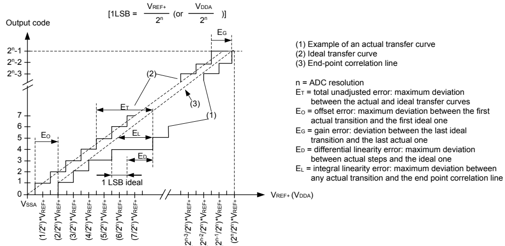
Figure 38. ADC accuracy characteristics
