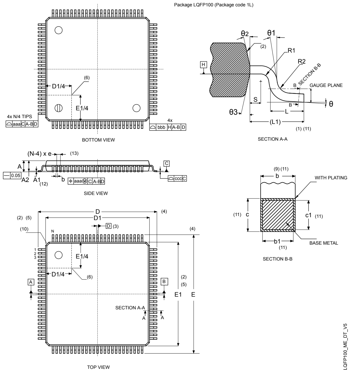
Figure 75. LQFP100 - Outline (15)
