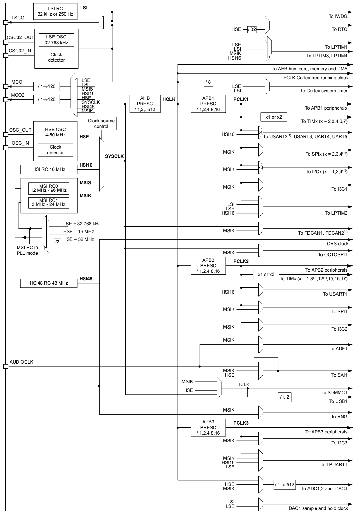
Figure 5. Clock tree
