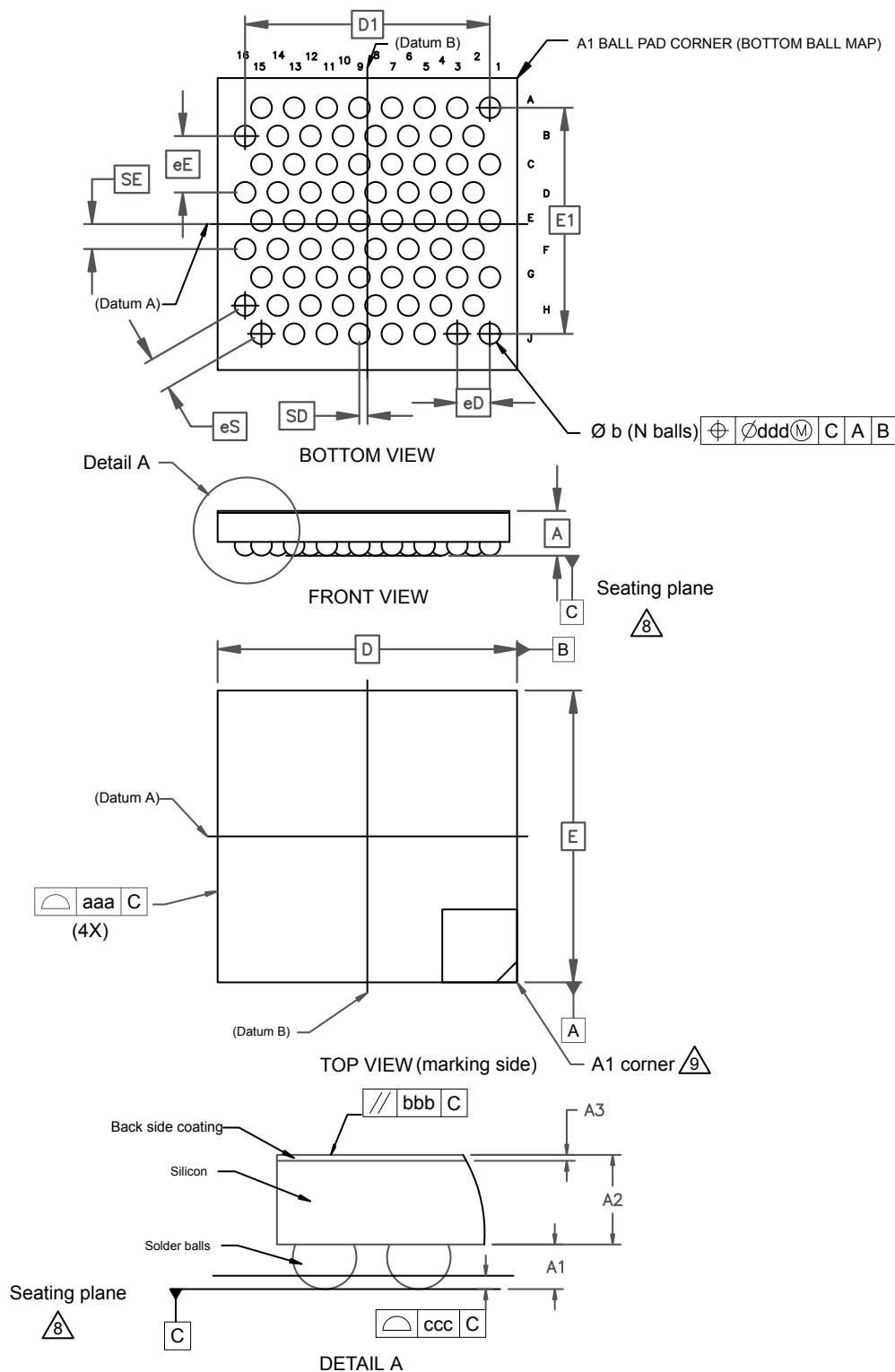
Figure 71. WLCSP72 - Outline
