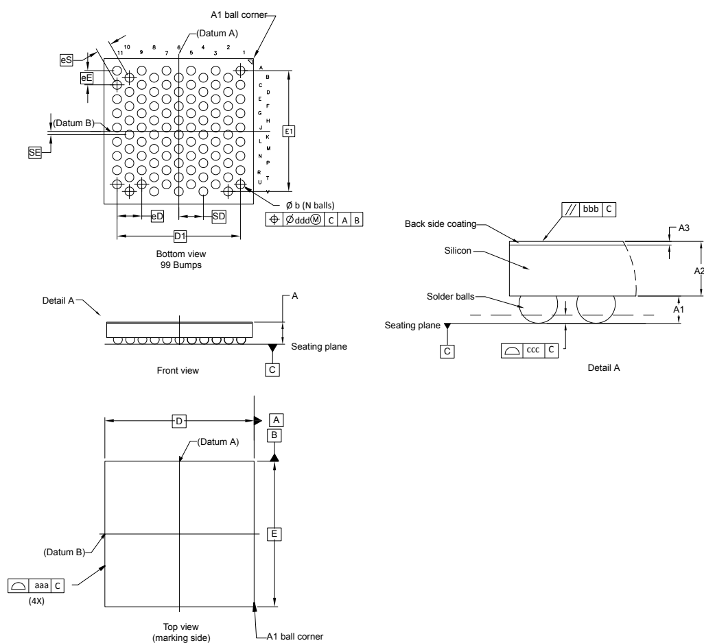
Figure 73. WLCSP99 - Outline
