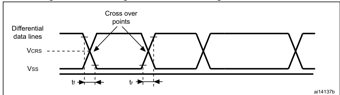
Figure 58. USB timings - definition of data signal rise and fall time
