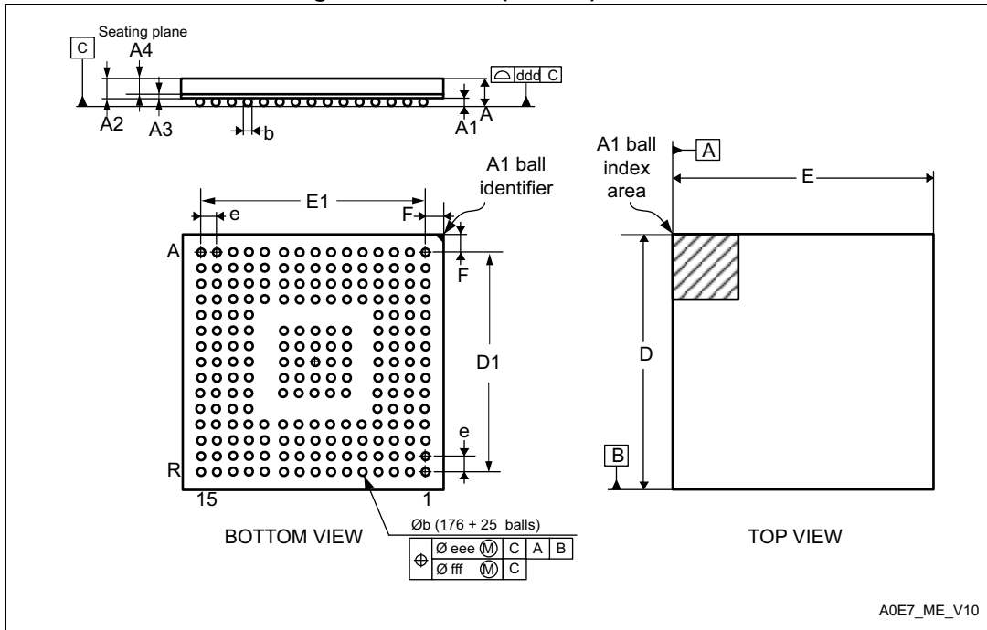
Figure 91. UFBGA(176+25) - Outline
