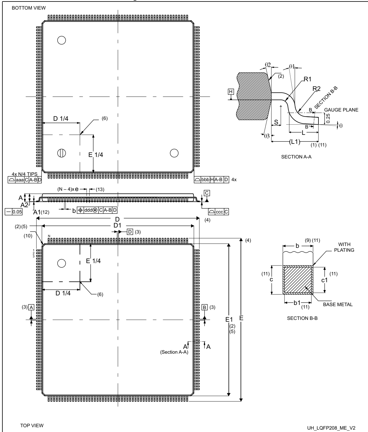
Figure 87. LQFP208 - Outline (15)
