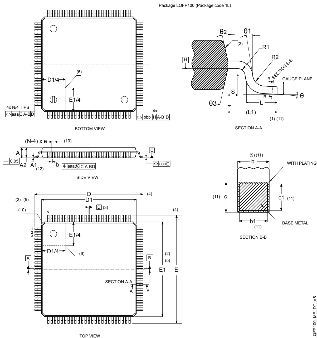
Figure 56. LQFP100 - Outline (15.)
