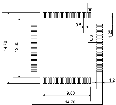
Figure 55. LQFP80 - Footprint example
