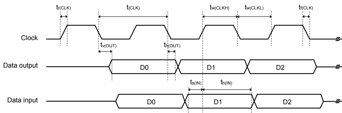
Figure 23. OCTOSPI SDR read/write timing diagram
