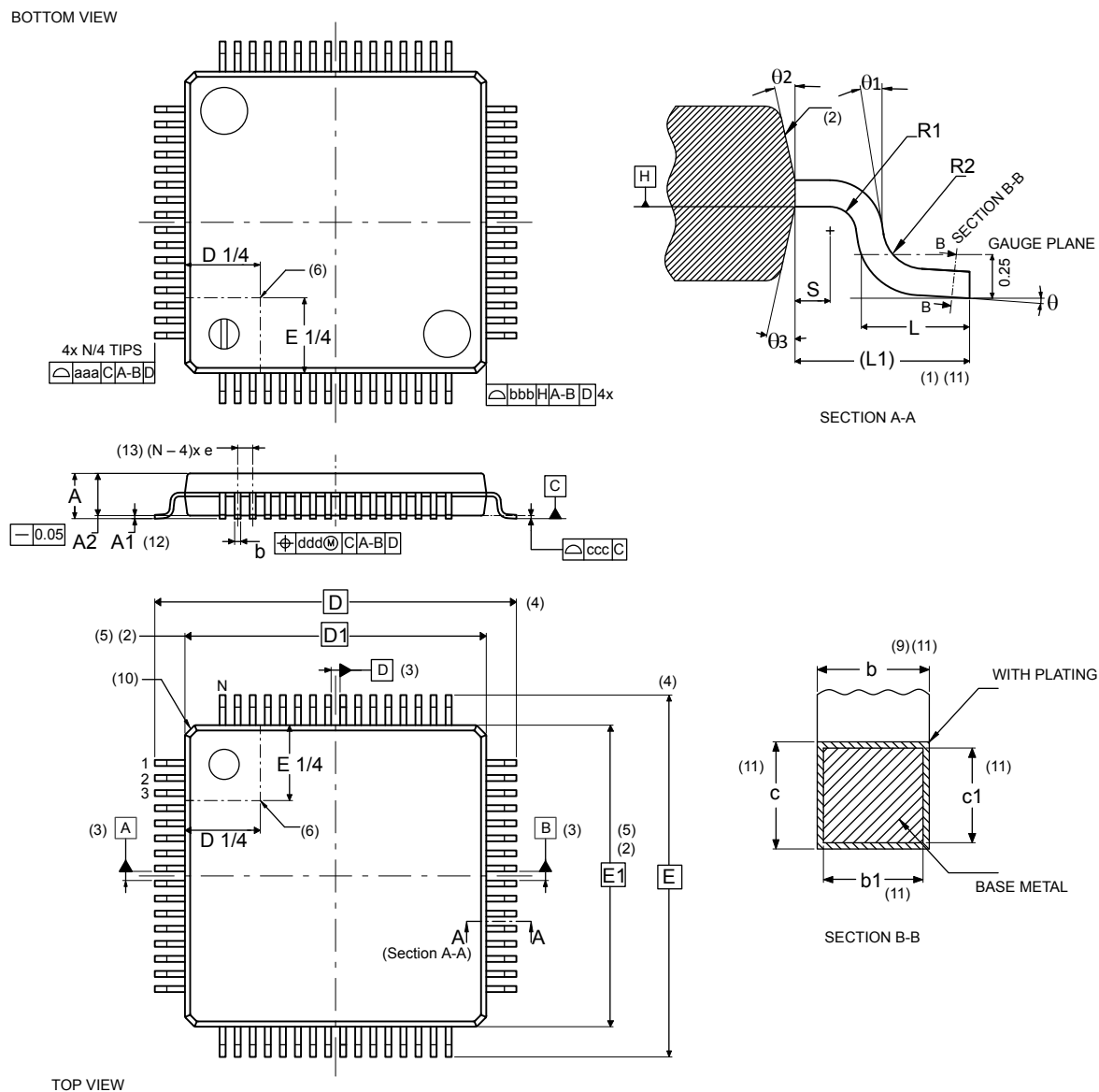
Figure 53. LQFP64 - Outline (15.)
