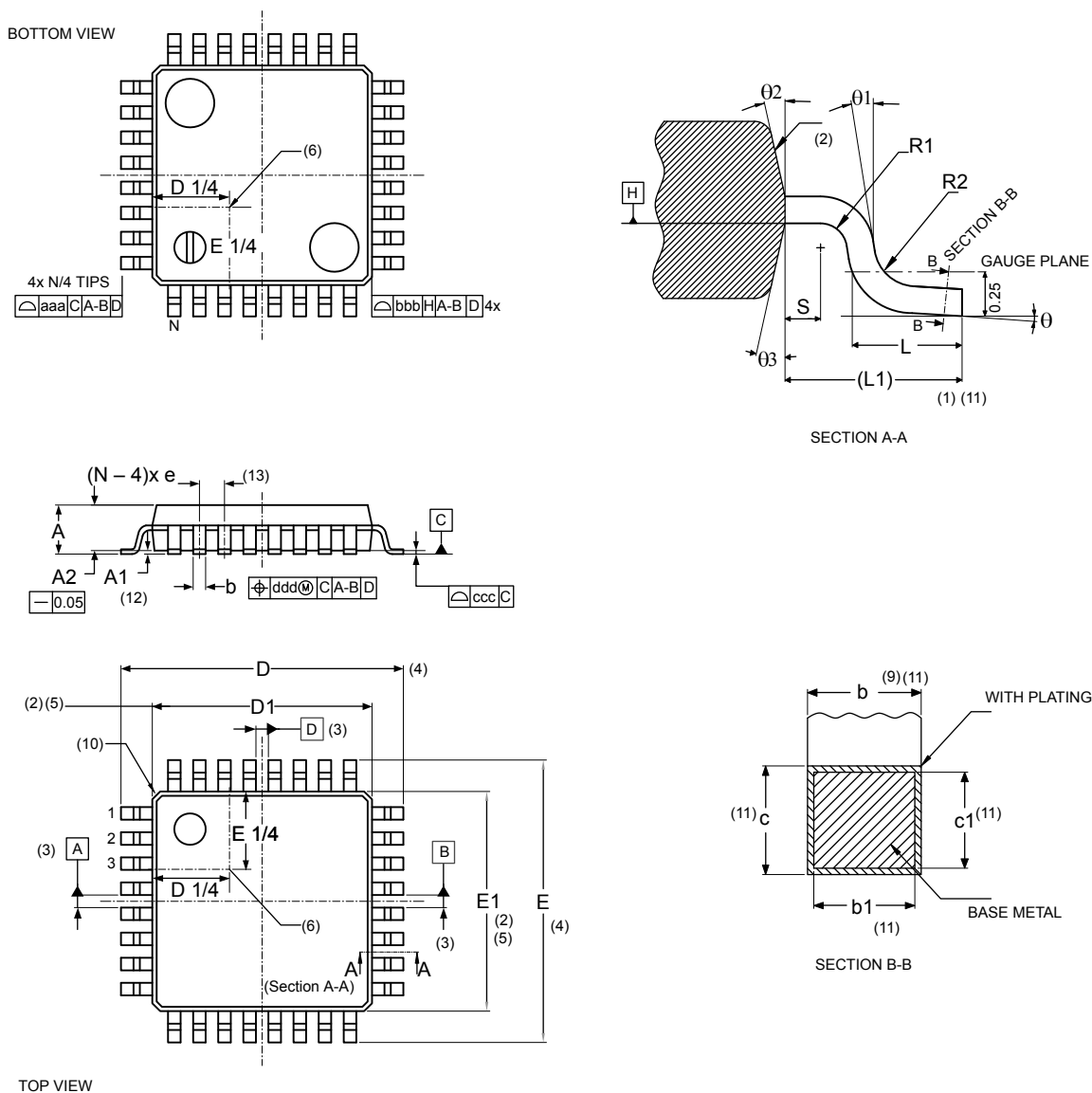
Figure 45. LQFP32- Outline
