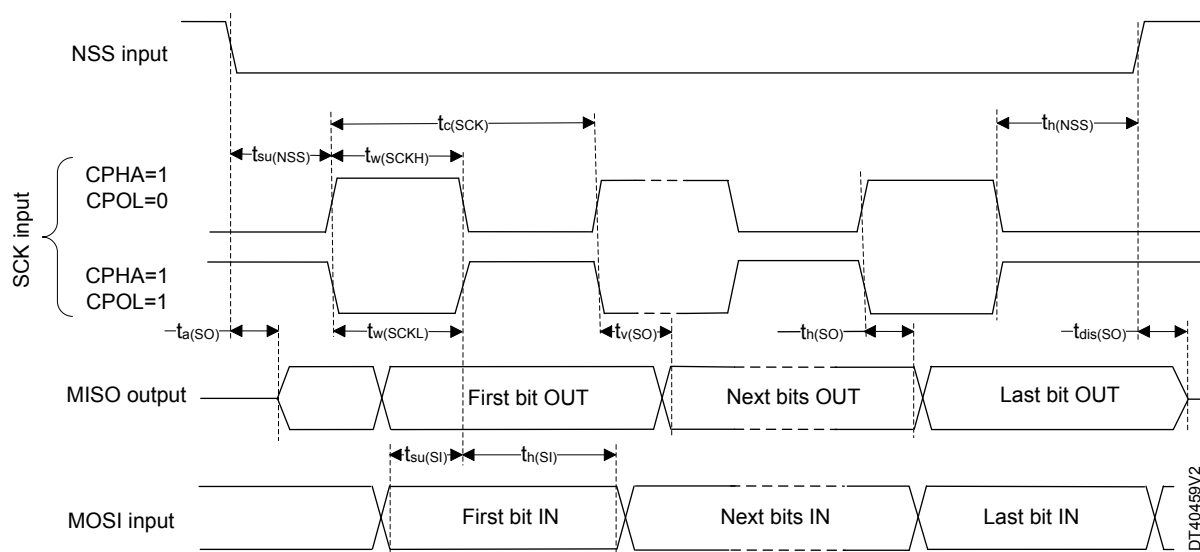
Figure 38. SPI timing diagram - slave mode and CPHA = 1
