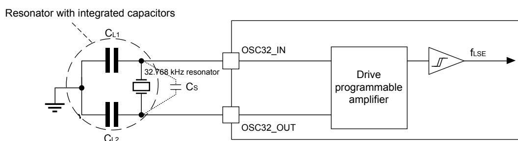
Figure 18. Typical application with a 32.768 kHz crystal
