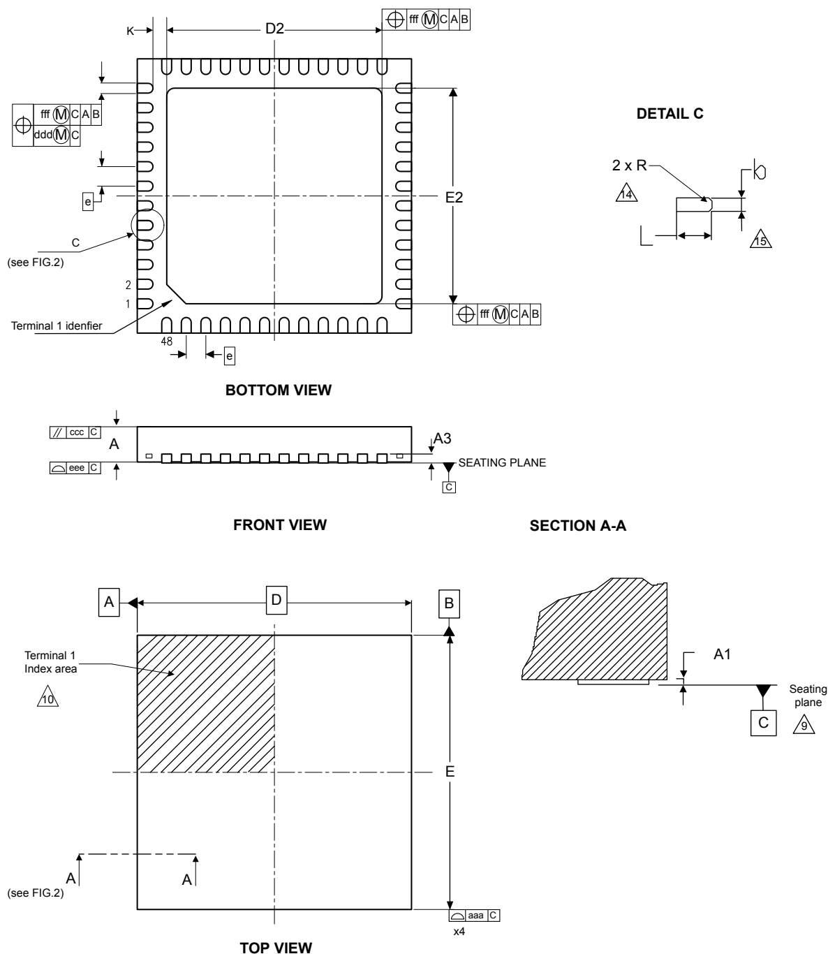
Figure 51. UFQFPN48 - Outline
