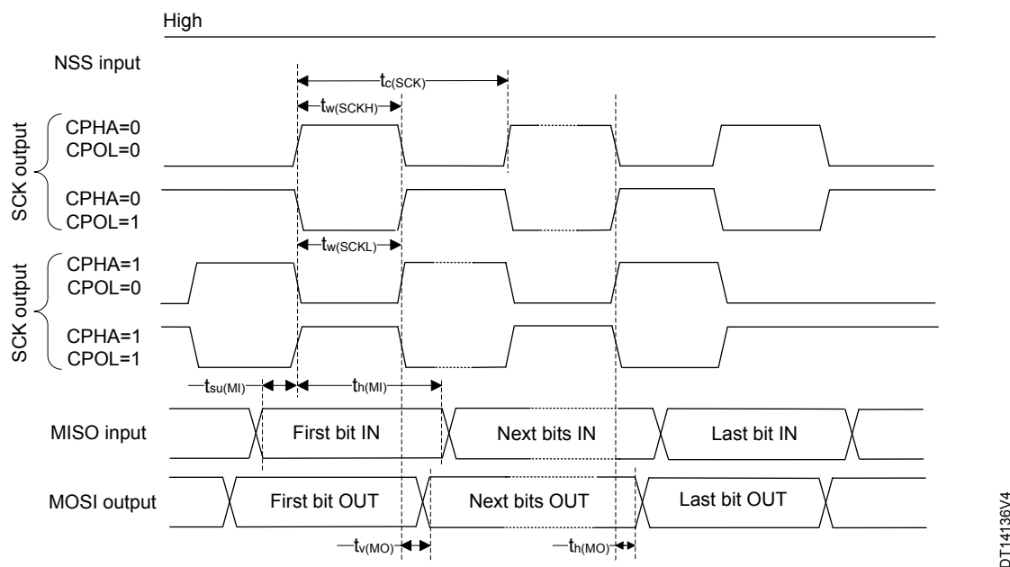
Figure 39. SPI timing diagram - master mode
