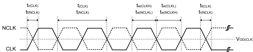
Figure 25. OCTOSPI Hyperbus clock
