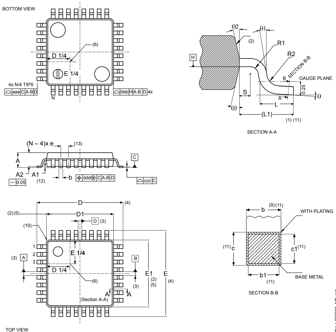
Figure 43. LQFP32- Outline
