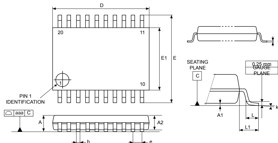
Figure 37. TSSOP20 - Outline
