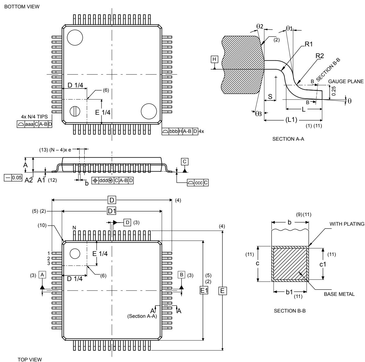
Figure 51. LQFP64 - Outline (15.)
