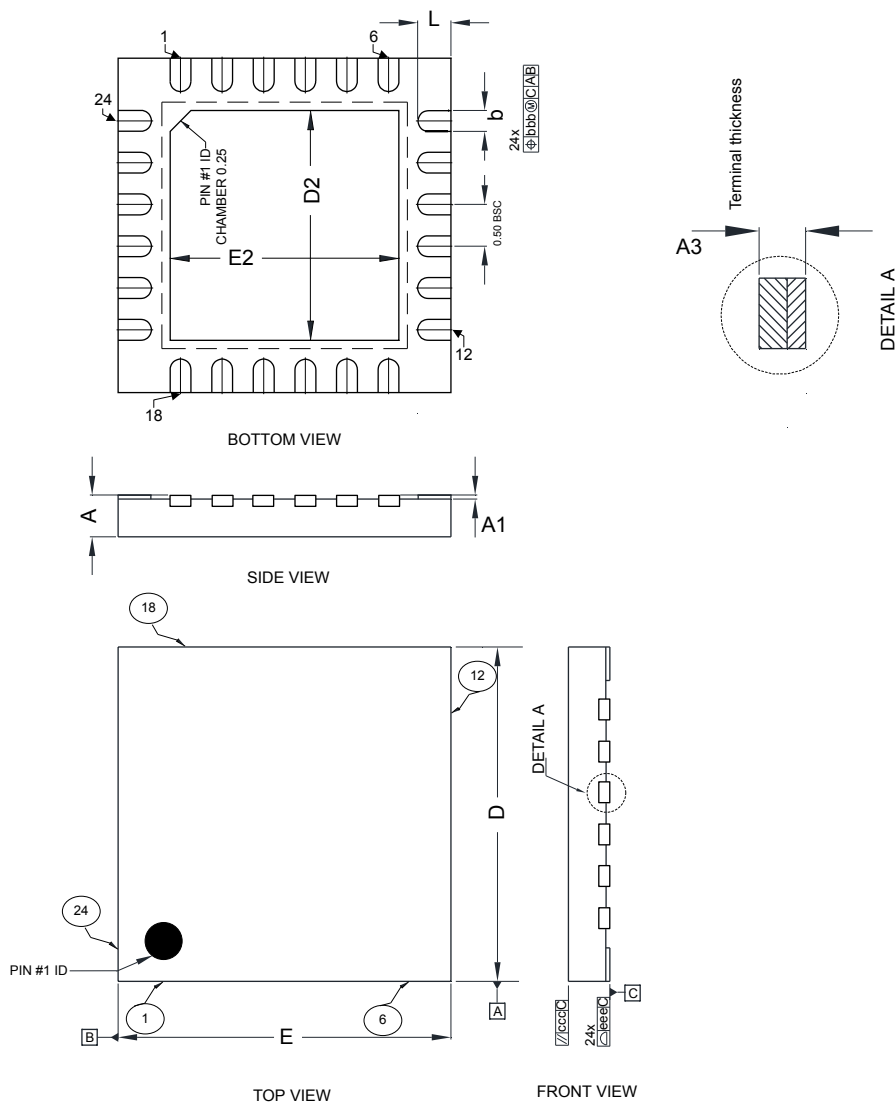
Figure 41. UFQFPN24 - Outline
