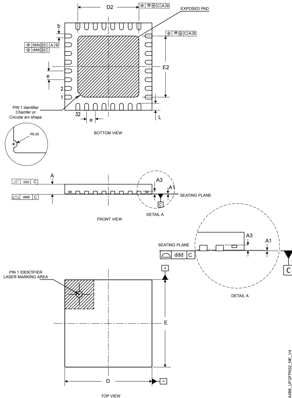
Figure 45. UFQFPN32 - Outline
