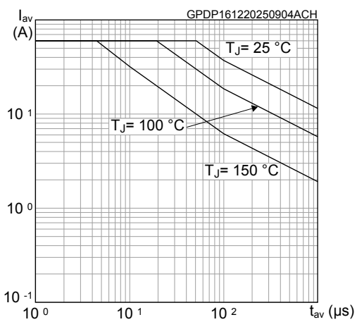
Figure 9. Avalanche characteristics
