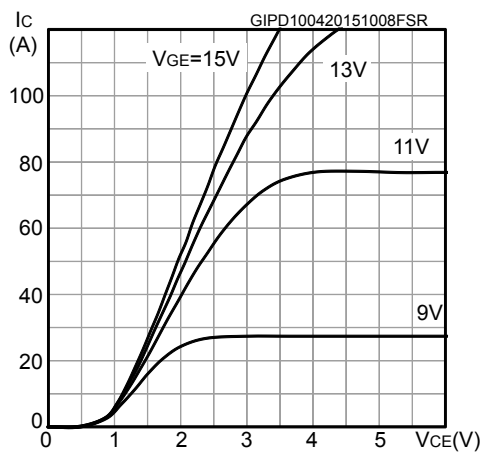
Figure 3. Typical output characteristics ( T_J = 25^\circ\text{C} )
