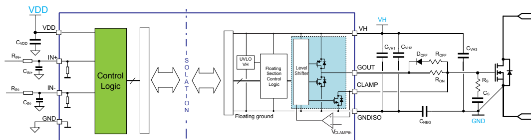
Figure 8. STGAP2SA reference schematic for suggested PCB layout
