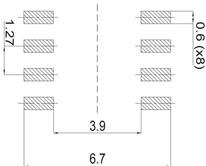
Figure 12. SO-8 suggested land pattern
