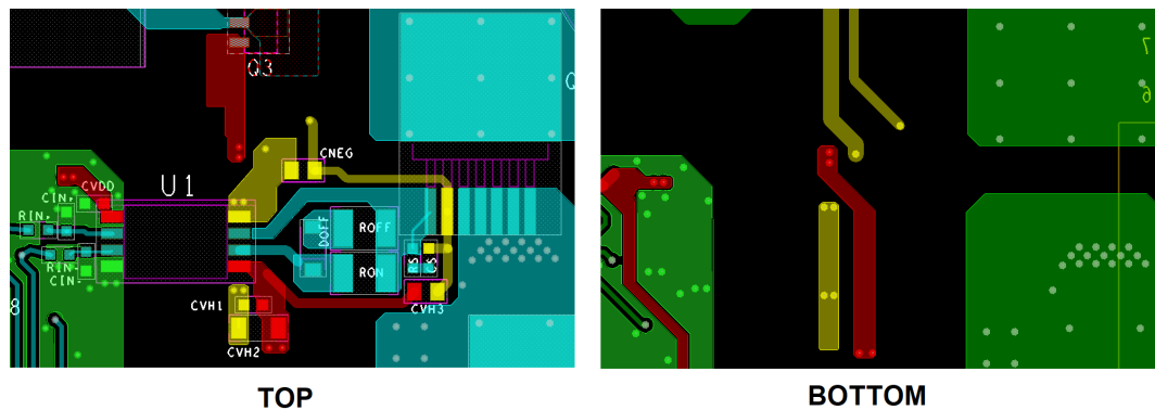
Figure 7. STGAP2SA suggested PCB layout: top and bottom
