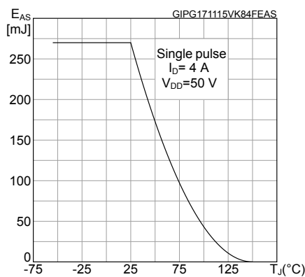
Figure 11. Maximum avalanche energy vs starting T_J
