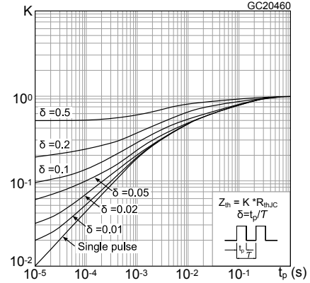
Figure 2. Thermal impedance
