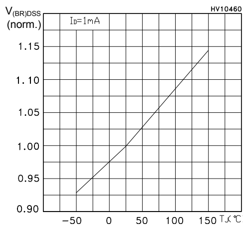
Figure 14. Normalized breakdown voltage vs temperature
