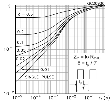
Figure 2. Thermal impedance
