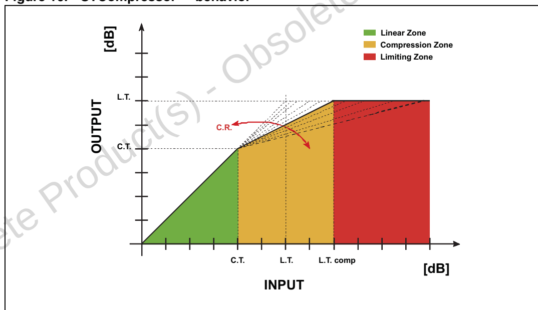
Figure 10. STCompressor™ behavior
