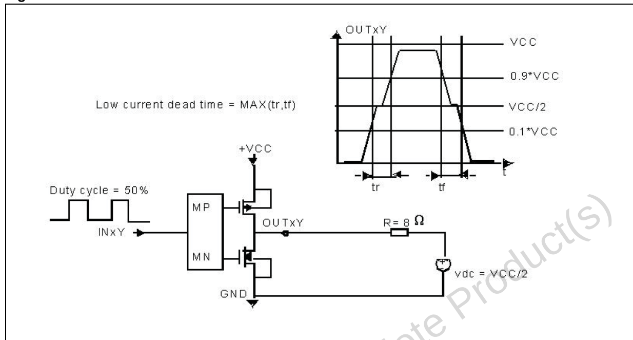
Figure 3. Test circuit
