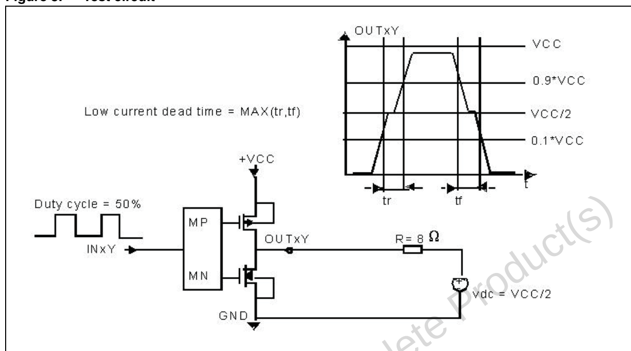
Figure 3. Test circuit
