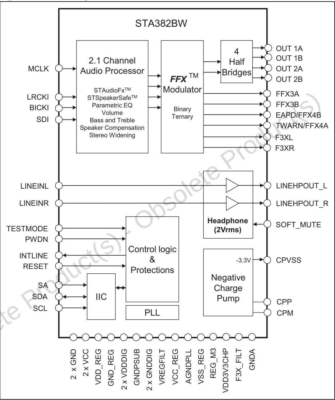
Figure 1. Block diagram
