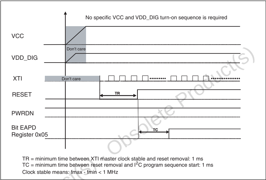
Figure 3. Power-on sequence
