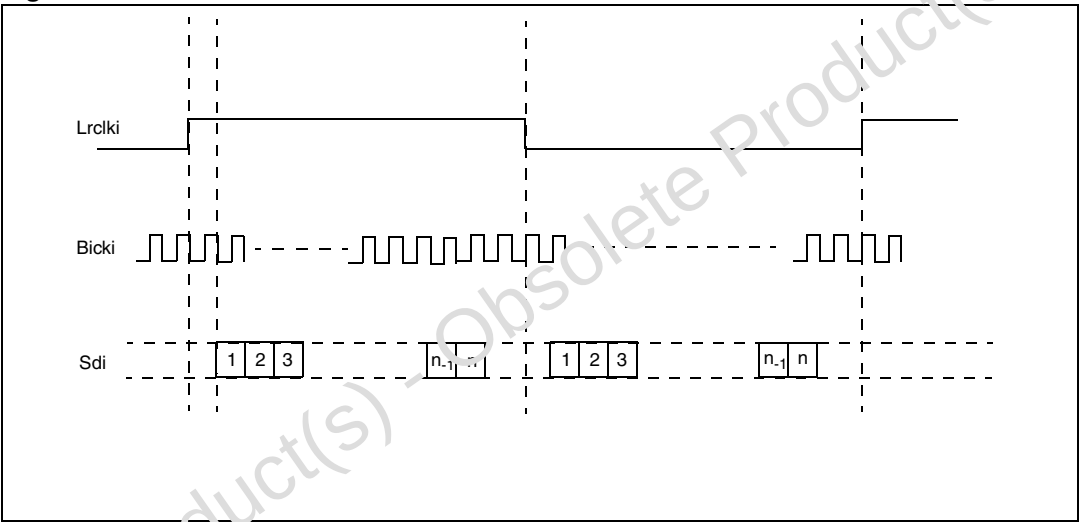
Figure 8. I 2 S
