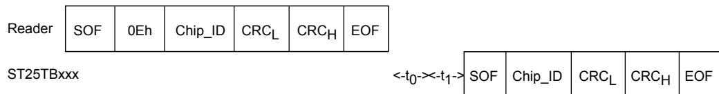
Figure 48. Select frame exchange between reader and ST25TB512-AT
