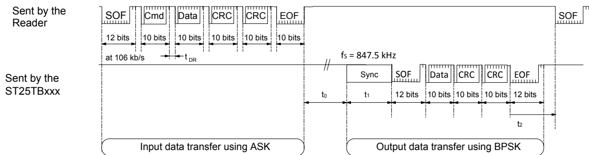
Figure 10. Example of a complete transmission frame
