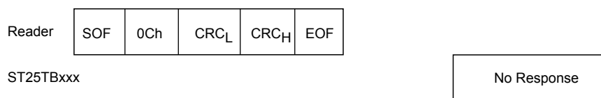
Figure 33. Reset_to_inventory frame exchange between reader and ST25TB512-AT
