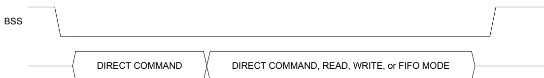
Figure 13. SPI communication: direct command chaining
