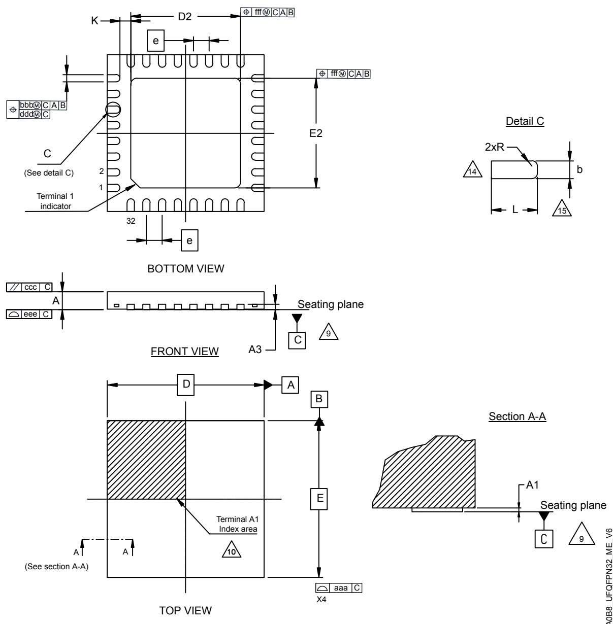
Figure 19. UFQFPN32 - Outline
