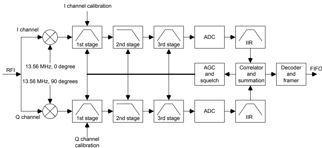
Figure 5. Receiver block diagram
