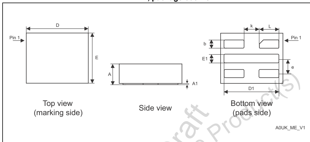
Figure 15. UFDFPN5 - 5-lead ultra thin fine pitch dual flat package, no lead, 1.7x1.4 mm, package outline
