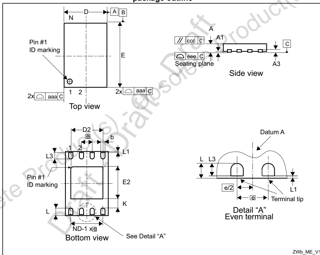
Figure 14. UFDFPN8 - 8-lead 2 x 3 mm, 0.5 mm ultra thin profile fine pitch dual flat package outline
