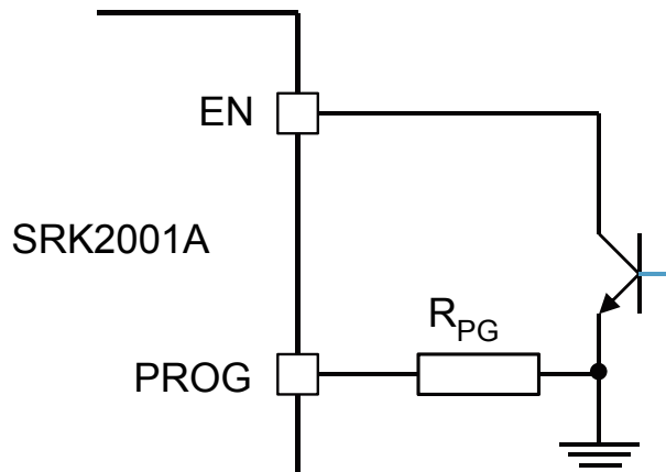
Figure 9. EN - PROG pin configurations
