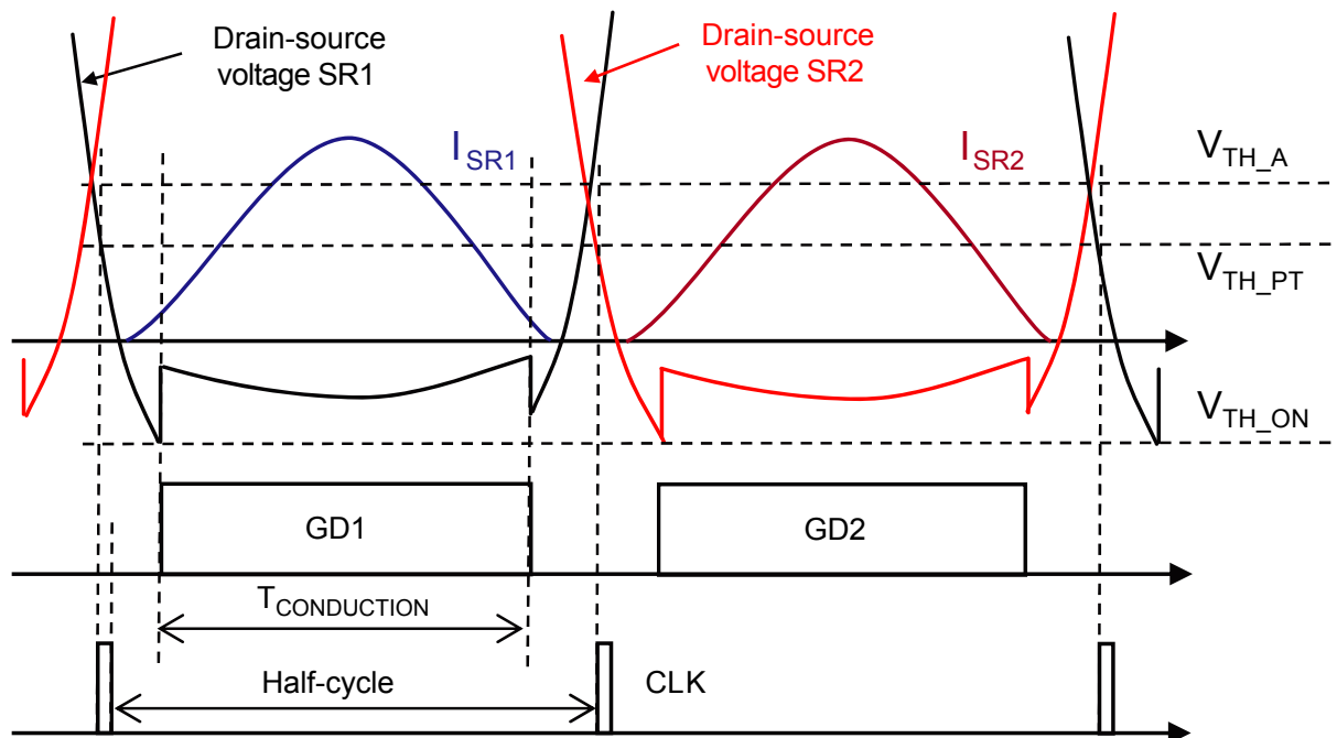
Figure 5. Typical waveforms
