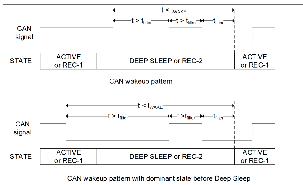
Figure 35. CAN wake-up capabilities
