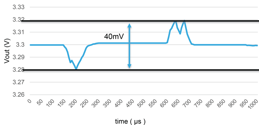
Figure 53. Buck1&2 @ 2.4 MHz
