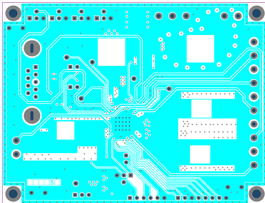
Figure 77. SPSB100GS 6-Layer Demo Board – Layer 5
