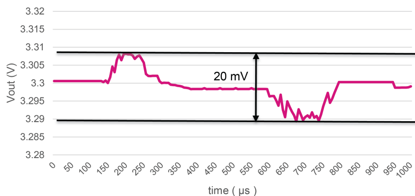
Figure 55. Buck1&2 @ 400 kHz
