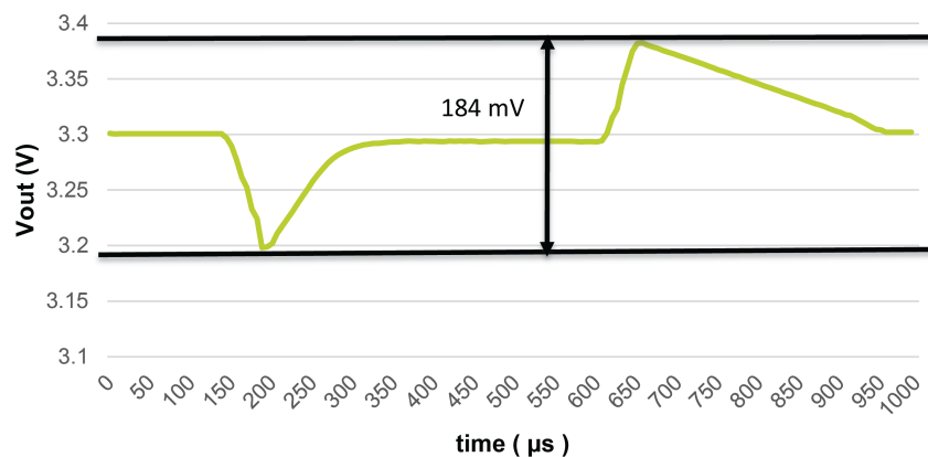
Figure 52. Buck1&2 @ 400 kHz
