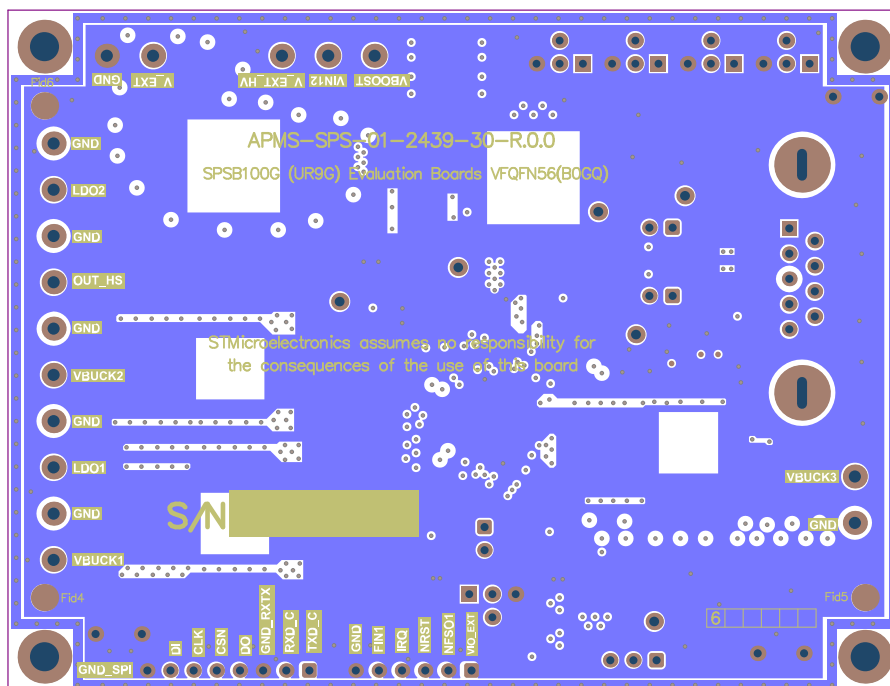
Figure 78. SPSB100GS 6-Layer Demo Board – Bottom Layer
