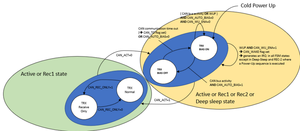
Figure 34. Transceiver state diagram
