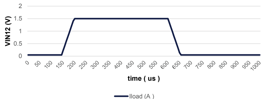
Figure 52. Buck1&2 @ 400 kHz
