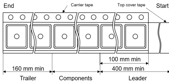
Figure 21. Tape leader and trailer dimensions
