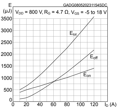
Figure 10. Typical switching energy vs drain current
