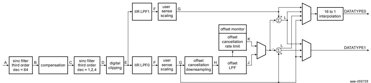
Figure 8. Acceleration signal processing flow
