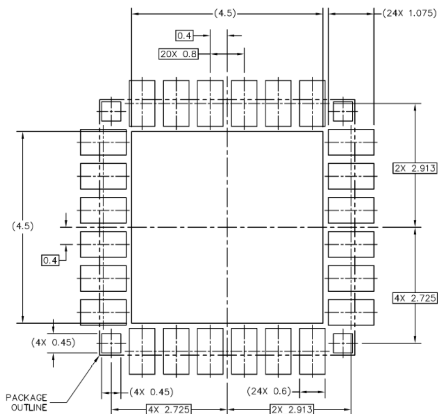
H-PQFN-24 I/O 0.1 DIMPLE WETTABLE FLANK 6 X 6 X 1.9 PKG, 0.8 PITCH
