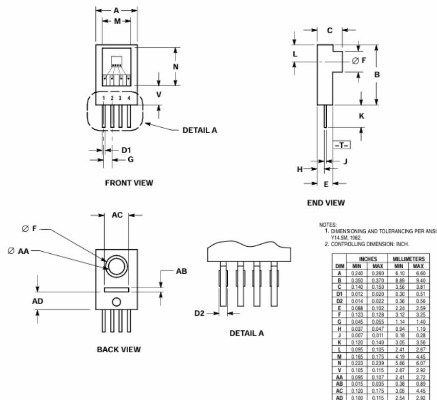
Figure 3. Case 98ASB1335C, Chip Pak package
