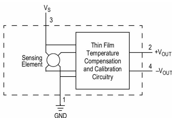
Figure 1. Block diagram
