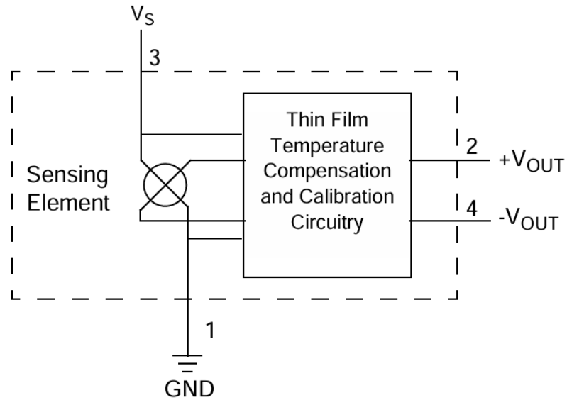
Figure 1. Temperature Compensated Pressure Sensor Schematic
