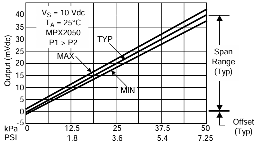
Figure 3. Output versus Pressure Differential
