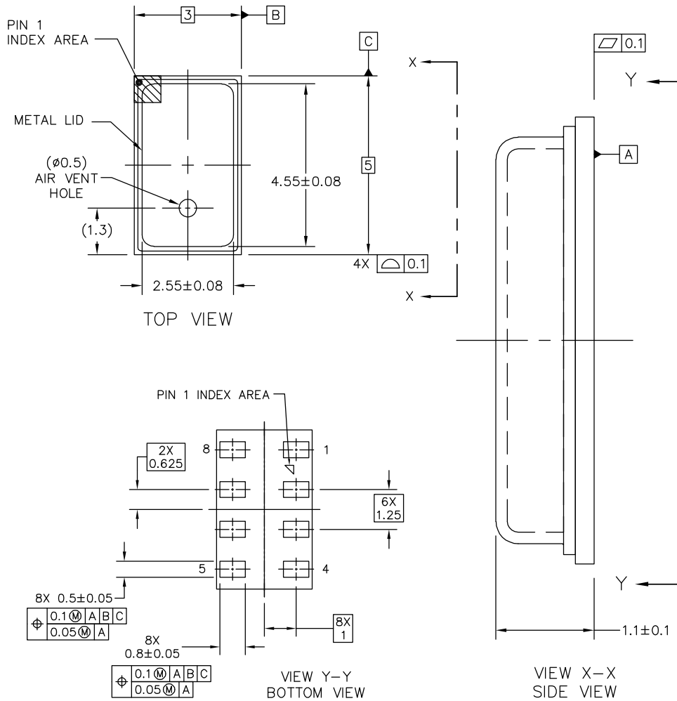
Figure 9. LGA package
