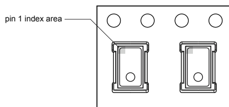
Figure 13. Device orientation in chip carrier
