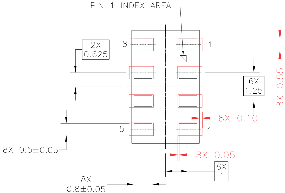
Figure 11. Recommended PCB landing pattern
