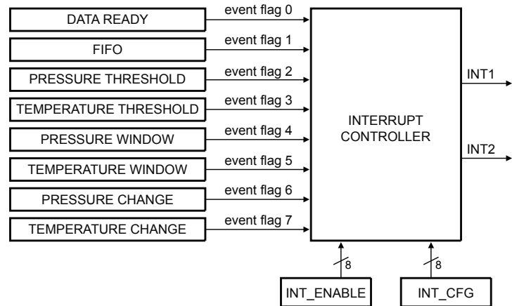
Figure 7. Interrupt controller block diagram
