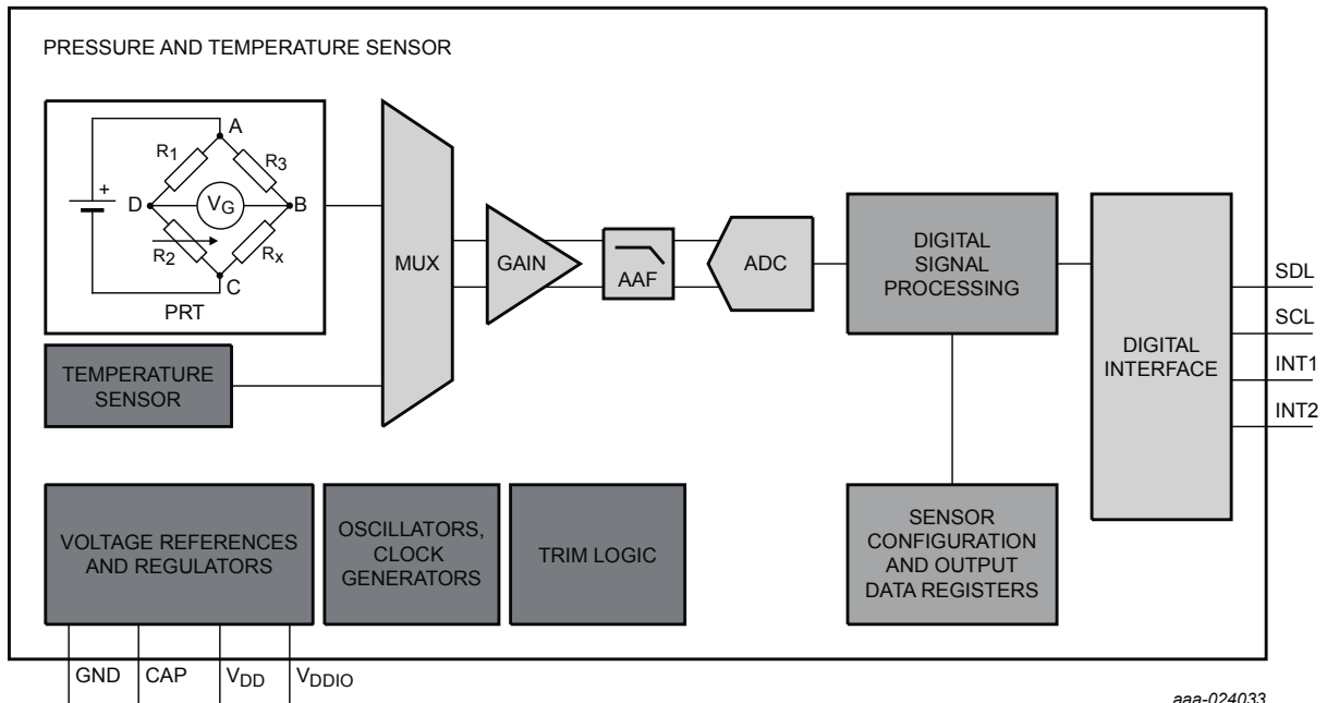
Figure 1. Block diagram
