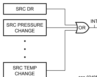
Figure 8. INT1/INT2 pin control logic
