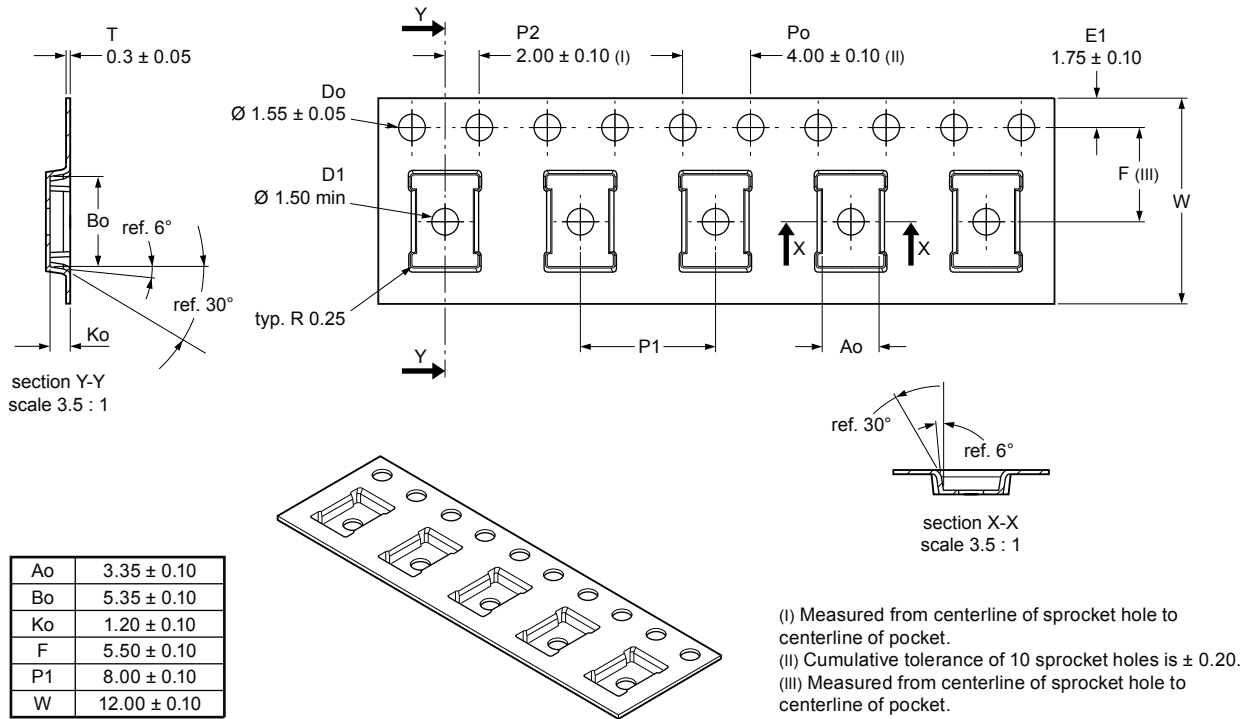
Figure 12. LGA 3 mm × 5 mm embossed carrier tape dimensions
