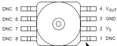
MP3V5050V Case 98ASB17757C
