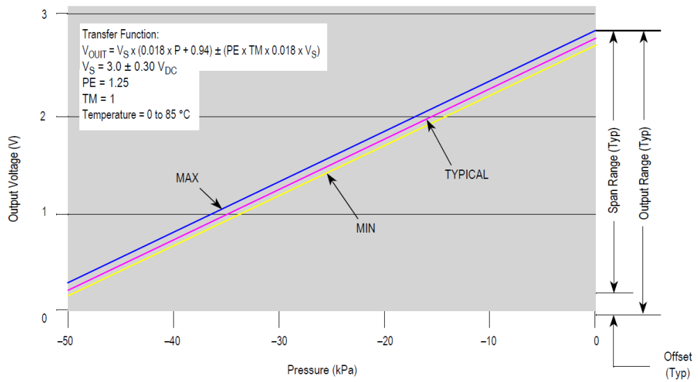
Figure 6. Transfer function
