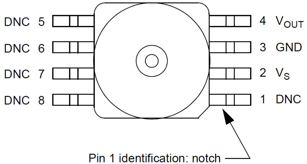
Figure 2. Device pinout (top view)
