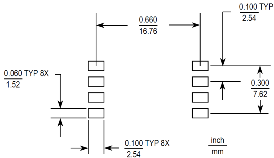
Figure 9. SOP footprint
