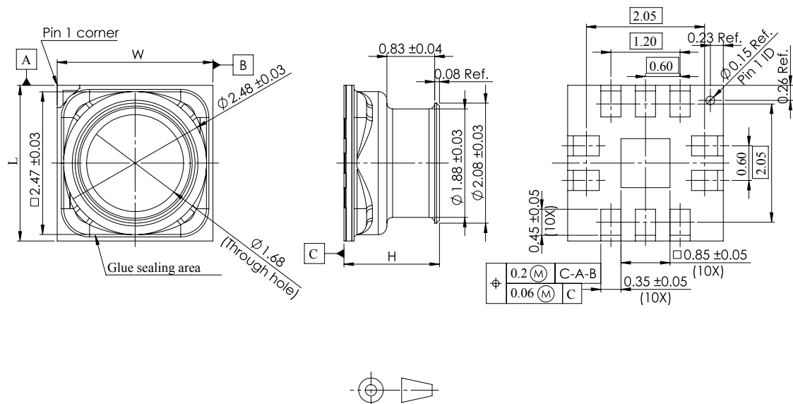
Figure 26. LGA-11L 2.7 x 2.7 x 1.85 mm package outline and mechanical data
