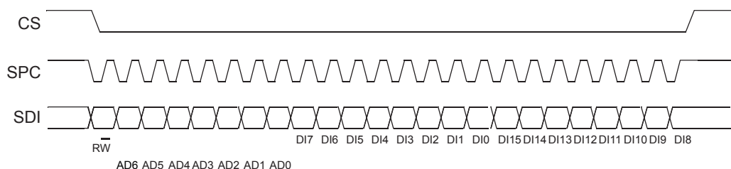
Figure 21. Multiple byte SPI write protocol (2-byte example)
