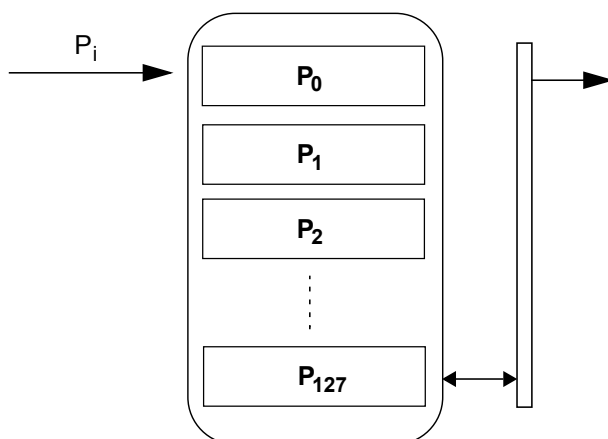
Figure 10. FIFO mode
