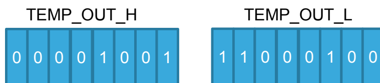
Figure 8. Temperature readings
