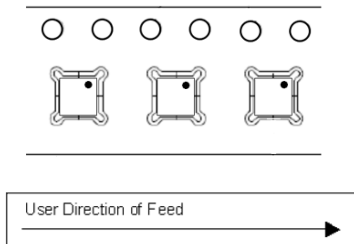
Figure 28. LGA-11L package orientation in carrier tape
