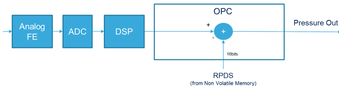
Figure 25. One-point calibration
