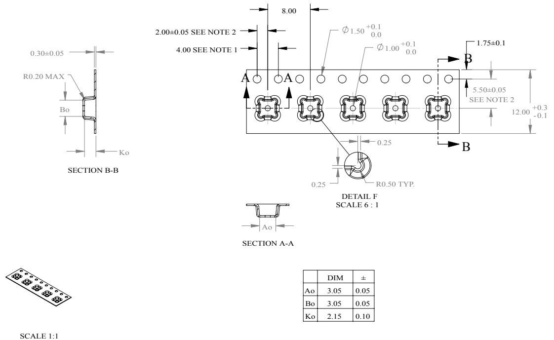
Figure 27. Carrier tape information for LGA-11L package
