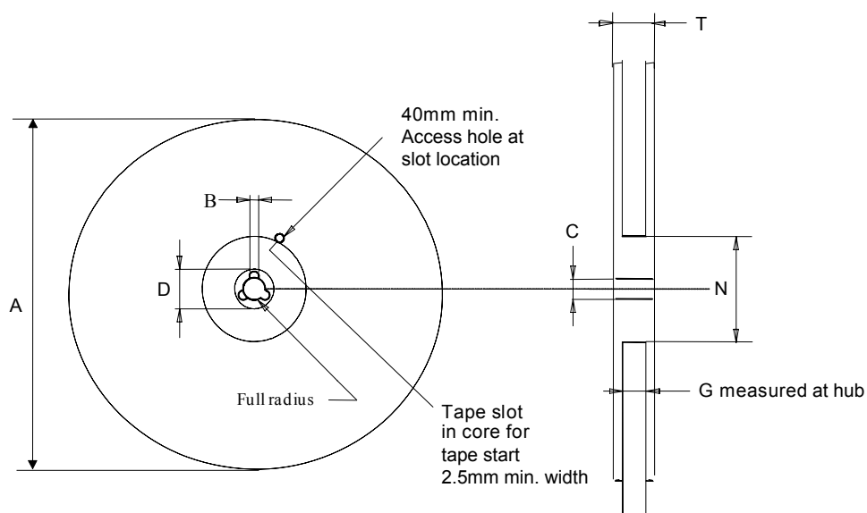
Figure 29. Reel information for carrier tape of LGA-11L package
