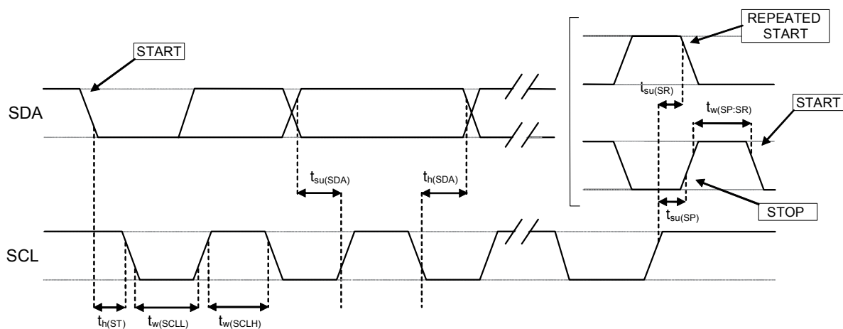
Figure 4. I 2 C target timing diagram
