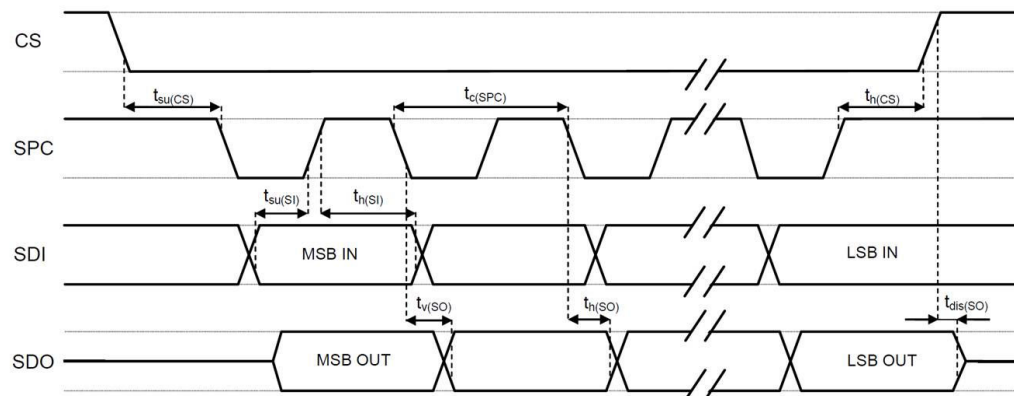
Figure 5. SPI target timing diagram
