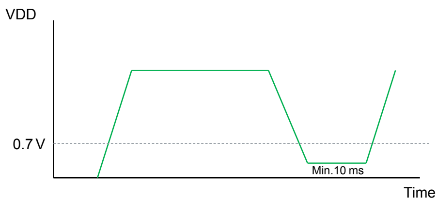
Figure 16. LPS27DEWO power-off sequence
