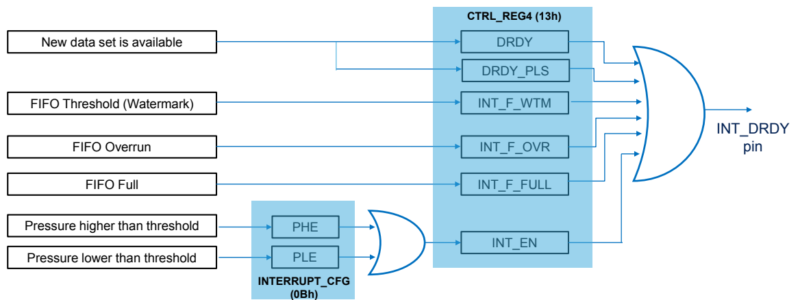
Figure 24. Interrupt events on INT_DRDY pin
