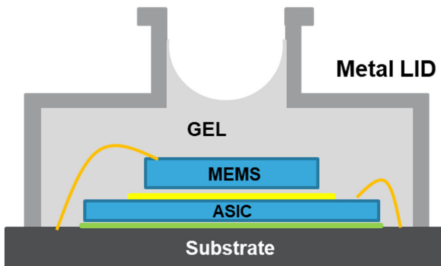
Figure 6. LPS27DEWO internal structure
