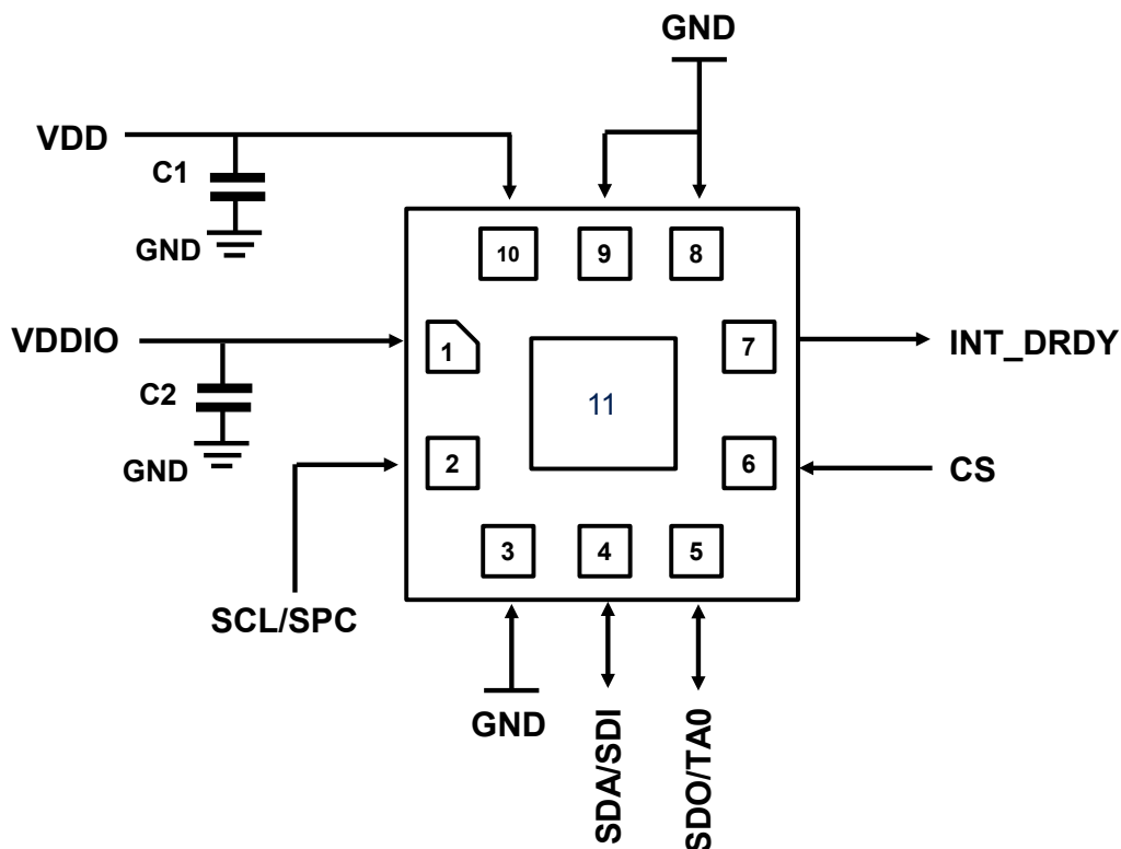
Figure 15. LPS27DEWO electrical connections (top view)
