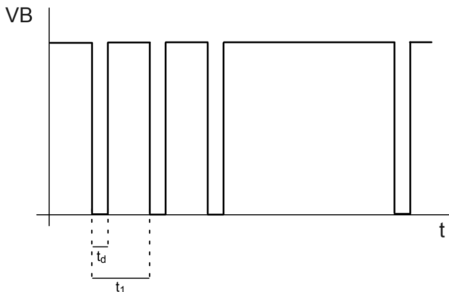
Figure 9. Micro-interruption
