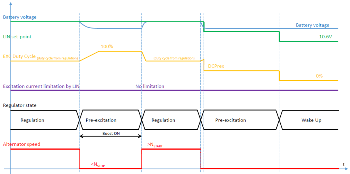
Figure 14. Pre-excitation specific mode: example 2
