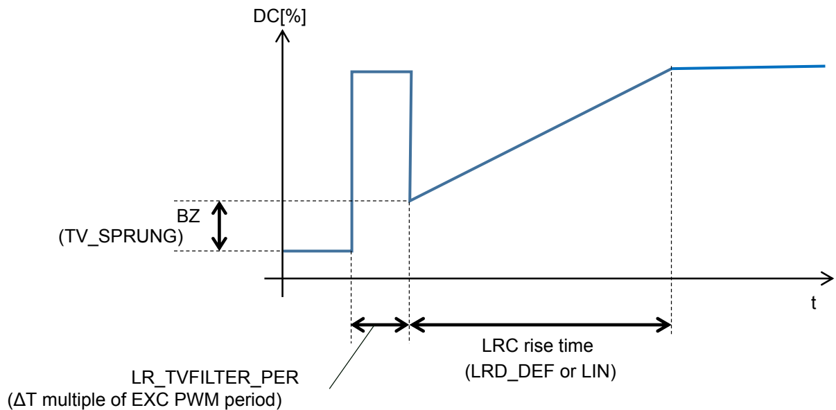
Figure 12. Load response control
