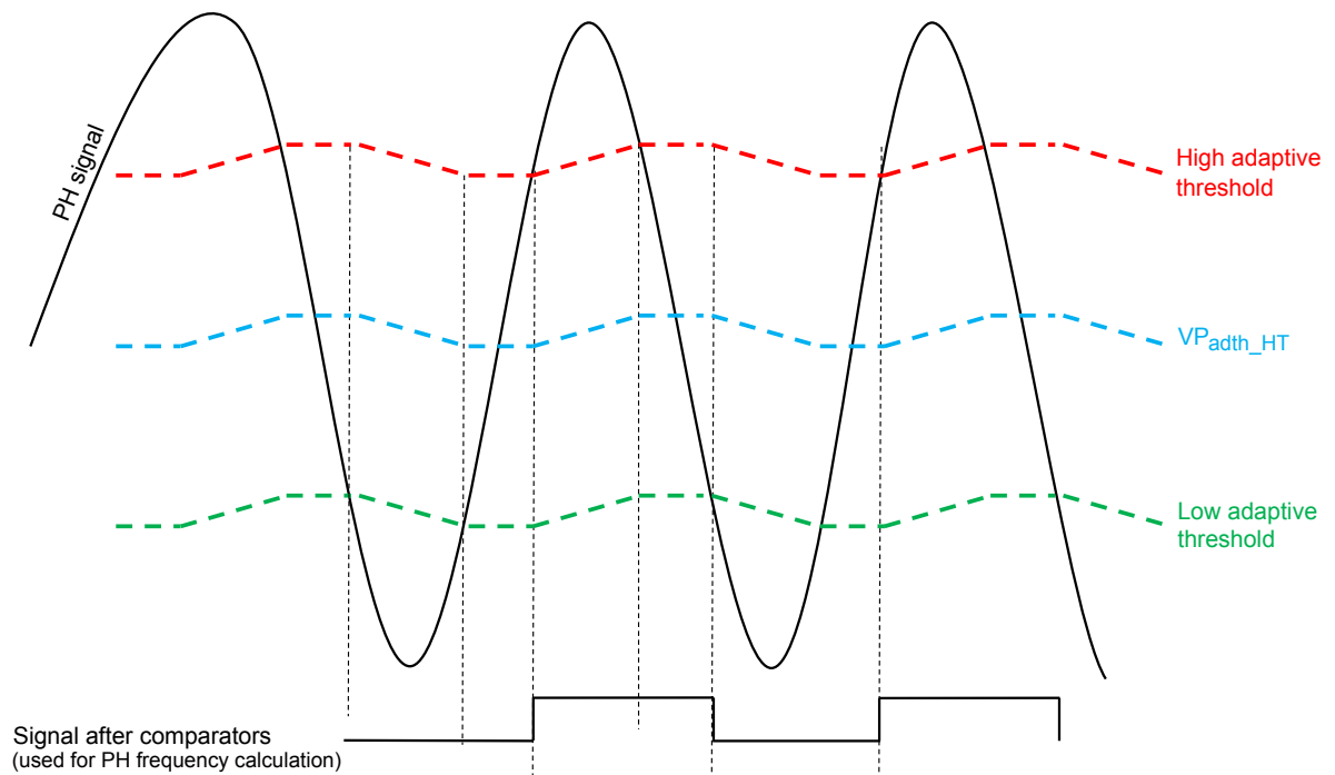
Figure 11. PH frequency calculation using adaptive PH thresholds calculation
