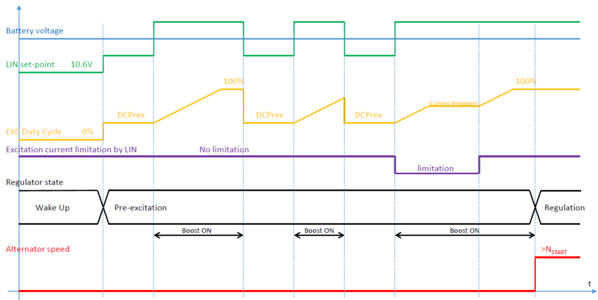
Figure 13. Pre-excitation specific mode: example 1
