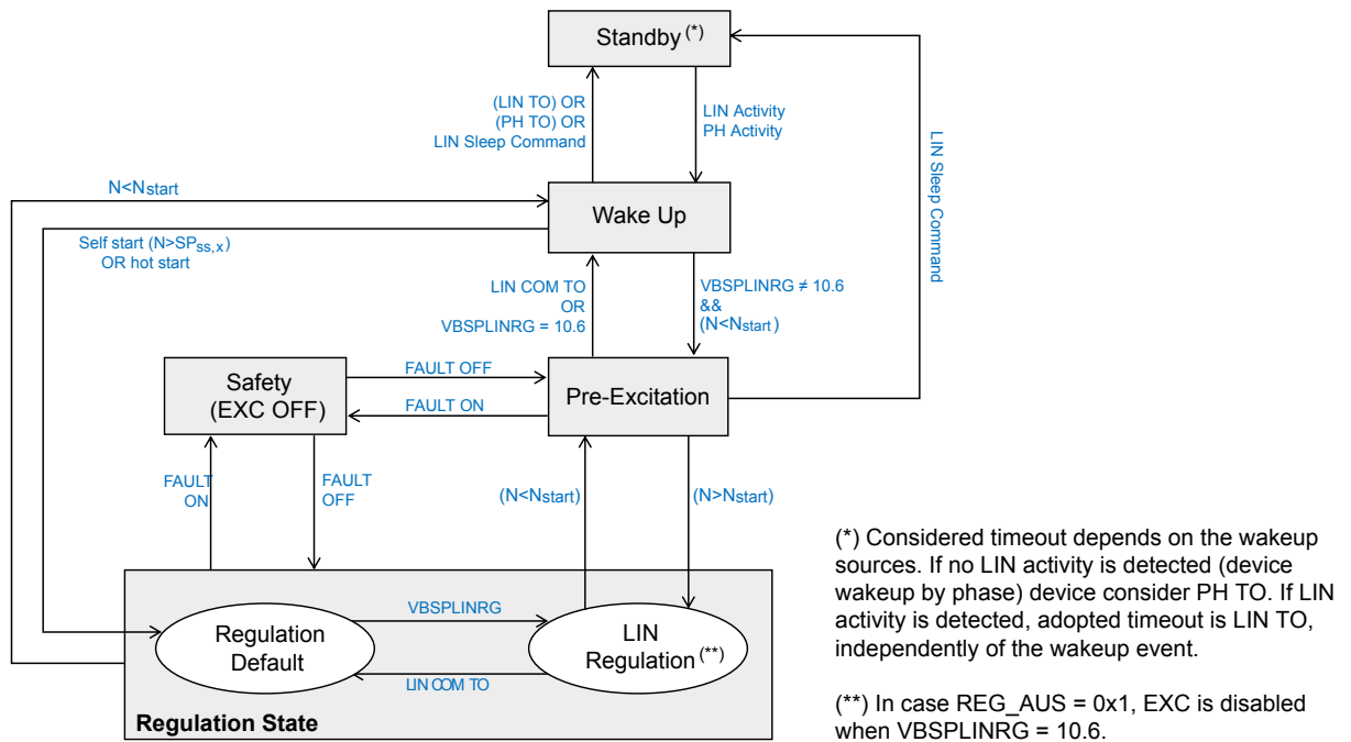
Figure 4. L9918B finite state machine diagram
