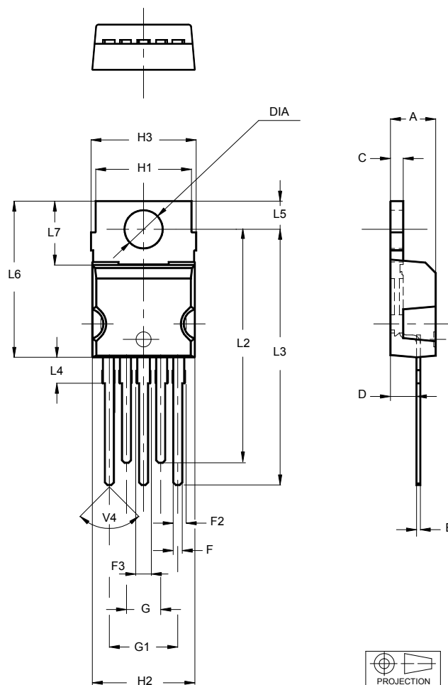
Figure 16. PENTAWATT In Line package outline
