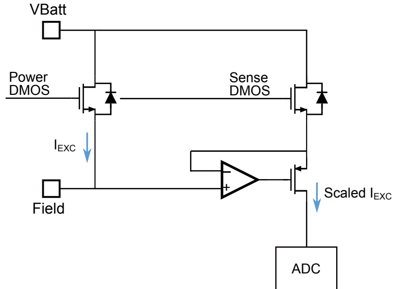
Figure 15. Excitation high side power MOS current measurement: working principle
