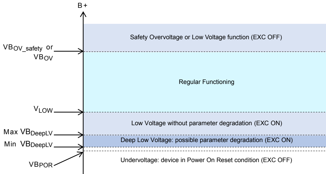
Figure 10. Battery voltage range
