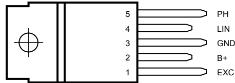
Figure 2. Pins connection diagram (top view)
