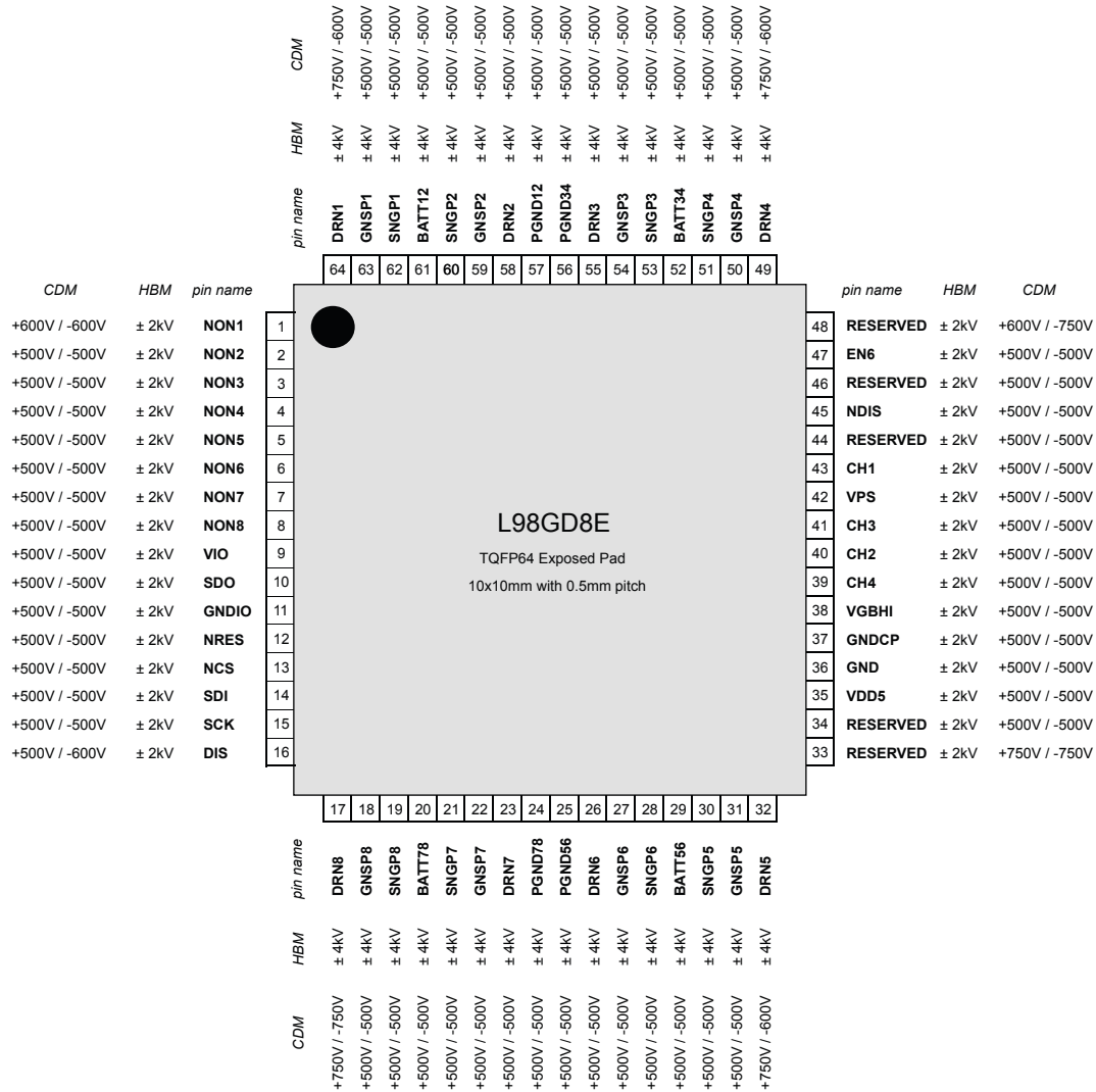
Figure 8. ESD ratings on pinout summarizes the ESD ratings for each pin according to both CDM and HBM models.
