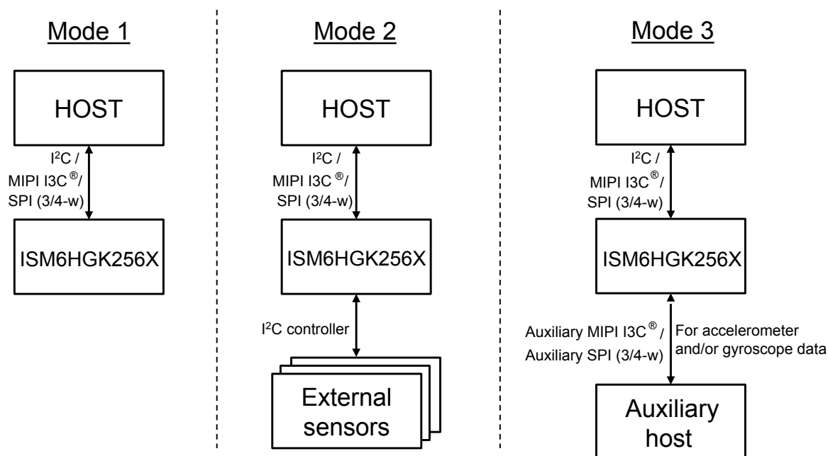
Figure 6. ISM6HGK256X connection modes
