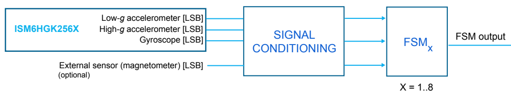
Figure 2. State machine in the ISM6HGK256X
