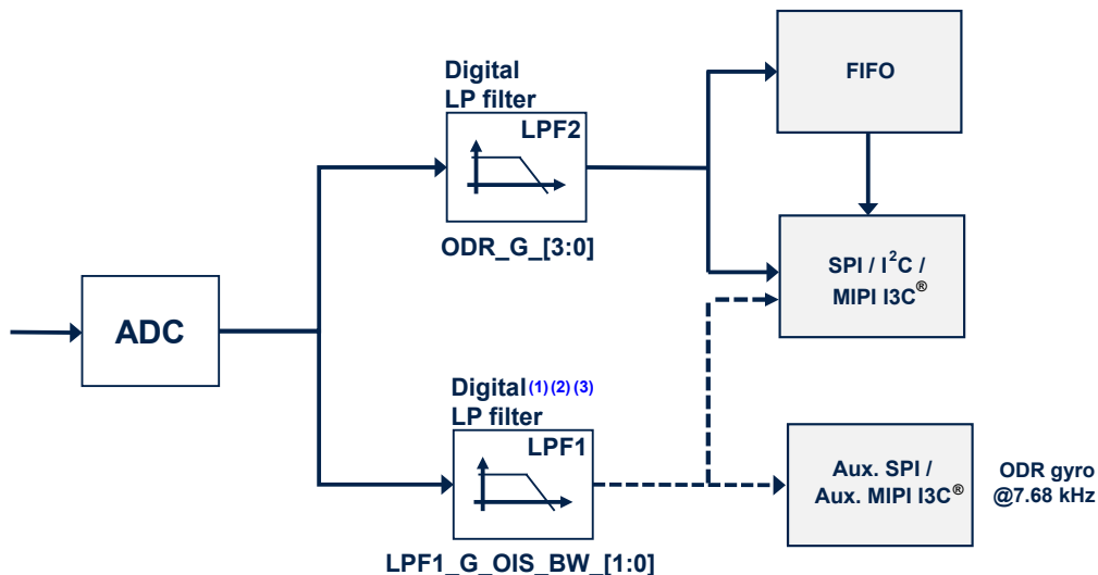
Figure 23. Gyroscope digital chain - mode 3 (OIS)
