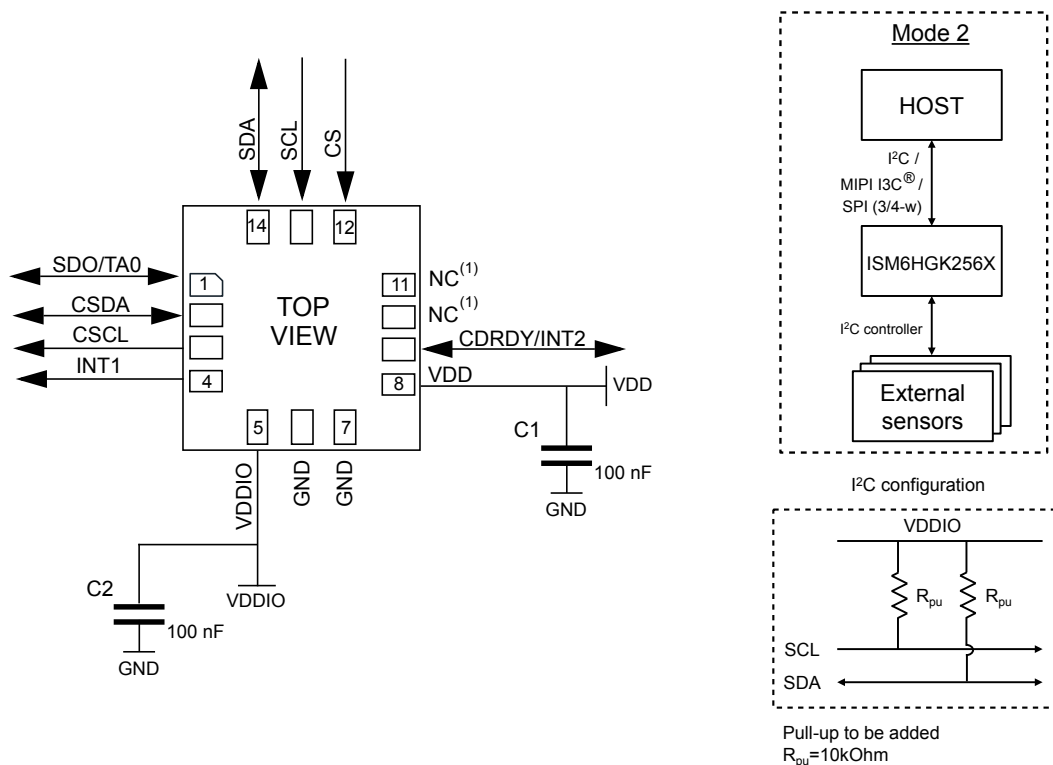
Figure 29. ISM6HGK256X electrical connections in mode 2
