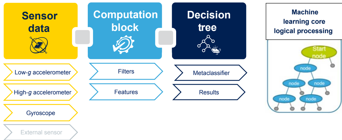
Figure 3. Machine learning core in the ISM6HGK256X
