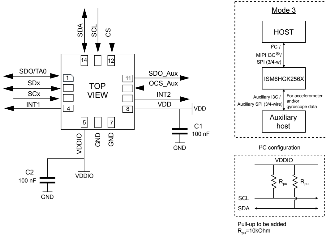
Figure 30. ISM6HGK256X electrical connections in mode 3 (auxiliary 3/4-wire SPI or auxiliary MIPI I3C)
