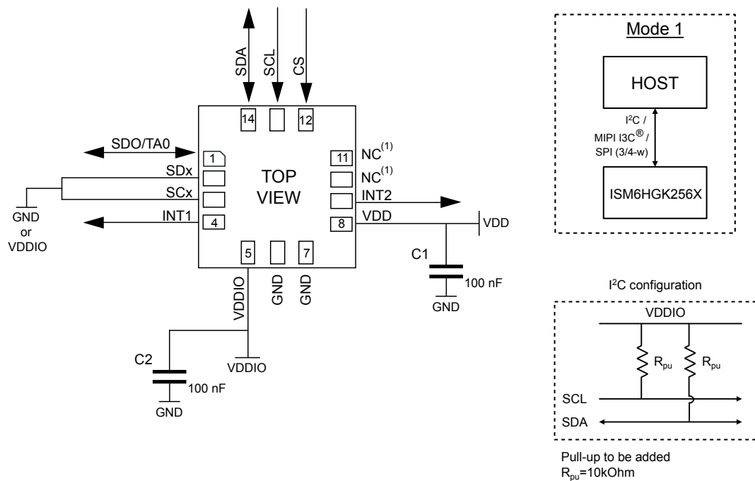
Figure 28. ISM6HGK256X electrical connections in mode 1
