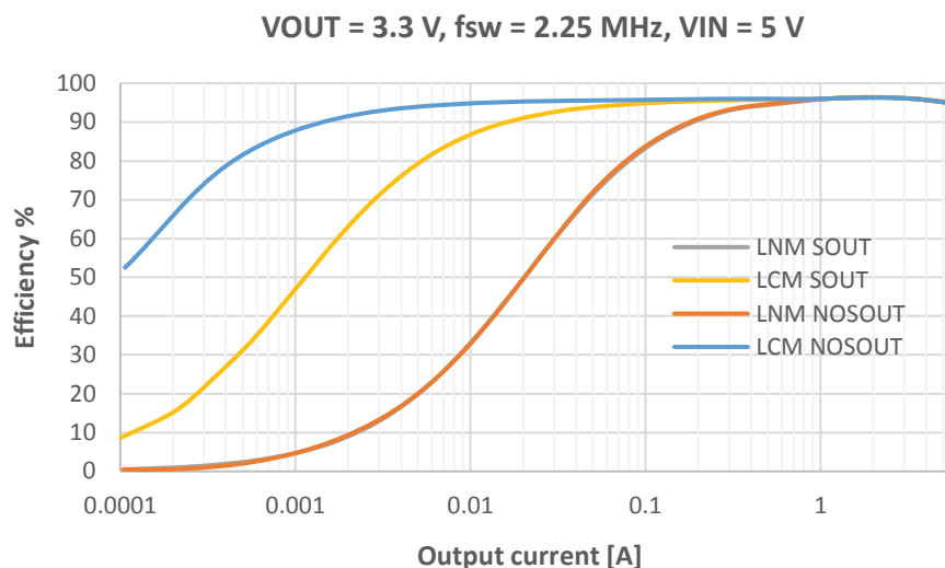
Figure 36. Efficiency (log. scale)
