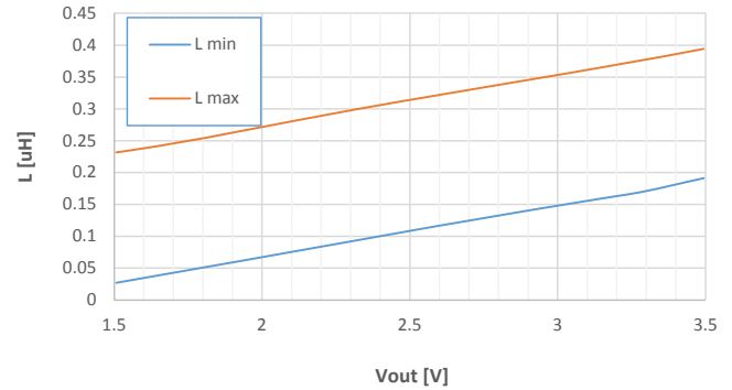
Figure 27. Lind vs. Vout - 3.5 MHz / Vin=5 V
