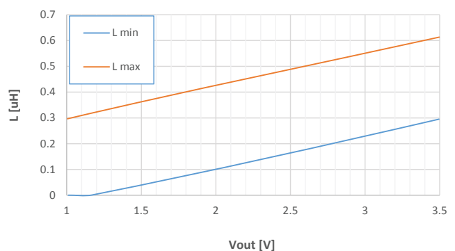
Figure 25. Lind vs. Vout - 2.25 MHz / Vin=5 V
