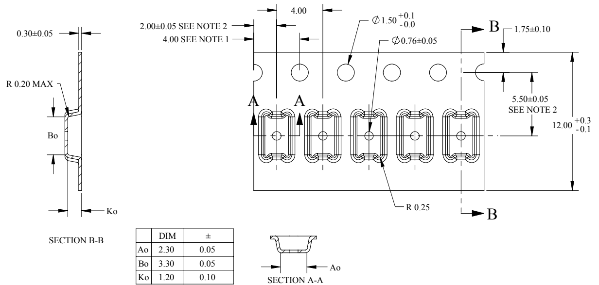
Figure 51. Carrier tape
