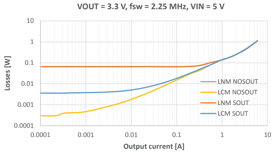
Figure 38. Total losses (log. scale)
