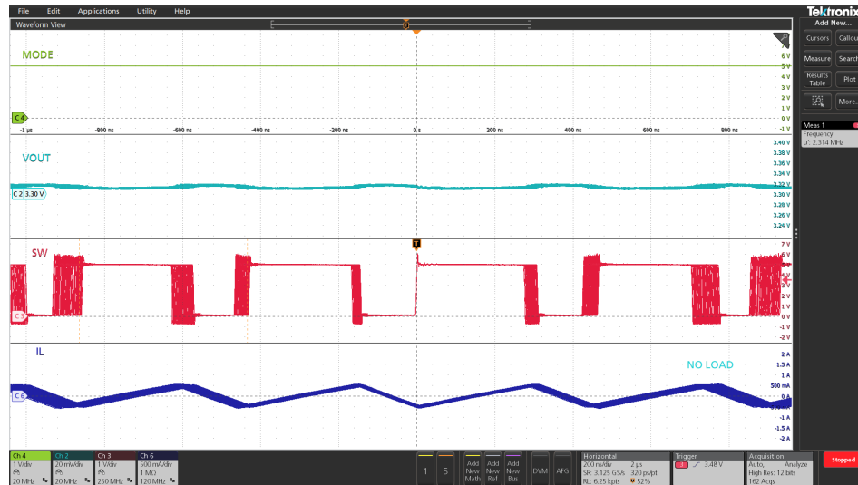
Figure 16. RFSET = 27 k, dithering enabled
