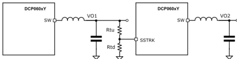
Figure 4. Schematic connection for tracking example
