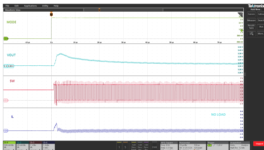
Figure 14. MODE toggle, LCM to LNM transition example
