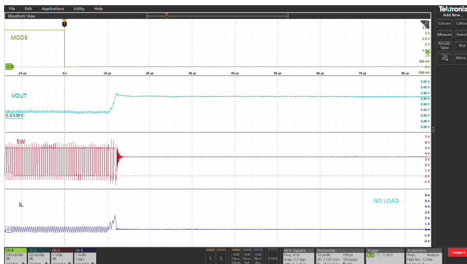
Figure 15. MODE toggle, LNM to LCM transition example
