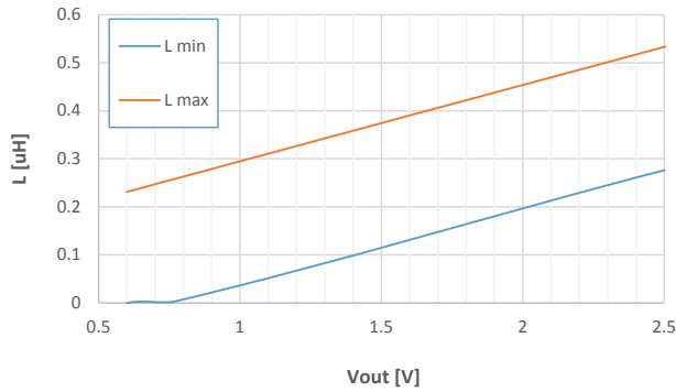
Figure 22. Lind vs. Vout - 1.8 MHz / Vin=3.3 V
