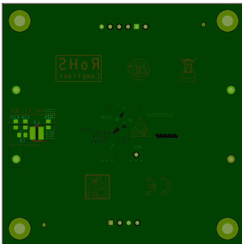
Figure 35. Evaluation board PCB layout. Bottom
