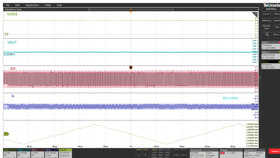
Figure 17. RFSET = 27 k, switching frequency time trend
