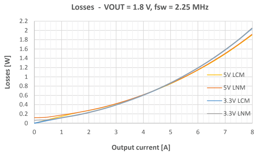
Figure 48. DCP0608Y Eval board total losses
