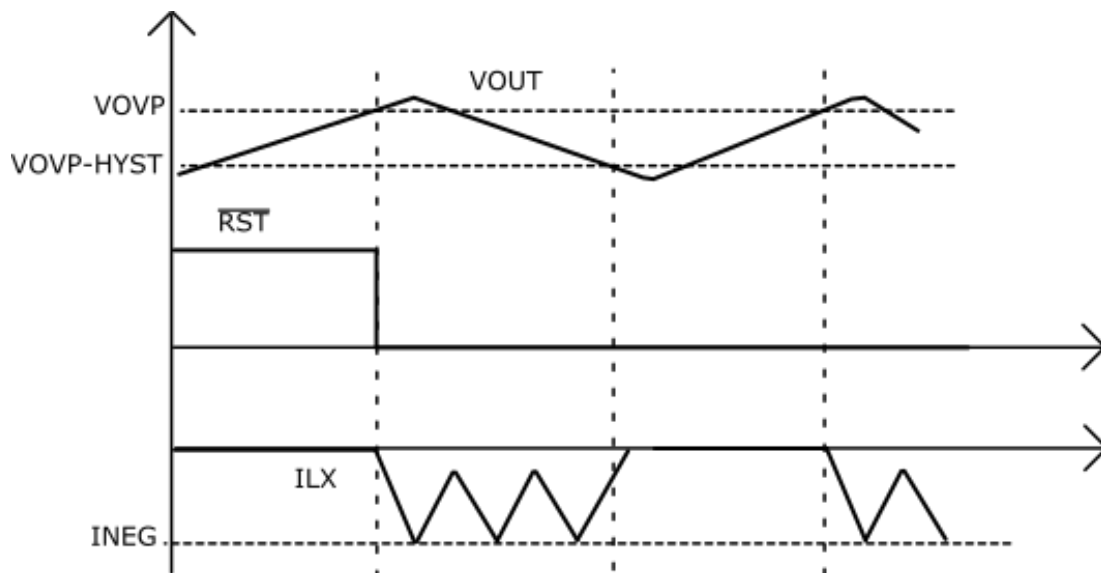
Figure 21. Output overvoltage protection
