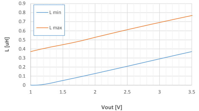
Figure 23. Lind vs. Vout - 1.8 MHz / Vin=5 V
