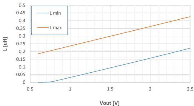
Figure 24. Lind vs. Vout - 2.25 MHz / Vin=3.3 V
