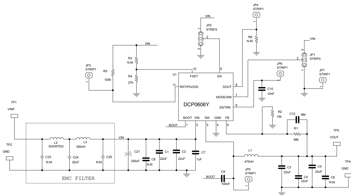
Figure 31. Evaluation board schematic
