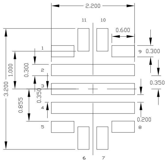
Figure 50. QFN11 (2 x 3 x 0.9 mm) recommended footprint - dimensions are in mm
