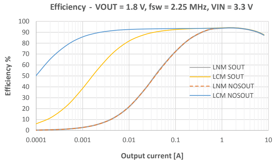
Figure 45. DCP0608Y Eval board efficiency (VIN = 3.3 V)
