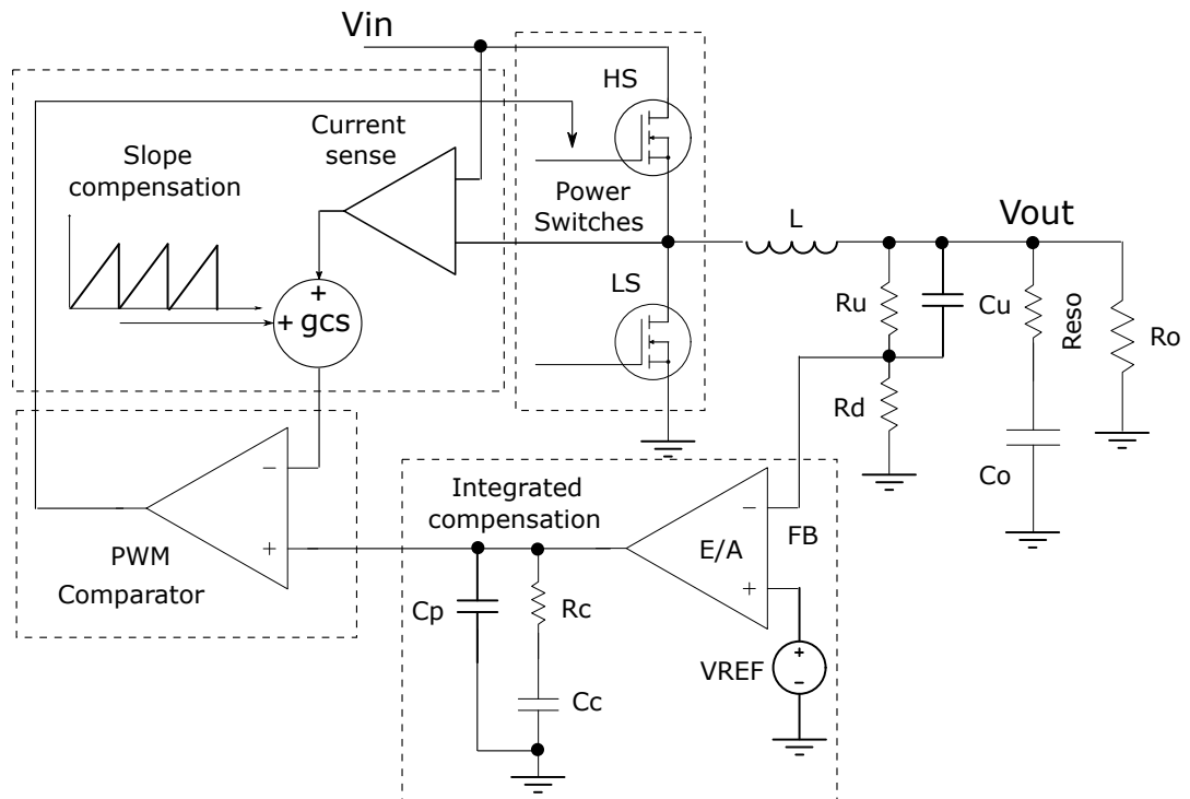
Figure 6. Control loop block diagram
