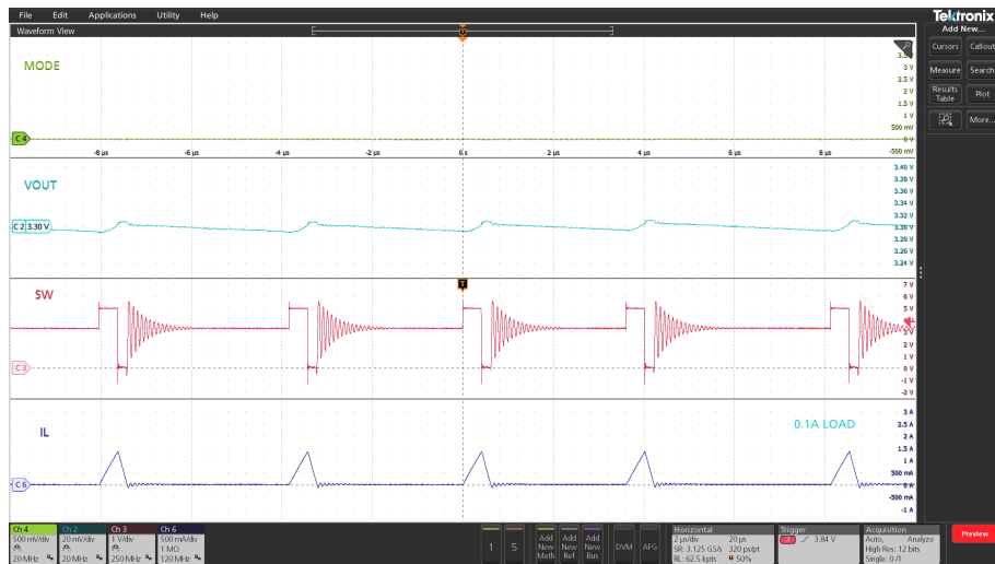
Figure 10. LCM operation, 100 mA load
