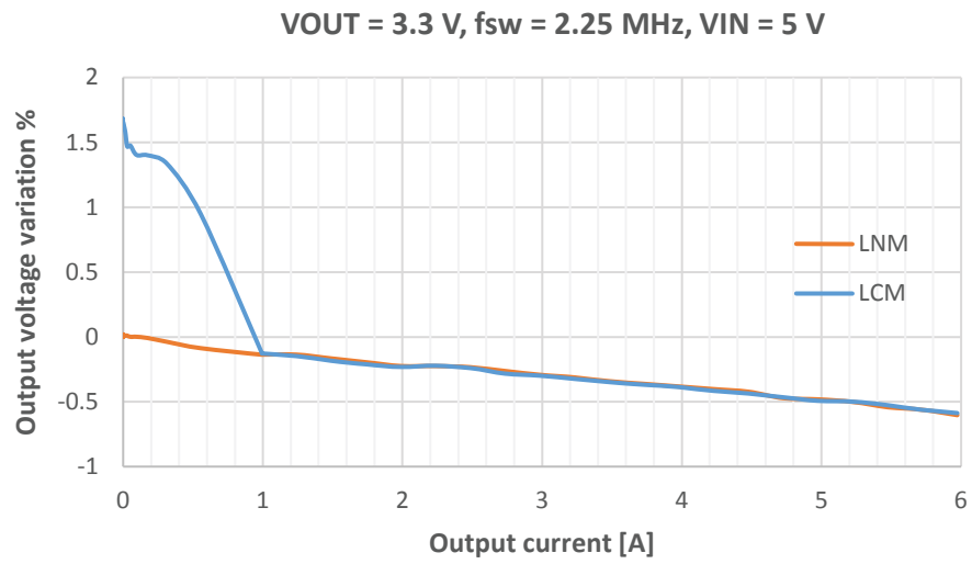
Figure 39. Load regulation
