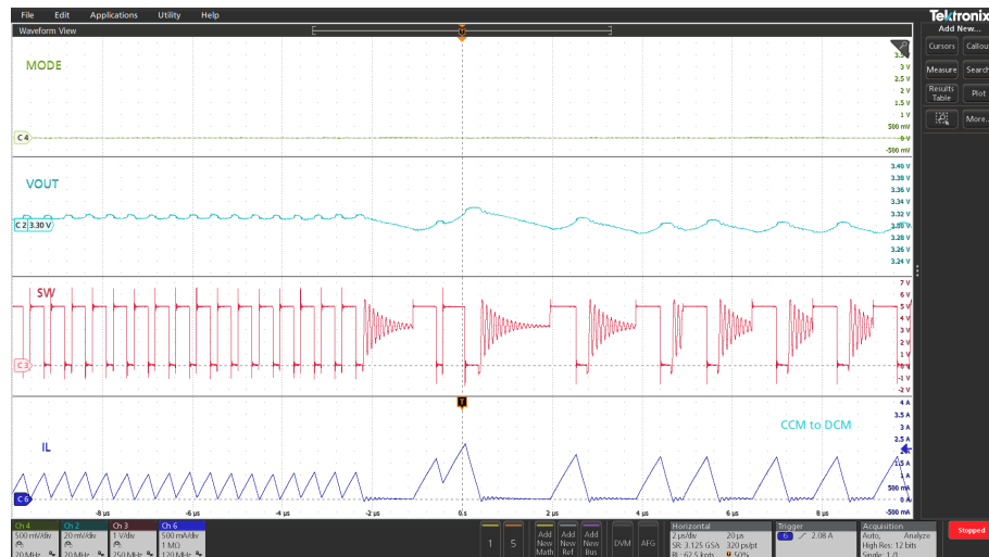
Figure 13. LCM operation, CCM to DCM transition
