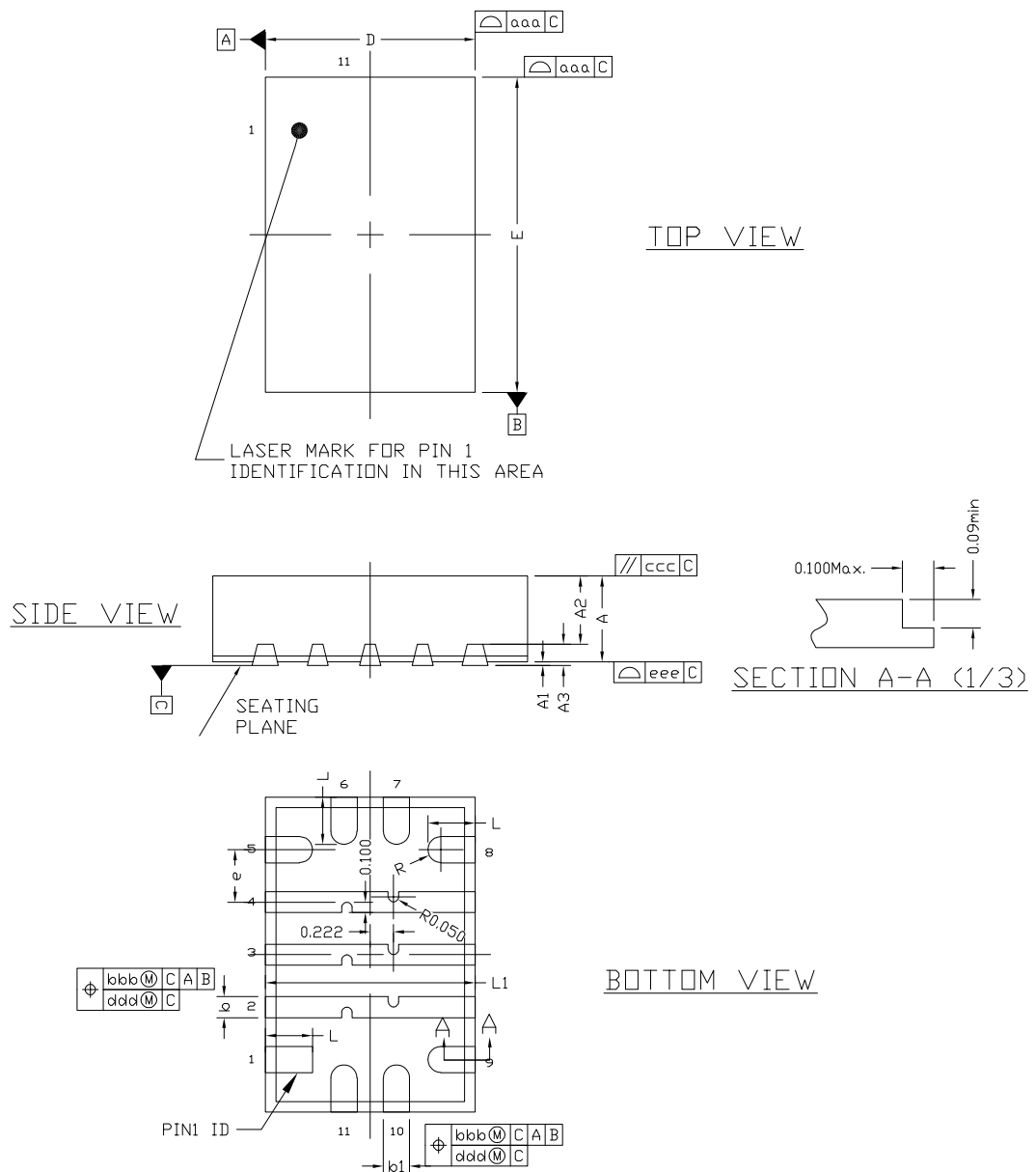
Figure 49. QFN11 (2 x 3 x 0.9 mm) package outline
