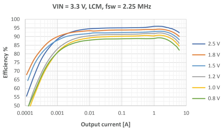
Figure 43. Efficiency vs. V_{OUT} – V_{IN} = 3.3\text{ V} - LCM ( S_{OUT} = GND )
