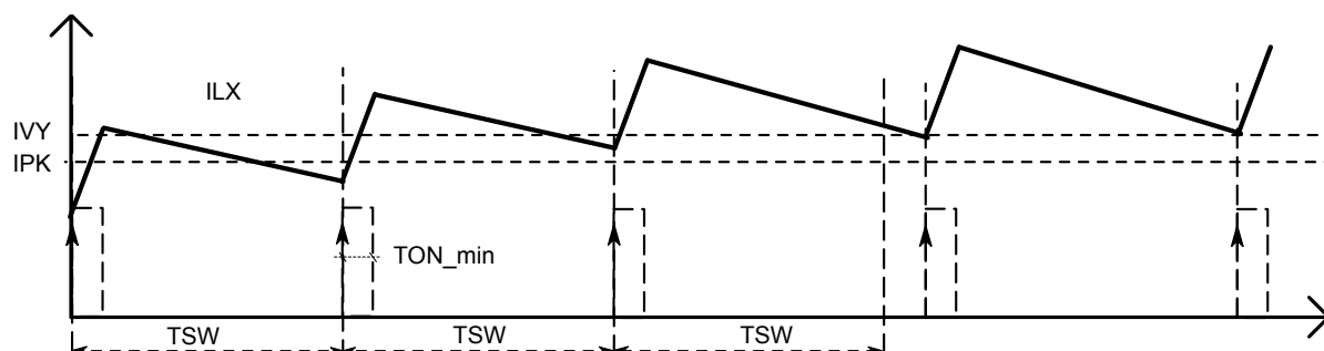
Figure 20. OCP – Valley current limit
