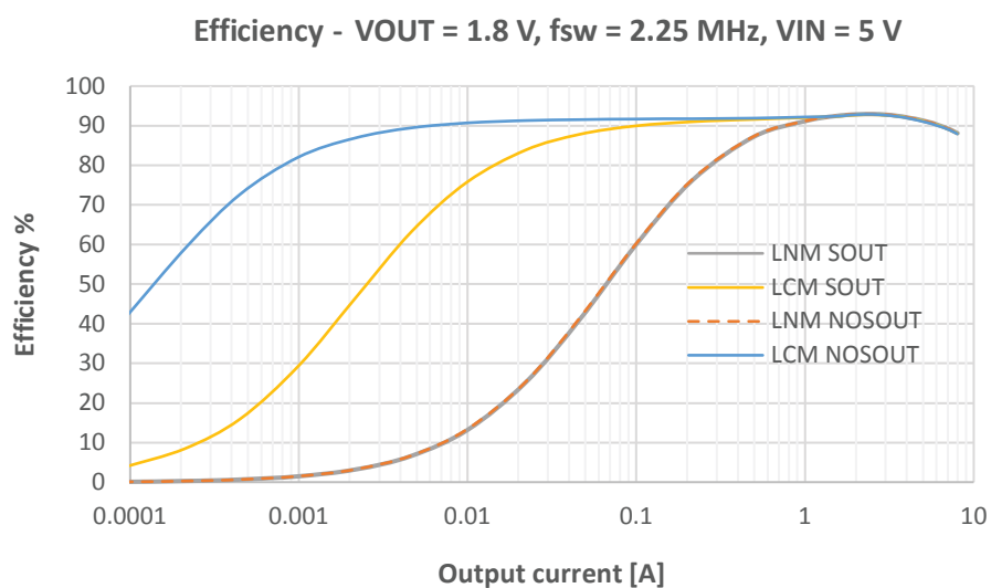
Figure 44. DCP0608Y eval board efficiency (VIN = 5 V)
