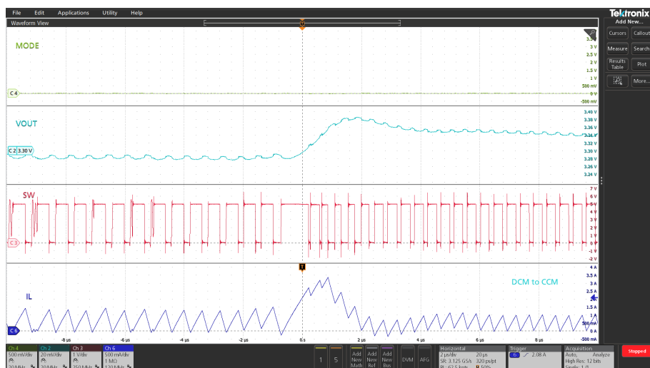
Figure 12. LCM operation, DCM to CCM transition
