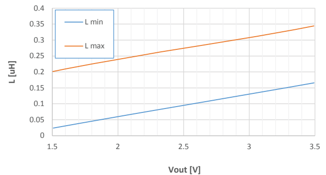
Figure 29. Lind vs. Vout - 4 MHz / Vin=5 V
