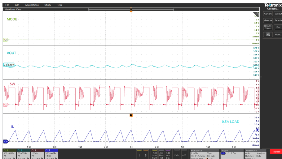
Figure 11. LCM operation, 500 mA load
