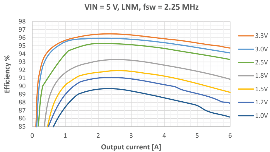
Figure 40. Efficiency vs. VOUT – VIN = 5 V - LNM
