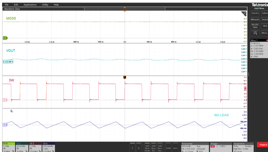
Figure 8. LNM operation, no load
