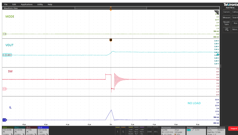
Figure 9. LCM operation, no load
