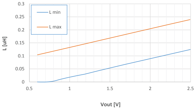
Figure 28. Lind vs. Vout - 4 MHz / Vin=3.3 V
