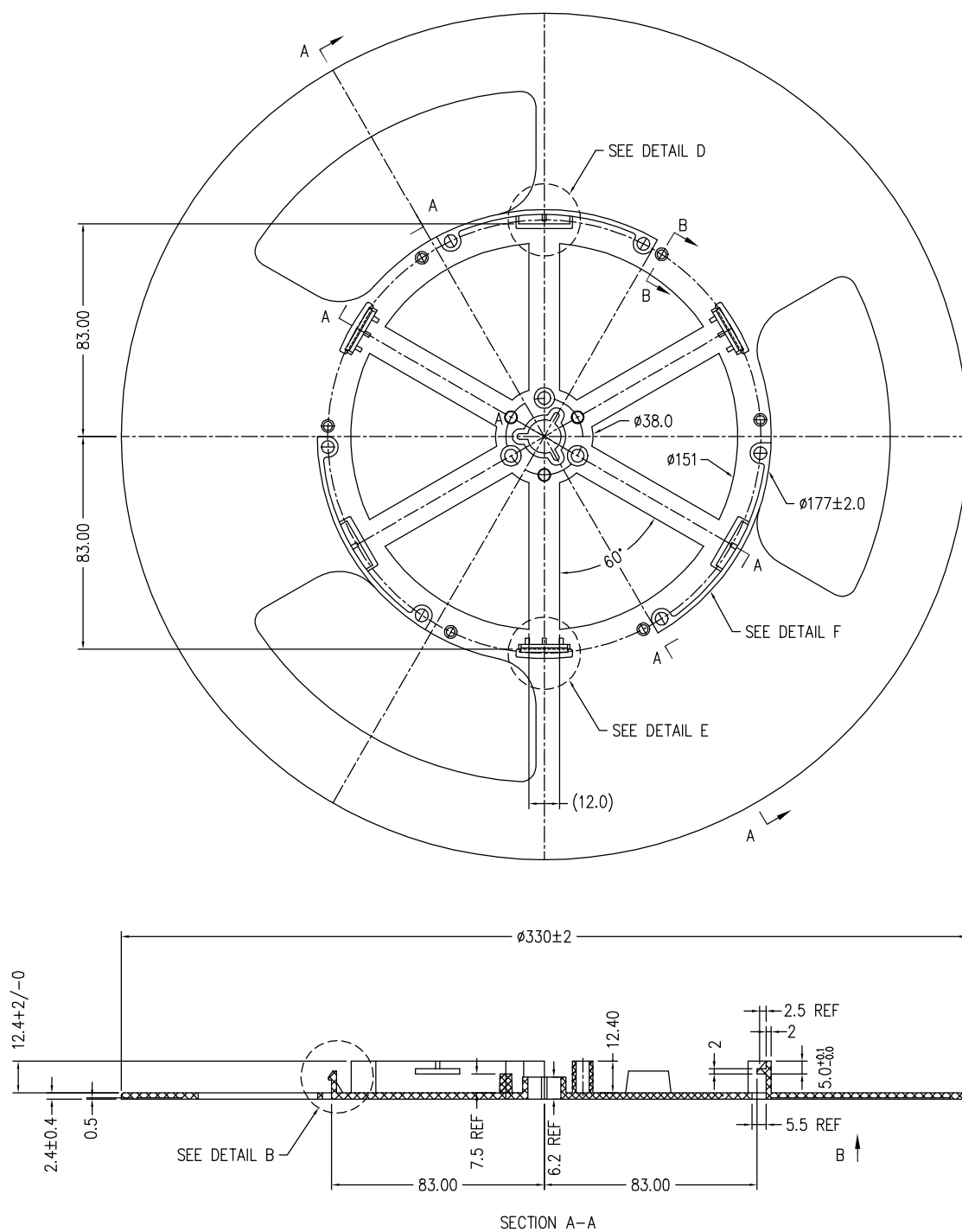
Figure 53. Carrier reel
