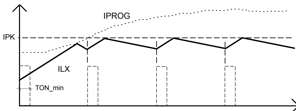
Figure 19. OCP - Peak current limit
