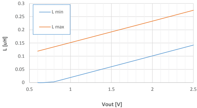
Figure 26. Lind vs. Vout - 3.5 MHz / Vin=3.3 V
