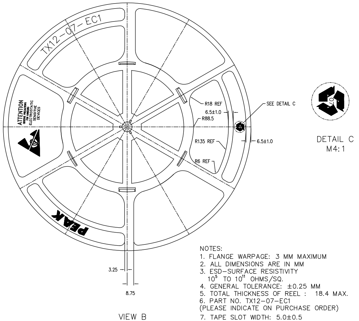
Figure 54. Reel drawing
