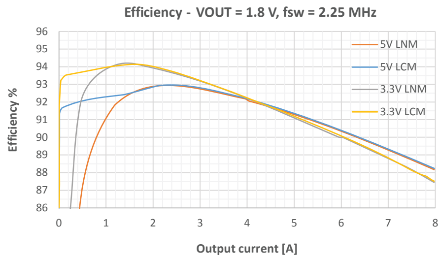
Figure 46. DCP0608Y Eval board efficiency (lin. scale)
