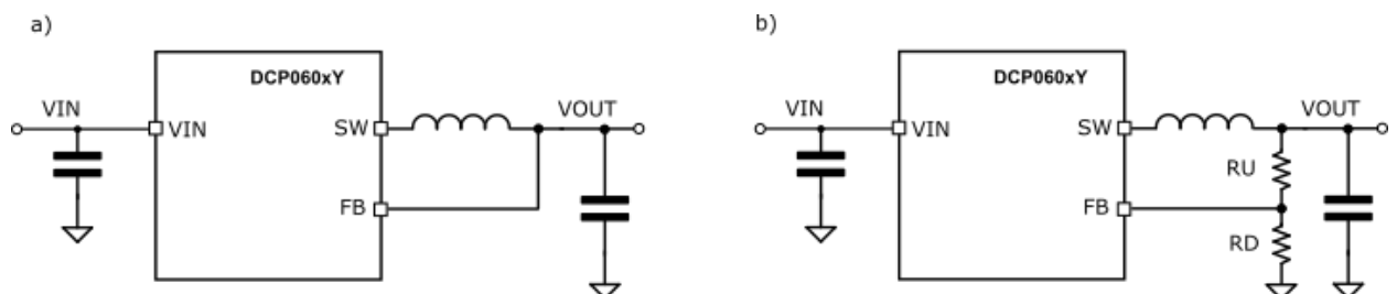
Figure 7. Output voltage programming. Fixed version (left) and adjustable version (right)
