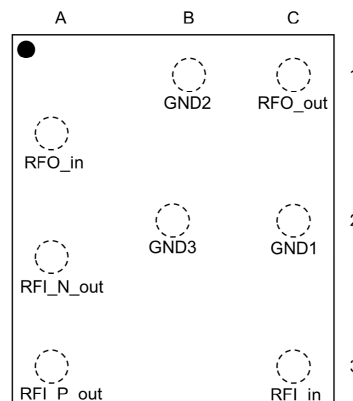
Figure 10. Top view
