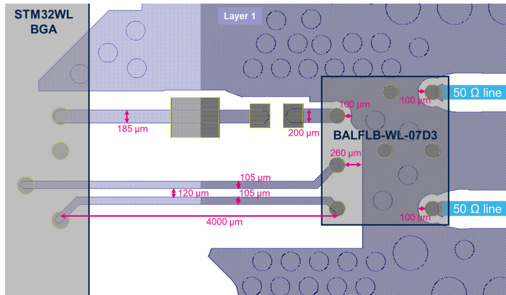
Figure 12. BGA-4L PCB land pattern recommendation
