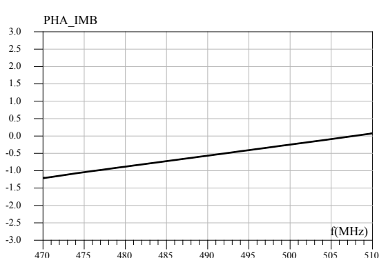
Figure 4. Phase imbalance (°)
